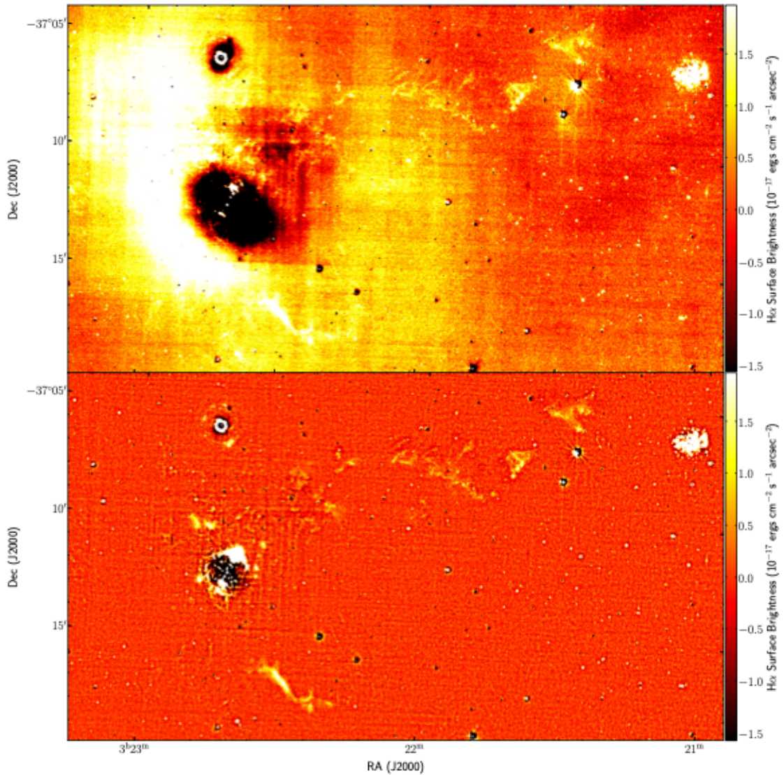
Fig. A.1. Comparison of the original and filtered H\alpha images. Top image: H\alpha image after the standard data reduction process. Bottom image: H\alpha image we present in our work that iteratively modelled and subtracted (described in Sect. 3.2) the background of the original image. Both images are presented on the same scale. The original image is clearly dominated by over- and under-subtracted artefacts, while the new image has a smooth and uniform background, which retains the majority of the real H\alpha emission. Some diffuse H\alpha emission is lost in this process, however, the new image is a significant improvement that shows the underlying structure of the giant H\alpha filaments in the IGM.
