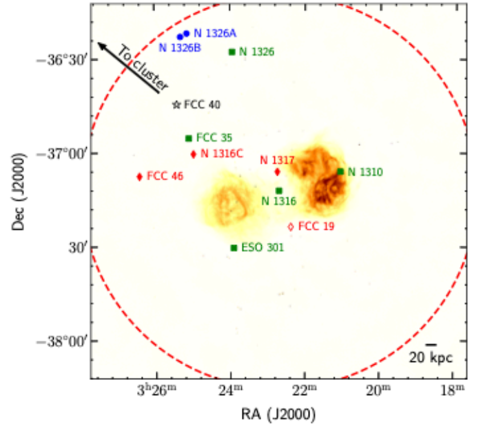
Fig. 8. Pre-processing map of the Fornax A group. The background image shows the 1.44 GHz MeerKAT radio continuum emission (Maccagni et al. 2020) and the position of each group galaxy are overlaid with the same markers as Fig. 7. The filled markers represent HI detections, the open markers indicate HI non-detections, where the early, ongoing, advanced, and unclassified pre-processing categories are shown as blue circles, green squares, red diamonds, and black stars, respectively. The red dashed circle denotes the 1.05^\circ ( 0.38 \text{ Mpc} ) virial radius of the group as adopted in Drinkwater et al. (2001). A 20 kpc scale bar is shown in the bottom right corner and the direction to the Fornax cluster is shown by the black arrow. There is no consistent trend between projected position and pre-processing status, although the majority of group galaxies show evidence of pre-processing. The extent of the NGC 1316 AGN lobes show that it may be playing a role in the pre-processing of neighbouring galaxies and the magnetic field could help the containment of multiphase gas.
