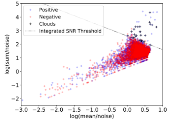
Fig. 1. Sum of the pixel values as a function of the mean pixel value for all sources detected with SoFiA. The blue points indicate the positive detections and the red points indicate the negative detections (Serra et al. 2012). Detected HI clouds are shown as black crosses. The dotted line shows the per-source integrated S/N of 4. Only positive sources above this threshold and with a reliability >0.65 are retained in our final catalogue. The chosen integrated S/N of 4 is a conservative threshold as it is closer to area of parameter space occupied by the most statistically significant detections (i.e. the positive sources with a high sum/noise for their mean/noise value) and is clearly above the edge of non-statistically significant detections (i.e. where the density of positive sources is approximately the same as the density of negative sources). Owing to this conservative threshold, the detected HI clouds, while often diffuse, occupy the parameter space of real, reliable HI emission.
