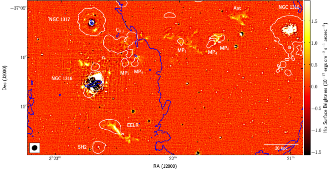
Fig. 6. OmegaCAM H\alpha emission showing the ionised gas in the vicinity of NGC 1316. The blue contour shows the majority of the western lobe of NGC 1316 in radio continuum at a (conservative) level of 1.3 \text{ mJy beam}^{-1} from Maccagni et al. (2020). The white contours show the 3\sigma H I column density of 1.4 \times 10^{19} \text{ atoms cm}^{-2} (over 44.1 \text{ km s}^{-1} ) from this work. Known sources (i.e. galaxies and IGM H I) and multiphase (MP) gas clouds that contain H\alpha and H I as well as the Ant-like feature from Fomalont et al. (1989) are labelled. This image reveals long filaments of ionised gas in the IGM.
