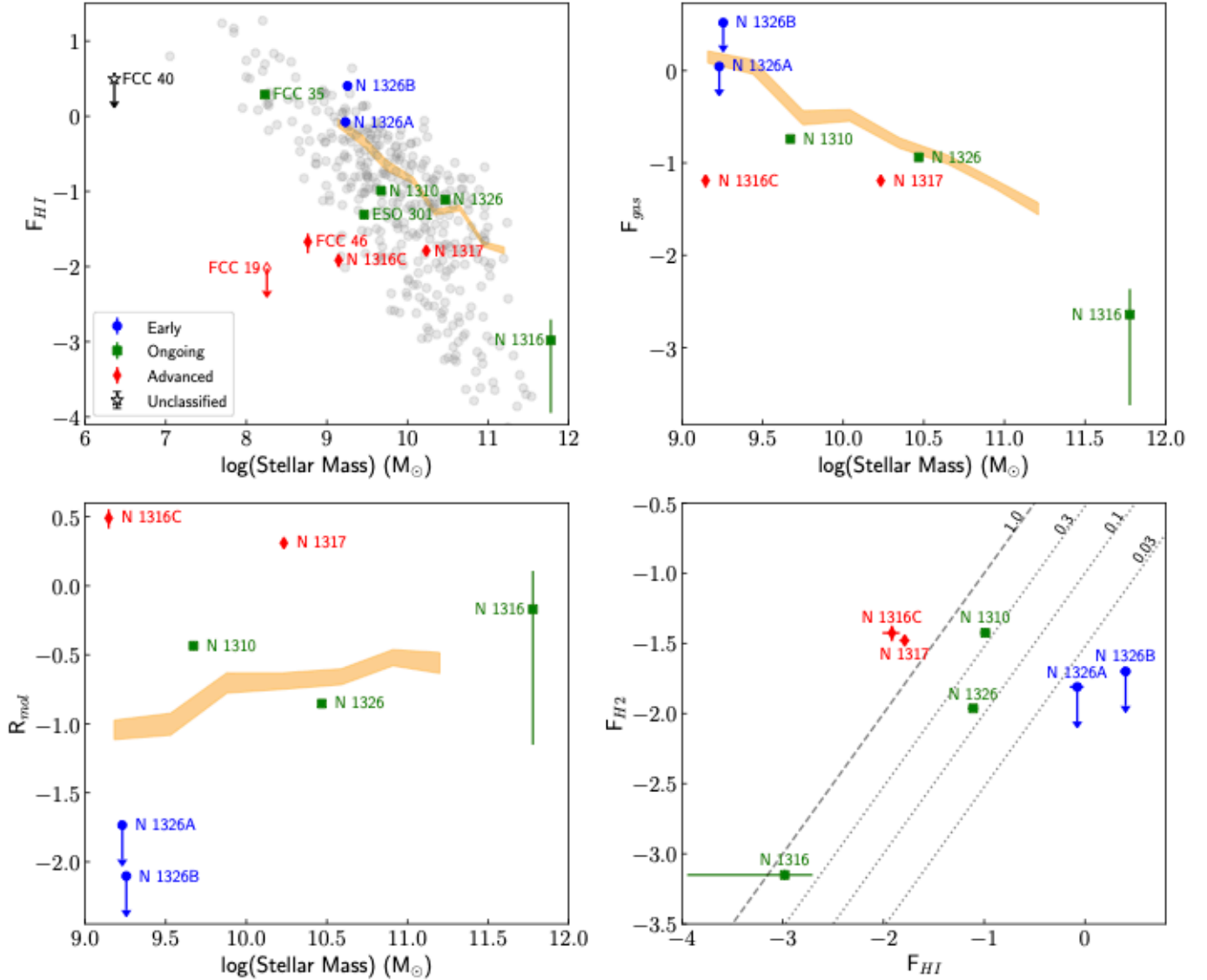
Fig. 7. Atomic and molecular gas scaling ratios. In all figures, the early, ongoing, and advanced pre-processing categories are shown as blue circles, green squares, and red diamonds, respectively and H_2 upper limits are depicted by arrows. Solid markers indicate H\text{I} detections and open markers are non-detections. FCC 40 is not assigned to any pre-processing category and is shown as the open black star. Top left panel: H\text{I} gas fraction compared to galaxies from the HRS (Boselli et al. 2010, 2014) and VGS (Kreckel et al. 2012) (grey points) that show the typical scatter in F_{H\text{I}} . The orange shaded region indicates the median trend from xGASS (Catinella et al. 2018). Top right panel: total gas fraction of our galaxies compared to the median xGASS-CO trend (Catinella et al. 2018) (orange shaded region). Bottom left panel: molecular-to-atomic-gas ratio of our galaxies compared to the median xGASS-CO trend (Catinella et al. 2018) (orange shaded region). Bottom right panel: H_2 gas fraction as a function of H\text{I} gas fraction, showing constant ratios of 100%, 30%, 10%, and 3%. Overall, the galaxies in the early category are H\text{I} rich, the galaxies in the ongoing category typically follow the xGASS and xGASS-CO median scaling relations (Catinella et al. 2018), while galaxies in the advanced category have no H\text{I} or are H\text{I} -deficient with irregularly high H_2 -to- H\text{I} ratios.
