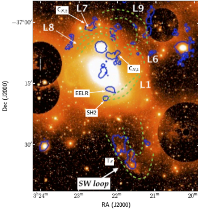
Fig. 5. Low surface brightness (star removed) image of NGC 1316 in g -band, observed with the VST (Iodice et al. 2017). The known (Schweizer 1980; Richtler et al. 2014; Iodice et al. 2017) stellar loops are labelled and outlined by the dashed green lines. The H I is shown by the solid blue contours and the previously known H I clouds are labelled. The clouds that make up T_S (including the new western H I cloud) overlap with the stellar SW loop. There is some overlap with some H I clouds in the north (e.g., C_{N,2} and the clouds to the west) and the optical loop L7. Overall, there is no consistent correlation between the stellar loops and the distribution of H I clouds.
