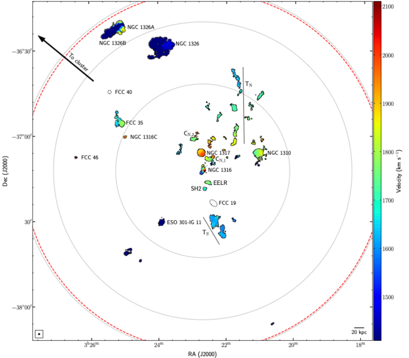
Fig. 4. HI velocity field, where the known galaxies and previously detected clouds and tails in the IGM are labelled. As in Fig. 2, the two galaxies not detected in HI are outlined by black, dashed ellipses and the direction to the Fornax cluster is shown by the black arrow. The velocity colour bar is centred on the systemic velocity of the BGG (NGC 1316) at 1760 \text{ km s}^{-1} . The grey circles indicate the sensitivity of the primary beam (Mauch et al. 2020) at 50%, 10%, and 2%. The red dashed circle denotes the 1.05^\circ ( 0.38 \text{ Mpc} ) virial radius of the group as adopted in Drinkwater et al. (2001), where the restoring ( 33.0'' \times 29.2'' ) beam and scale bar are shown in the bottom corners. The clouds that make up T_N have a new, extended component, effectively doubling the size compared to its original discovery in Serra et al. (2019).
