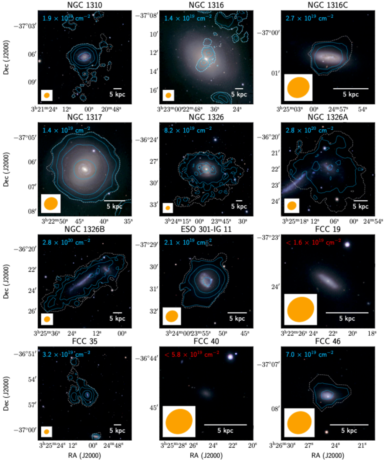
Fig. 3. Optical three-colour composite of each group galaxy in our sample with overlaid HI contours. The colour image is comprised of the g -, r -, and i -band filters from the FDS (Iodice et al. 2016); the white dashed contour shows the most sensitive, constant column density of N_{\text{HI}} = 1.4 \times 10^{19} \text{ atoms cm}^{-2} from Fig. 2 and the blue contours start from the local column density sensitivity (i.e. 1.4 \times 10^{19} \text{ atoms cm}^{-2} scaled by the primary beam response; see top left corner of each cutout) and increase by a factor of 3^n with n = 0, 1, 2, \dots , at each step. For non-detections, the 3\sigma HI column density upper limit over a single channel is shown in red in the top left of the cutout. The restoring beam ( 33.0'' \times 29.2'' ) is shown in orange in the bottom left corner and a 5 kpc scale bar is shown in the bottom right corner.
