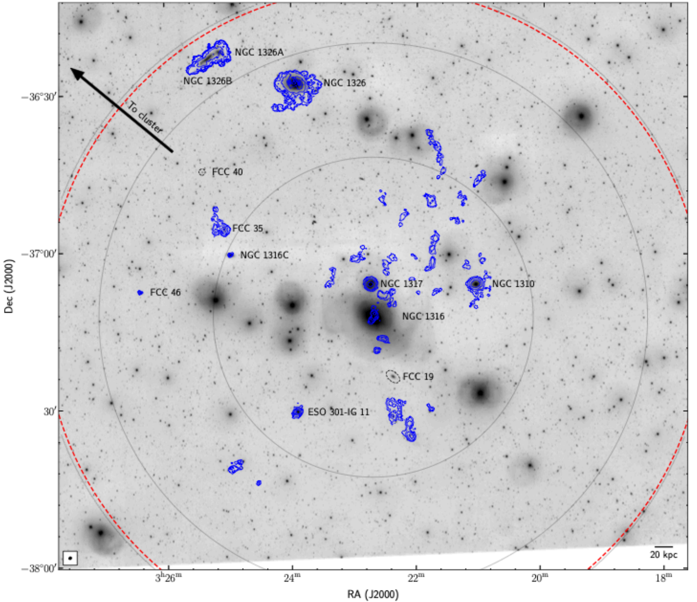
Fig. 2. Primary beam-corrected constant H I contours from MeerKAT (blue) overlaid on a FDS (Iodice et al. 2016) gri stacked optical image. The lowest contour represents the 3\sigma column density level of N_{\text{HI}} = 1.4 \times 10^{19} \text{ atoms cm}^{-2} over a 44.1 \text{ km s}^{-1} channel, where the contours increase by a factor of 3^n ( n = 0, 1, 2, \dots ). The group galaxies are labelled and the galaxies not detected in H I are outlined by a dashed black ellipse. The grey circles indicate the sensitivity of the primary beam (Mauch et al. 2020) at 50%, 10%, and 2%. The red dashed circle denotes the 1.05^\circ (0.38 Mpc) virial radius of the group as adopted in Drinkwater et al. (2001), where the restoring beam ( 33.0'' \times 29.2'' ) is shown in the bottom left corner and a scale bar indicating 20 kpc at the distance of Fornax A in the bottom right corner. The direction to the Fornax cluster is shown by the black arrow. In H I, we detect 10 (out of 12) galaxies, previously known clouds and streams in the IGM and a population of new H I clouds in the IGM. The previously known IGM H I structures are labelled in Fig. 4 for clarity.
