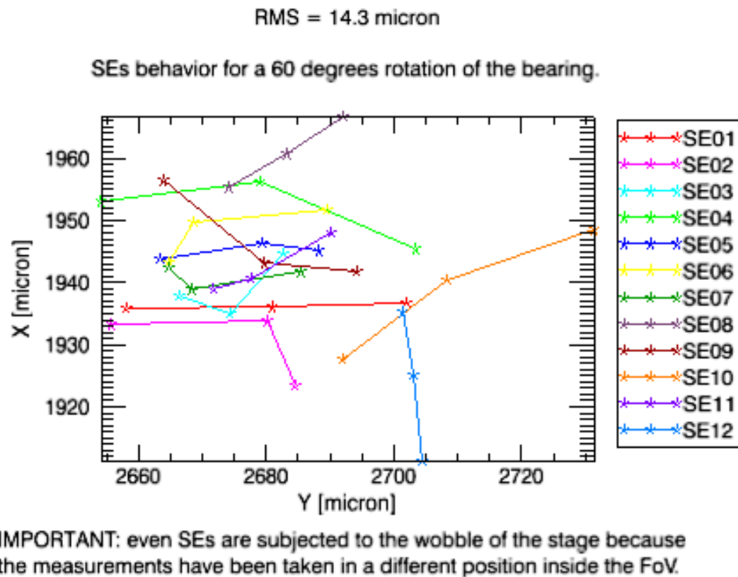
Fig. 4 all the SEs together in the field. The RMS relative shift is 14.3 microns, but it's clear that the spots produced by the even-labeled SEs are slightly shifted with respect to the median position of the spots, since the SEs are not exactly in the positions in which they have been aligned.
