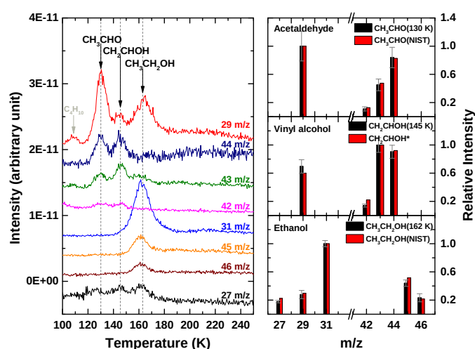
Fig. 3. Left: TPD mass spectra obtained after 60 min of codeposition of C 2 H 2 + O 2 + H (exp. 3) at 10 K. The applied deposition ratio of C 2 H 2 :O 2 :H was 1:10:40, and the used H-atom flux was 1.2 \times 10^{13} atoms cm -2 s -1 . Only relevant m/z channels are shown and shifted for clarity. The arrows and dashed lines indicate the peak position of the corresponding COMs. Right: comparison of the ionization fragmentation pattern of the detected COMs (black) with available values in the literature (red; NIST database: acetaldehyde and ethanol; Tureček & Hanuš 1984; vinyl alcohol).
