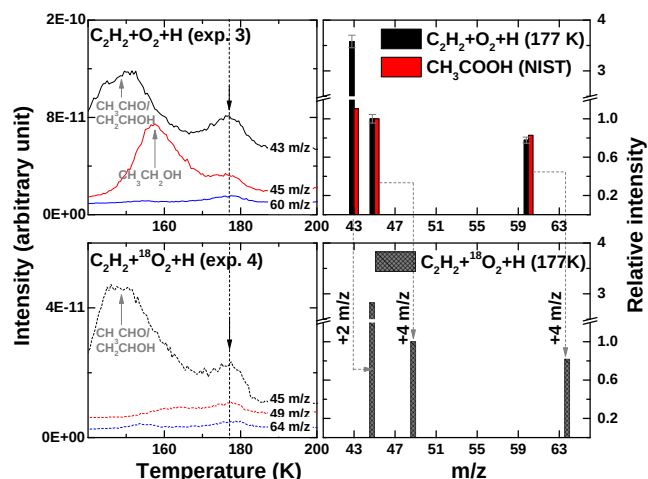
Fig. 4. Left: TPD mass spectra obtained after 360 min of codeposition of C 2 H 2 + O 2 + H (exp. 3) and C 2 H 2 + 18 O 2 + H (exp. 4) at 10 K. The applied deposition ratio of C 2 H 2 :( 18 O) 2 :H was 1:10:40, and the used H-atom flux was 1.2 \times 10^{13} atoms cm -2 s -1 . Only relevant m/z channels are shown and shifted for clarity. The dashed line indicates the peak position of the corresponding COMs. Right: comparison of the ionization fragmentation pattern for the QMS peak at 177 K (black) with data of CH 3 COOH in NIST (red). The position of the dashed arrows present for the isotope mass signal shifts in exp. 4.
