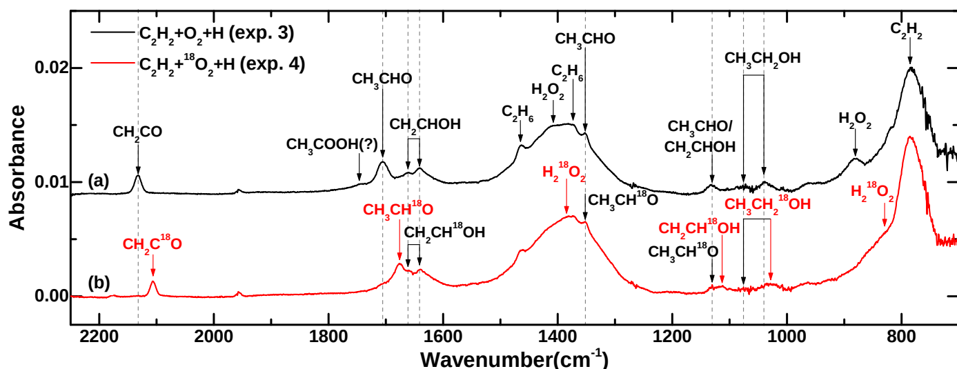
Fig. 2. IR spectra obtained after the codepositions of (a) C 2 H 2 + O 2 + H (exp. 3), and (b) C 2 H 2 + 18 O 2 + H (exp. 4) for 360 min at 10 K. The applied deposition ratio of C 2 H 2 : 18 O 2 :H was 1:10:40, and the used H-atom flux was 1.2 \times 10^{13} atoms cm -2 s -1 . The dashed lines are shown for the peak positions of regular molecules. IR spectra are offset for clarity.
