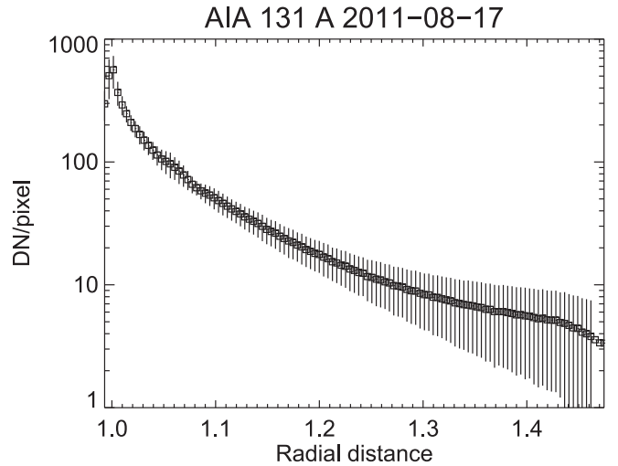
Figure 12. Observed radial fall-off in the AIA 131 Å band.
