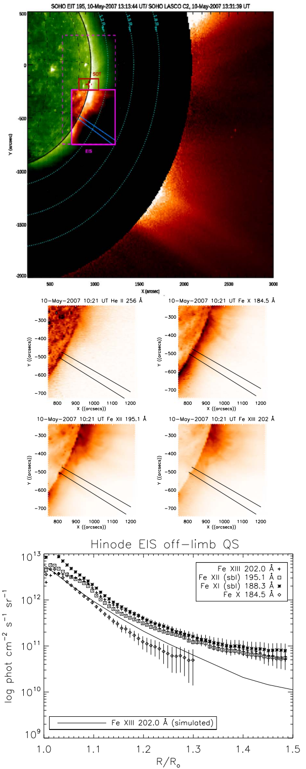
Figure 9. From top to bottom: (1) a SOHO EIT 195 Å image on 2007 May 10, with the Hinode EIS field of view (full possible, pink dashed rectangle; observed, full pink lines) and the EIS Fe XII 195.1 Å monochromatic image. The blue lines indicate the radial sector used for the averaging (see text). The SOHO LASCO C2 image is superimposed, showing that the selected radial sector is in a streamer. (2) Monochromatic images (negative) in a few spectral lines, with the radial sector indicated. (3) the observed radial variation of the radiance of the main coronal lines. The full line is the estimated radiance in the Fe XIII 202.0 Å line, based on the modeling of the 1996 solar minimum quiet Sun streamer.
