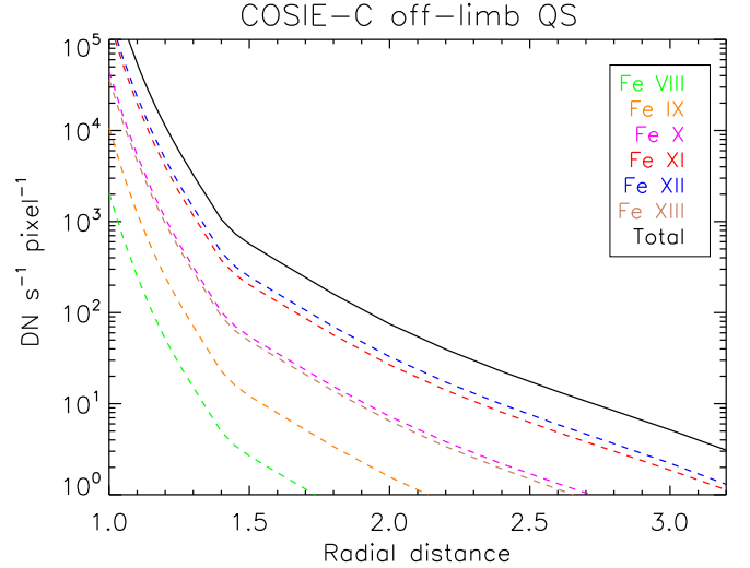
Figure 7. Estimated total count rates (per pixel) in the COSIE-C broadband, as a function of the radial distance, for the quiet Sun, using the UVCS model. The total rates are shown, as well as those produced by the main ions.
