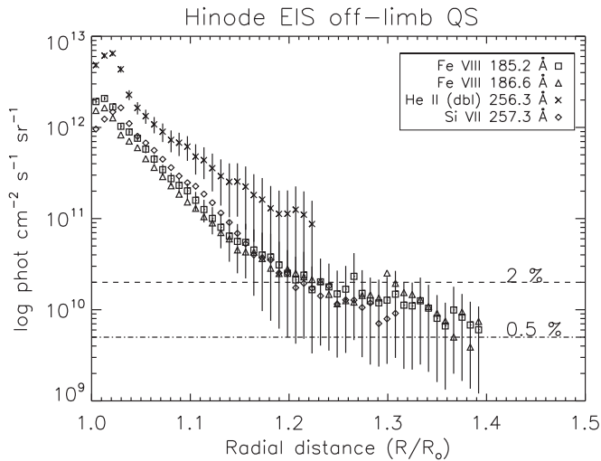
Figure 13. Observed radial fall-off in the cooler EIS lines (cf. bottom of Figure 9). The two dashed lines indicate 2% and 0.5% levels from the on-disk values.
