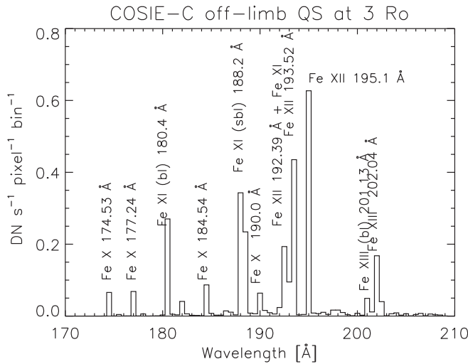
Figure 8. COSIE-C predicted spectrum at 3 R_{\odot} .
