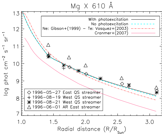
Figure 3. Radiance of the Mg X 610 Å line as a function of the radial distance, for three quiet Sun (QS) observations and one active region (AR). The lines are the predicted radiances.
