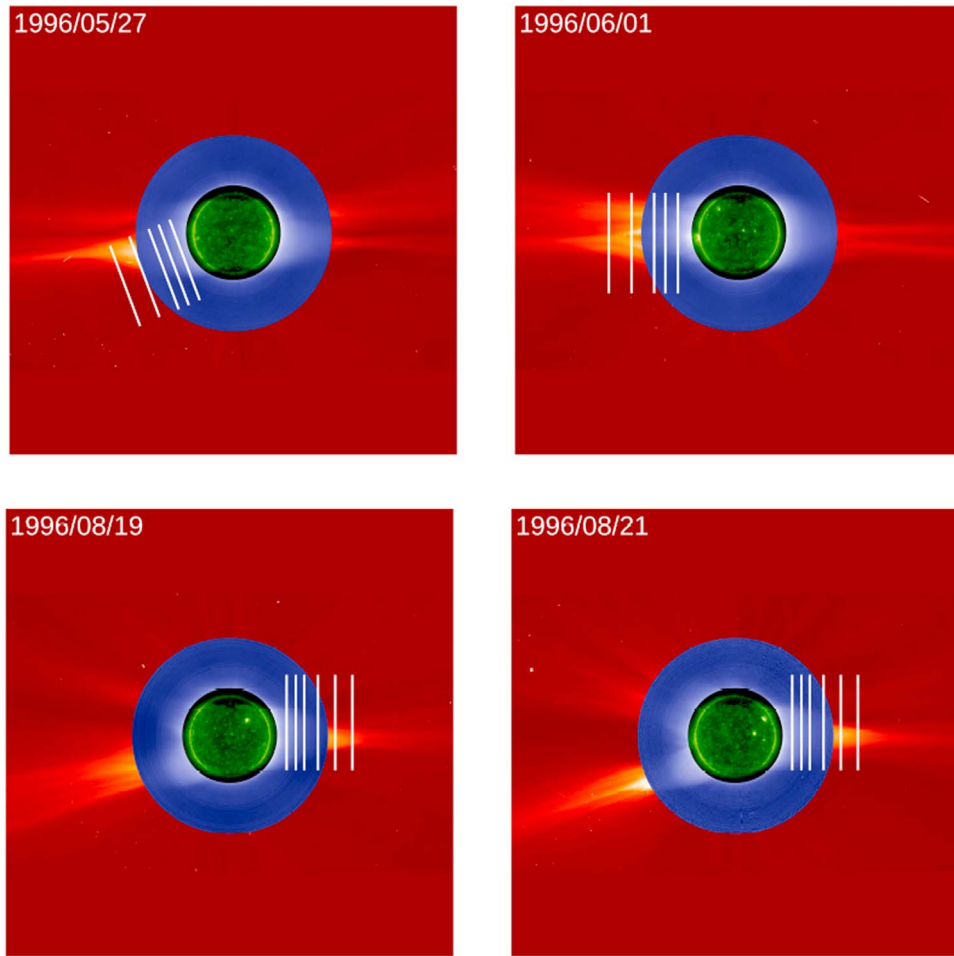
Figure 2. Composite images including SoHO EIT 195 Å, HAO Mauna Loa Mark 3, and LASCO/C2 white-light coronagraphs during times when the quiescent streamers discussed here were observed by SoHO UVCS, on 1996 May 27 (top left) and 1996 August 19 and 21 (bottom). The top right plot shows an active region streamer observed on 1996 June 1. The location of the UVCS slit is shown.
