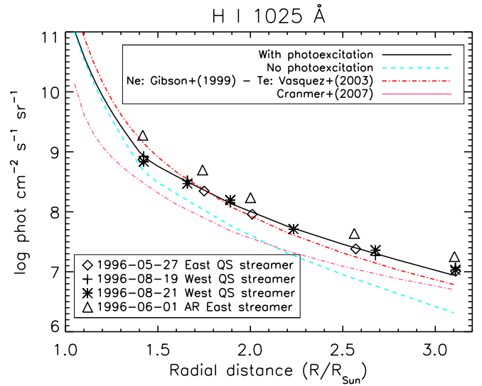
Figure 5. Radiance of the H I 1025 Å line as a function of the radial distance for three quiet Sun (QS) observations and one active region (AR). The lines are the predicted radiances.
