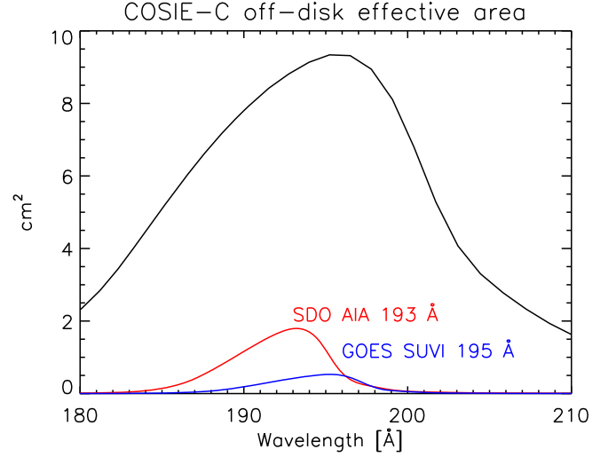
Figure 6. Estimated COSIE-C effective area, compared to those of the SDO AIA 193 Å and GOES SUVI 195 Å.
