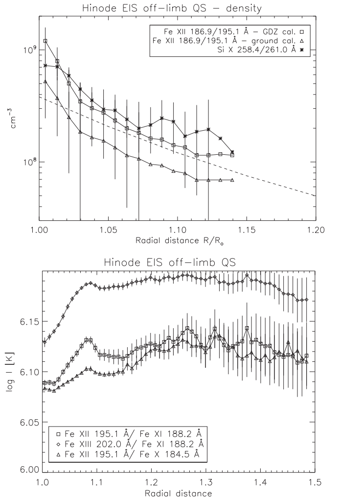
Figure 11. Averaged densities and temperatures obtained from EIS.
