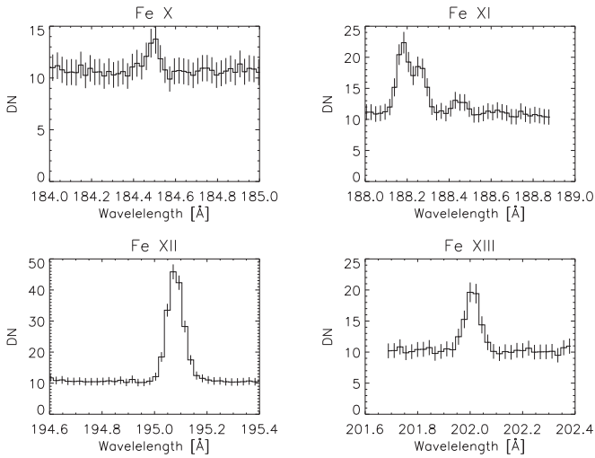
Figure 10. Hinode EIS spectra of the stronger lines at 1.5 R_{\odot} .
