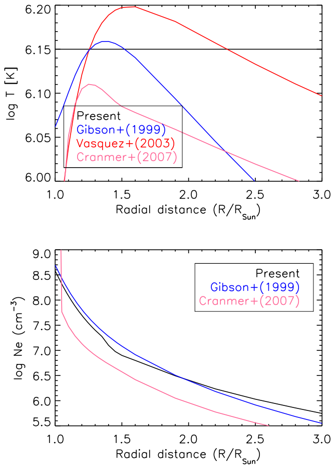
Figure 1. Radial profiles of the electron densities and temperatures we assumed for modeling quiet Sun streamers (black lines), compared to some literature values.
