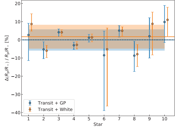
Figure 10. Comparison of the ratio between the planetary and stellar radius, R_p/R_* , estimated by the two different transit models considered. The blue points refer to the new combined model, which captures both stellar and transit signals simultaneously. The orange points refer to a simple transit model with white noise. The data points represent the relative deviation with respect to the input values and their respective uncertainties. The blue and orange solid lines and shaded areas, respectively, show the median and standard deviation of the corresponding data points. The black dotted line is the zero offset. The stars in the x -axis are ordered by decreasing SDE (ranging from 6.47 to 4.72).
