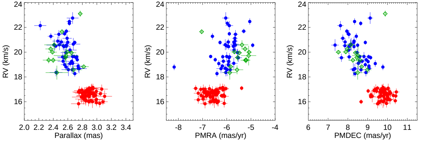
Fig. 2. Comparison between the RVs from Jeffries et al. (2014) and the Gaia parallaxes and proper motions for stars with P_{\text{Gaia}} > 0.75 . For comparison we also plot the NGC 2457 B members from Sacco et al. (2015). Symbols and colours are the same as in Fig. 1.
