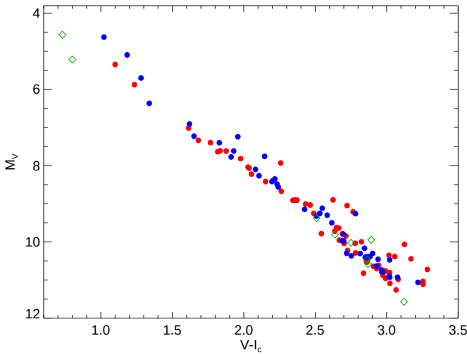
Fig. 3. Absolute V magnitude vs. V - I_c colour for the members of Gamma Vel A and B with P_{\text{Gaia}} > 0.75 . VI_c photometry is from Jeffries et al. (2009). For comparison, we also plot the NGC 2457 B members with available VI_c photometry from Sacco et al. (2015), assuming the same average distance as Gamma Vel B. Colours are as in Fig. 1.
