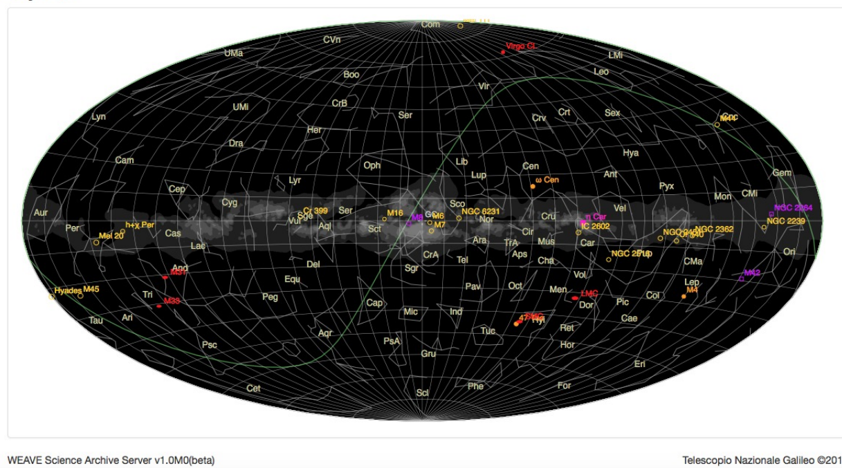
Figure 10. Main Milky Way galaxy features in galactic coordinates.
