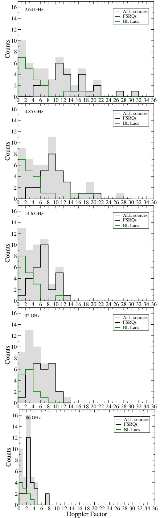
Fig. 5. Distributions of variability Doppler factors \delta_{var,eq} at selected frequencies: 2.64, 4.85, 14.6, 32, and 86 GHz from top to bottom . All sources (grey) are shown with FSRQs (black) and BL Lacs (green) superimposed. We note the systematic decrease of \delta_{var,eq} towards higher frequencies as well as the difference in the sample between FSRQs and BL Lacs (see text).
