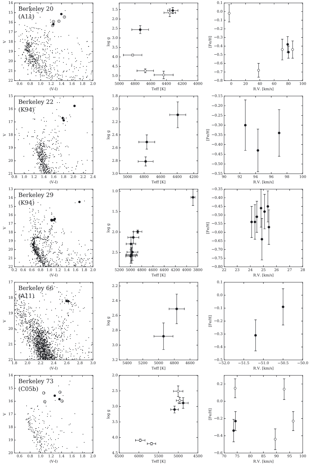
Fig. A.1. Left panels: V-I CMD of Be 20, Be 22, Be 29, Be 66, and Be 73. The spectroscopic targets analysed in this study are indicated with filled dots (for cluster members) and empty dots (non-members). Middle panels: effective temperature and surface gravity of the spectroscopic targets (as derived in this study). Right panels: radial velocities and metallicities (both as computed in this study) for the spectroscopic targets. References for photometry: A11: Andreuzzi et al. (2011) , K94: Kaluzny (1994) , and C05b: Carraro et al. (2005b) .
