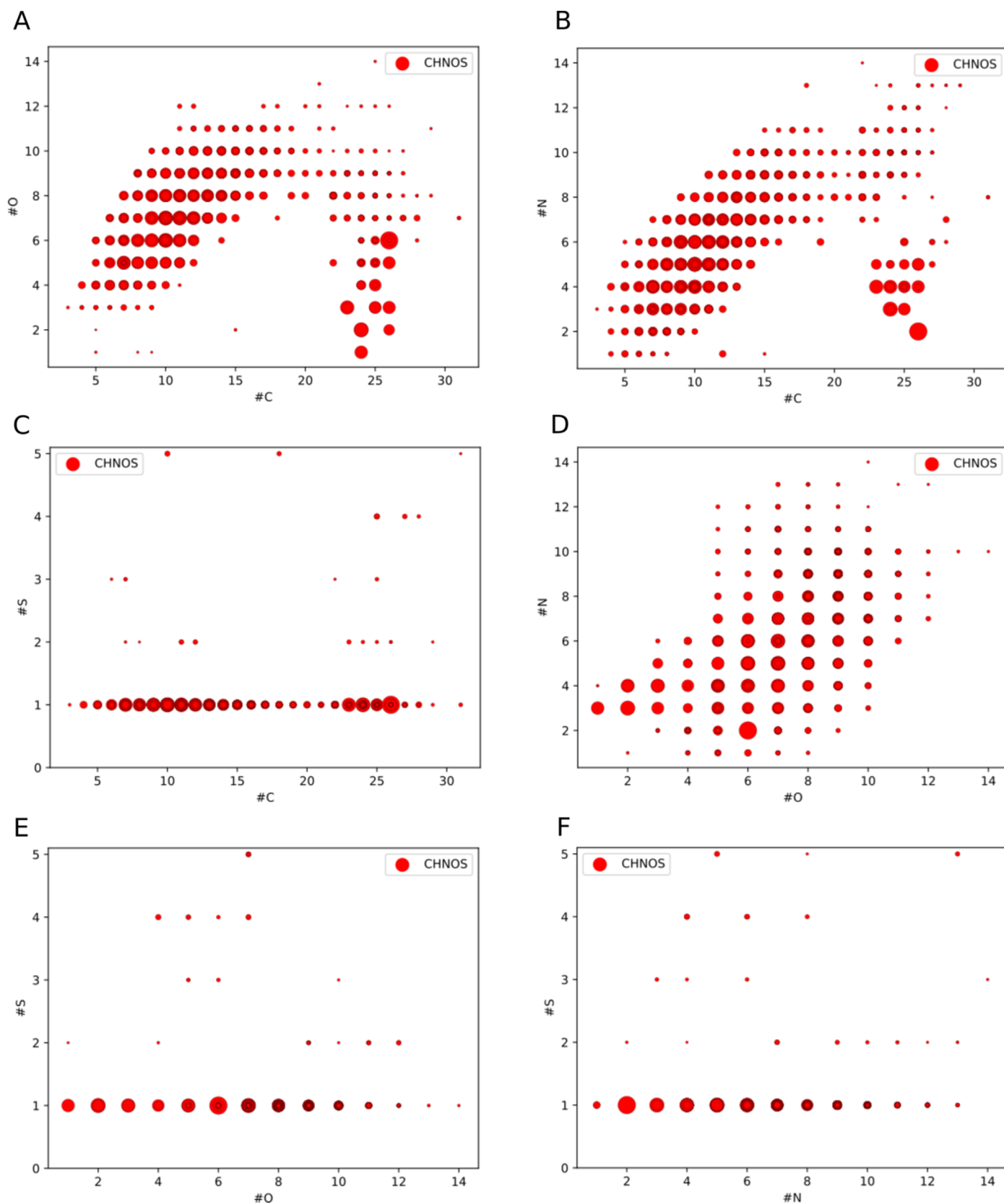
Figure 13. Atom count distributions. (A, B) Oxygen and nitrogen counts vs. carbon counts reveal two separate groups within the observed organosulfur compounds. (C, E, F) Organosulfur compounds bear mostly one sulfur atom. Among these one-S-bearing compounds, different intensity patterns are observed. (D) Nitrogen counts vs. oxygen counts show a large coverage among a large range of heteroatom counts. This indicates a rich diversity in heteroatom chemistry within the observed organosulfur compounds. The bubble size scales with mass spectrometric intensity.
