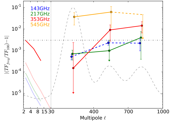
Fig. 41. Transfer function ratio, referred to 100 GHz, for various multipoles. For \ell = 2-30 , the solid red line is the measured 353 GHz empirical SRO11 time TF. The red dotted line shows an upper limit on the 353 GHz residuals after correction, while blue and green dotted lines show an estimate of the residuals at 143 and 217 GHz. The TF for \ell = 30-1000 is estimated from CMB anisotropies on the first three acoustic peaks (with negative values displayed by dashed lines). The grey dashed line is a CMB power spectrum, showing the position of the first three acoustic peaks.
