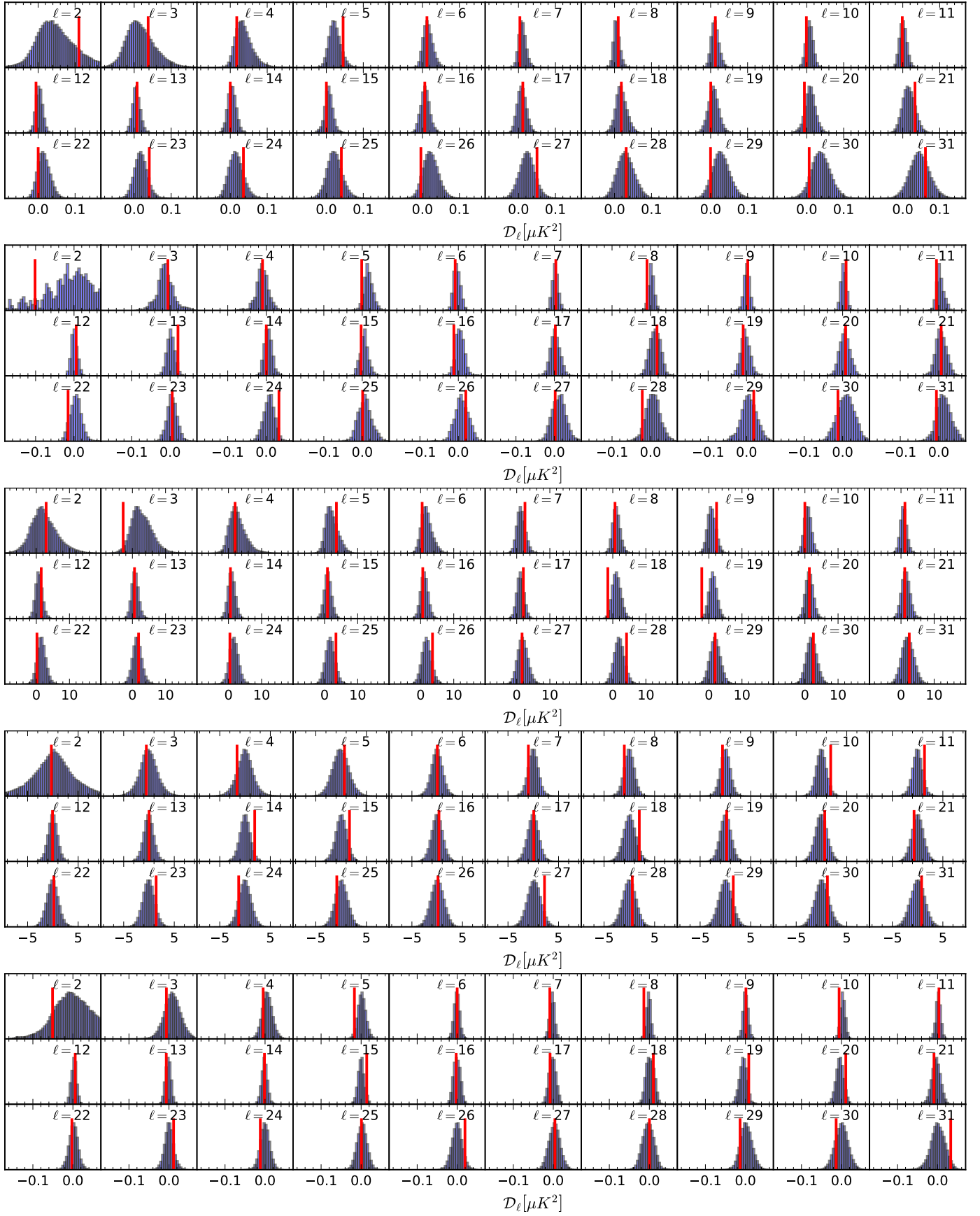
Fig. 16. Probability distribution for each multipole ( \ell = 2 – 31 ) of the 100 \times 143 cross-spectra, from the top panels to the bottom ones, showing EE , BB , TE , TB , and EB . Red vertical lines show the values for the data. The associated PTEs are given in Table 4.
