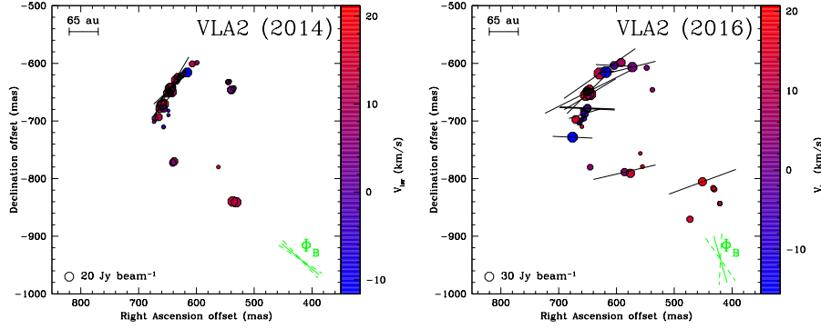
Figure 2: A close-up view of the 22 GHz \text{H}_2\text{O} maser features detected with the EVN around the radio sources VLA 2 in epochs 2014.46 (left panels) and 2016.45 (right panels). The reference position in epoch 2014.46 is \alpha_{2000} = 20^{\text{h}}38^{\text{m}}36^{\text{s}}.43399 and \delta_{2000} = 42^{\circ}37'34''.8710 ; while in epoch 2016.45 is \alpha_{2000} = 20^{\text{h}}38^{\text{m}}36^{\text{s}}.43403 and \delta_{2000} = 42^{\circ}37'34''.8667 . The octagonal symbols are the identified maser features. The linear polarization vectors, scaled logarithmically according to polarization fraction P_l , are overplotted. In the bottom-right corner the error-weighted orientation of the magnetic field ( \Phi_B ) is also reported; the two dashed segments indicate the uncertainties.
