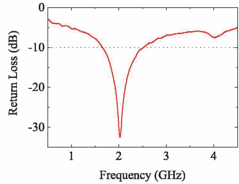
Fig. 3: The reflection coefficient S_{11} of the antenna.
