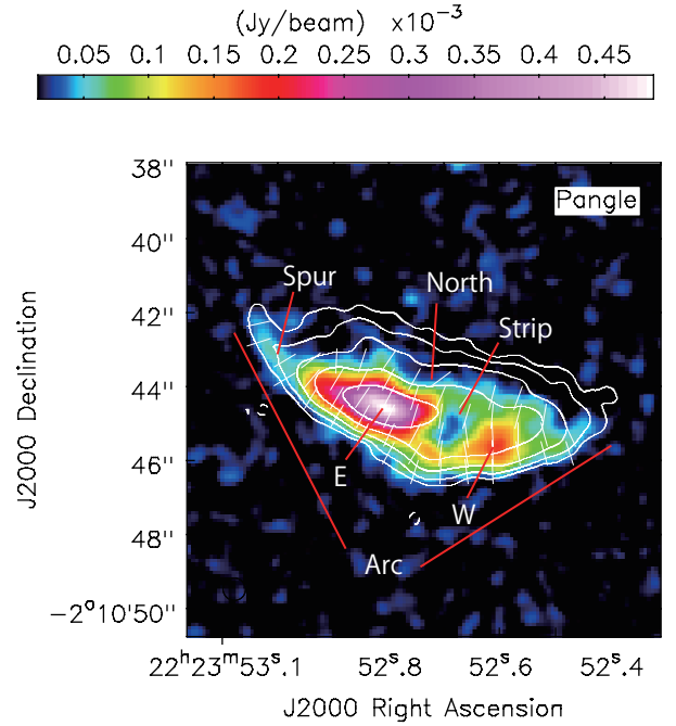
Figure 1. ALMA image at 97.5 GHz of 3C 445 South in total intensity (contours) overlaid on polarization intensity (colour-scale). The total intensity peak flux density is 1.3 \text{ mJy beam}^{-1} . The first contour is 45 \mu\text{Jy} , which is 3 times the rms measured on the total intensity image. Contours increase by a factor of 2. The polarization intensity colour scale is shown by the wedge at the top of the image. The 1\text{-}\sigma noise level measured on the polarization image plane is 12 \mu\text{Jy beam}^{-1} . Vectors represent the electric vector position angle. The restoring beam is plotted on the bottom left corner.
