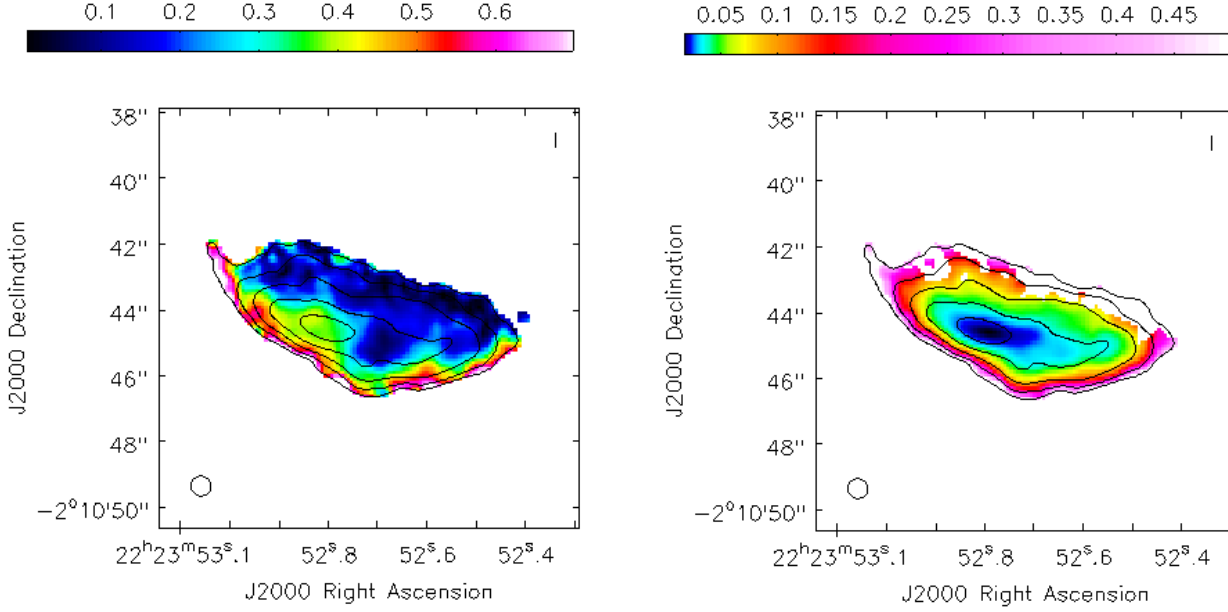
Figure 2. ALMA image at 97.5 GHz of 3C 445 South in total intensity (contours) overlaid on the fractional polarization ( left panel ) and fractional polarization error ( right panel ) images (colour-scale). The total intensity peak flux density is 1.3 \text{ mJy beam}^{-1} . The first contour is 45 \mu\text{Jy} , which is 3 times the rms measured on the total intensity image. Contours increase by a factor of 2. The fractional polarization and the fractional polarization error colour scales are shown by the wedge at the top of the images. The restoring beam is plotted on the bottom left corner.
