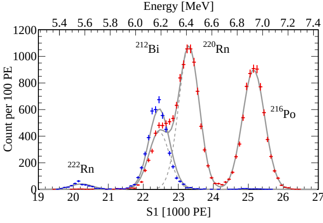
FIG. 4. The alpha spectrum of the ^{220}\text{Rn} decay chain is shown integrated over times during which the source is open (40.3 hours, red) and after (148.7 hours, blue) the source is closed. The constant background of ^{222}\text{Rn} (Figure 2) is visible only over the longer time period.
