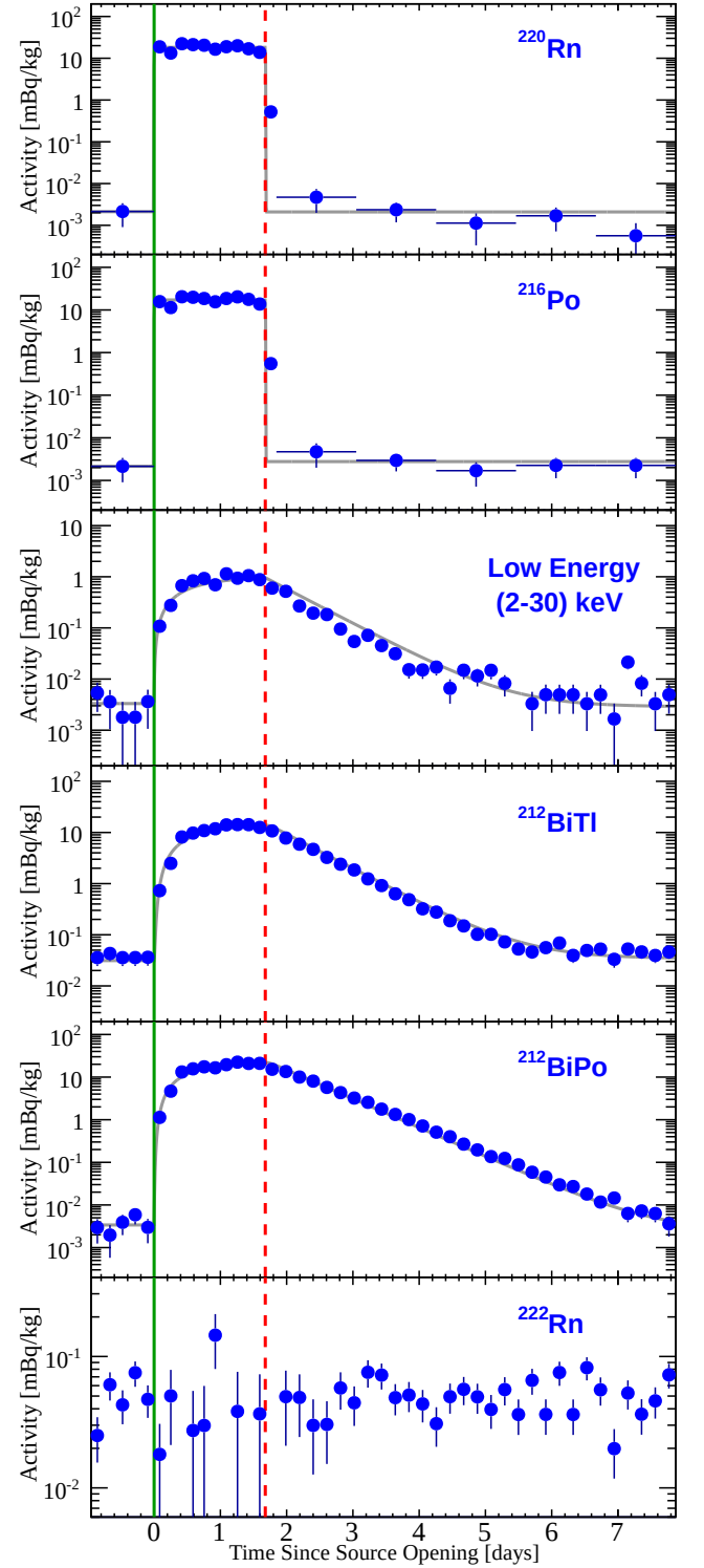
FIG. 2. Time evolution of isotopes in the ^{220}\text{Rn} decay chain and the ^{222}\text{Rn} background. Times at which the source was opened and closed are indicated by the solid green and the dashed red lines. The opening of the source is defined as time t = 0 . Gray curves show the numerical model of the growth and decay of each isotope, scaled to the observed rate. Binning for ^{220}\text{Rn} and ^{216}\text{Po} is adjusted for times of low activity.
