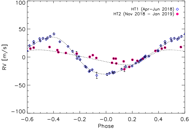
Fig. 10. Comparison between the VIS RVs obtained from TERRA pipeline in the two different observing seasons: HT1 (blue diamonds) and HT2 (pink dots).
