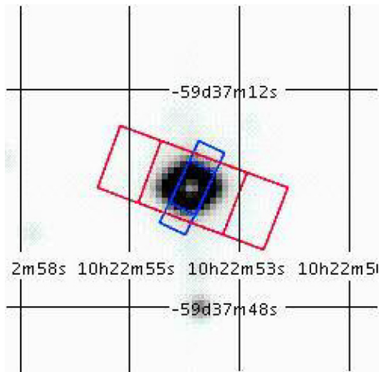
Figure 3. Overplot of the IRS spectral slits, for both high resolution modules, on the 2MASS K_s image. The smaller aperture (blue box in the electronic edition) corresponds to the SH aperture, the larger one (red box in the electronic edition) is the LH aperture.
