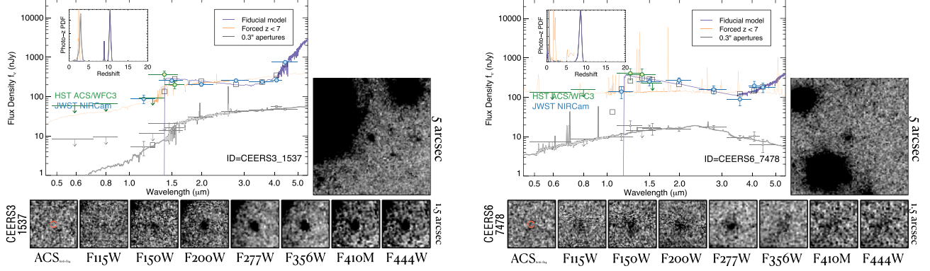
Figure 19. Two sources that had incorrectly drawn Kron apertures due to the presence of nearby bright sources. The large plot shows the SED, with the Kron NIRC (HST) photometry in blue (green). The best-fit EAZY model to these data is shown in purple (with squares denoting the model bandpass-averaged fluxes), with the best-fit z < 7 solution shown in orange. The small gray circles show the fluxes measured in 0.3'' diameter apertures, with the gray line showing the EAZY fit to these small-aperture fluxes. The P(z) s for all three EAZY runs are shown in the top left. The large image shows a 5'' \times 5'' cutout around each source, highlighting the nearby neighbor responsible for stretching the Kron aperture, leading to much brighter Kron fluxes. The small images show a 1.5'' region around each source in the seven NIRC bands (and the stacked ACS dropout bands), with the red circle denoting a 0.3'' diameter region around the source. The P(z) from the colors measured in this small circular aperture prefers lower redshifts in both cases; thus, these sources were removed from the sample.
