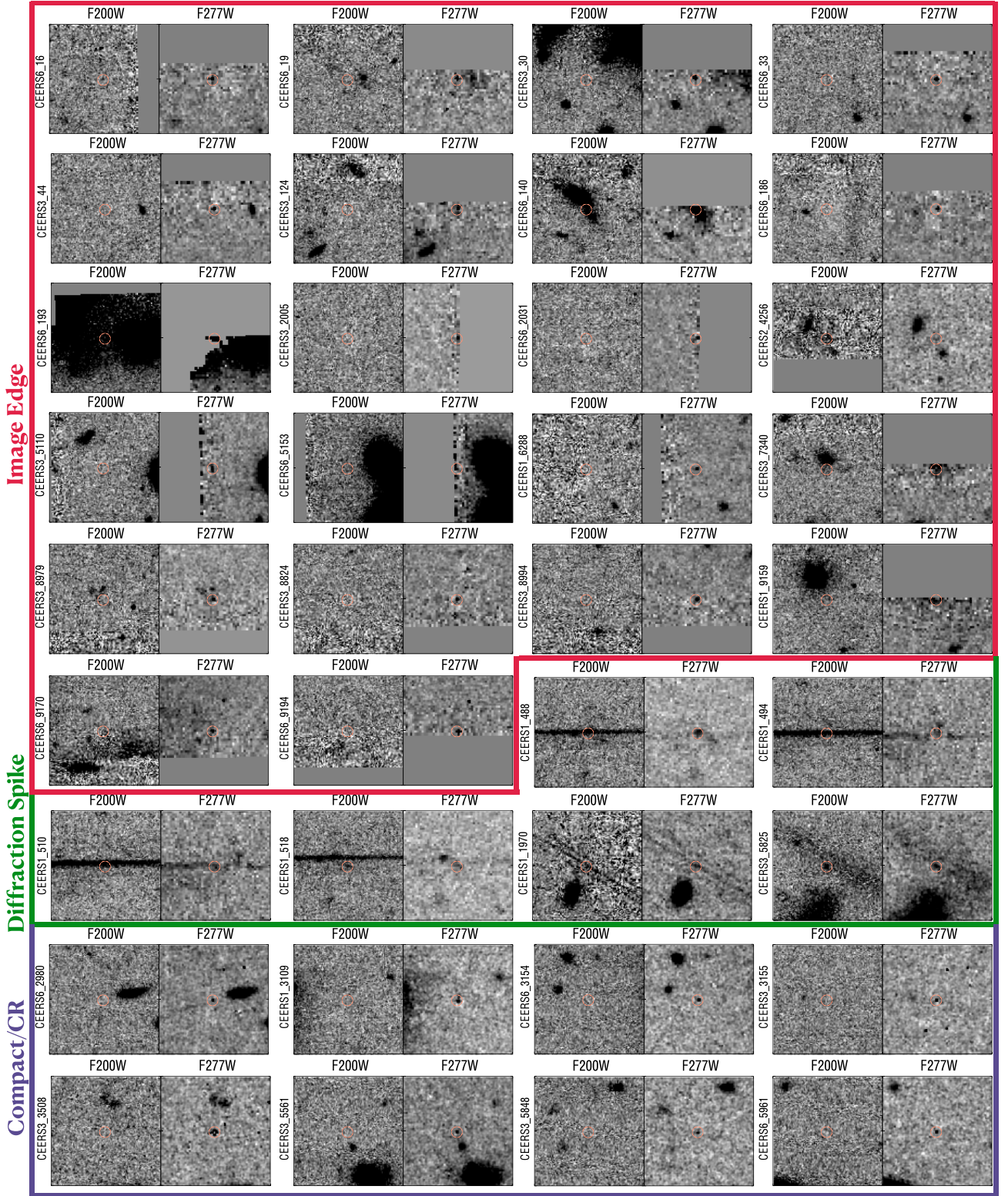
Figure 20. This compilation shows 3'' \times 3'' cutout images of the 36 sources identified as spurious from our visual inspection of the initial list of candidates. The majority of these spurious detections come from very near the image edges, which are easily identifiable (and can be automated in the future). Six objects are obvious diffraction spikes. The remaining eight sources are very compact and boxy and visible only in the LW channels. We conclude that these are highly likely to be unflagged cosmic rays, which will be better flagged in future reductions (M. Bagley et al. 2022, in preparation). We note that seven out of eight are in the CEERS3 or 6 pointings, which had fewer images with longer exposure times than CEERS1 and 2, leading to more numerous cosmic-ray hits.
