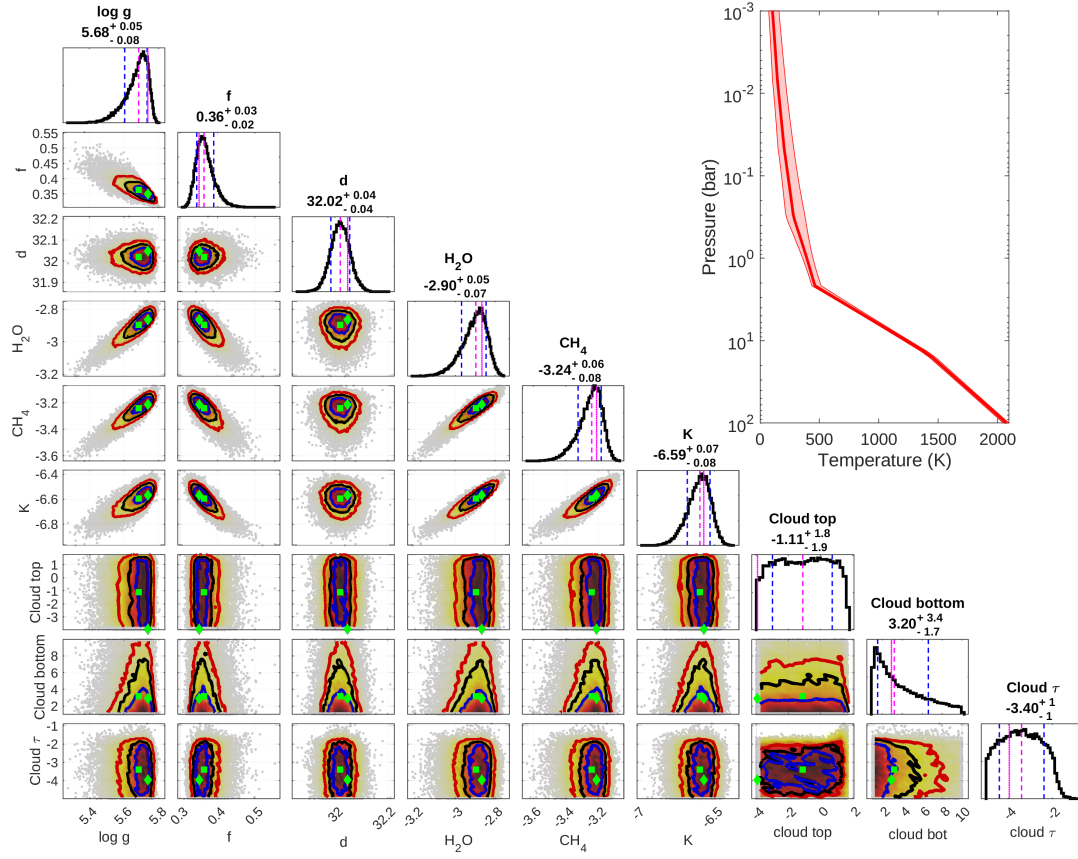
Figure A2. Posterior distributions for the retrieval of HD 19467 B using the full available spectrum. See caption of Figure 11 for details on the posterior plots.
