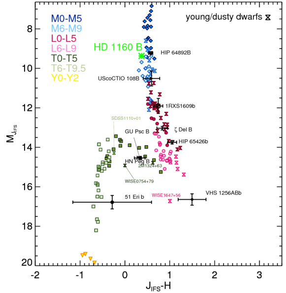
Figure 6. Absolute J magnitude vs. J-H color-magnitude diagram with the position of HD 1160 B that is indicated by a green asterisk. The positions of field M, L and T dwarfs are also represented in different colors according to the spectral type. Black asterisk represents the positions of other substellar companions.
