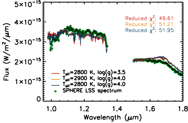
Figure 4. Comparison of the extracted spectrum for HD 1160 B (green squares) with the three best fit theoretical BT-Settl spectra (orange, red and blue solid lines).
