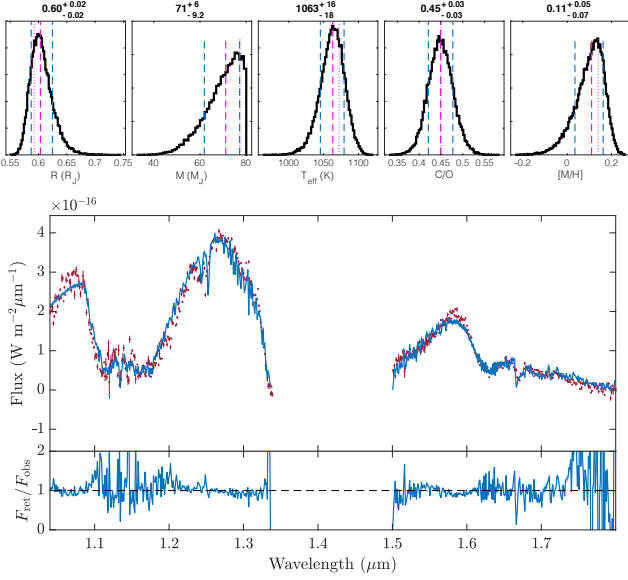
Figure A1. Top: Posterior distributions of derived quantities for the retrieval of HD 19467 B. The posteriors are shown for the brown dwarf radius R , its mass M , effective temperature T_{\text{eff}} , the C/O ratio, and the overall metallicity [M/H] . Bottom: Posterior spectra and residuals. The solid lines refer to the median of all posterior spectra. The shaded areas signify the 3\sigma confidence intervals of the spectra. The measured spectrum is indicated by the red data points.
