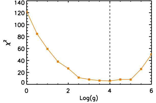
Figure 5. Values of the \chi^2 obtained from the fit versus the values of \log g for a fixed T_{eff} of 2800 K. The vertical dashed line highlights the position of the minimum of the curve.
