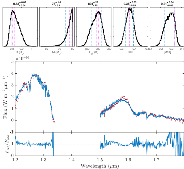
Figure 12. Top: Posterior distributions of derived quantities for the retrieval of HD 19467 B. The posteriors are shown for the brown dwarf radius R , its mass M , effective temperature T_{\text{eff}} , the C/O ratio, and the overall metallicity [M/H] . Bottom: Posterior spectra and residuals. The solid lines refer to the median of all posterior spectra. The shaded areas signify the 3\sigma confidence intervals of the spectra. The measured spectrum is indicated by the red data points.
