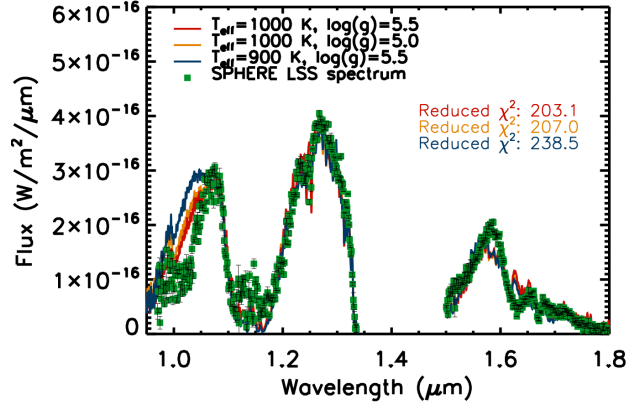
Figure 9. Comparison of the extracted spectrum for HD 19467 B (green squares) with the three best fit theoretical BT-Settl spectra (orange, red and blue solid lines).
