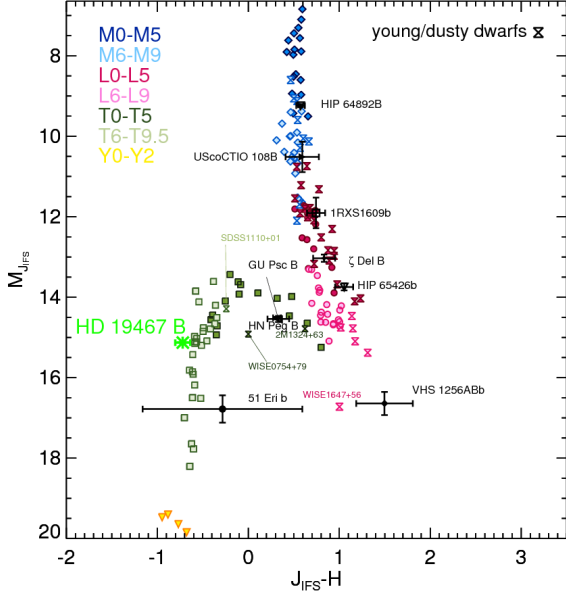
Figure 10. Absolute J magnitude vs. J-H color-magnitude diagram with the position of HD 19467 B that is indicated by a green asterisk. The positions of field M, L and T dwarfs are also represented in different colors according to the spectral type. Black asterisks represent the positions of other substellar companions.
