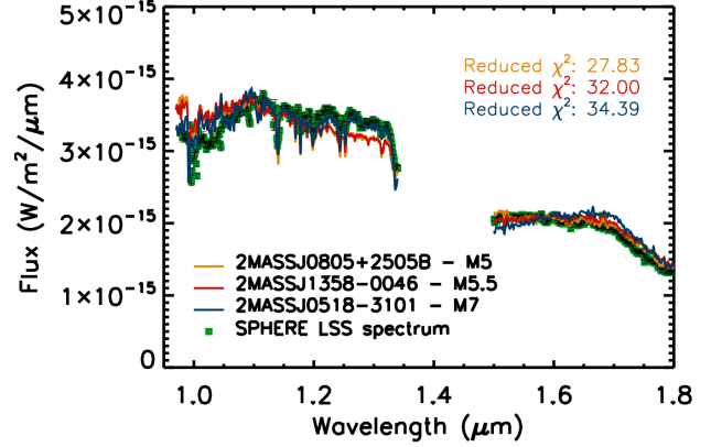
Figure 2. Comparison of the extracted spectrum for HD 1160 B (green squares) with the three best fit spectra from the Montreal library (red, orange and blue solid lines).
