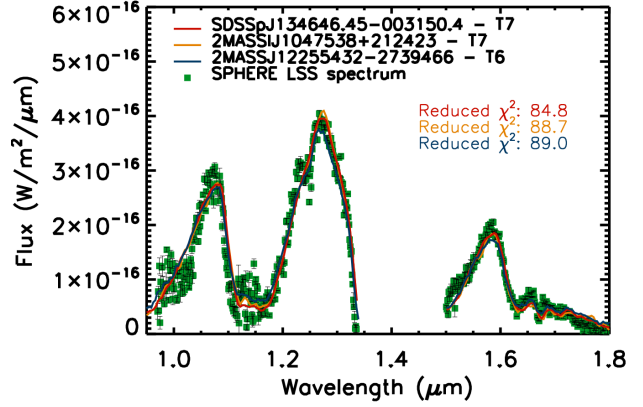
Figure 8. Comparison of the extracted spectrum for HD 19467 B (green squares) with the three best fit spectra from the SpeXPrism library (red, orange and blue solid lines).
