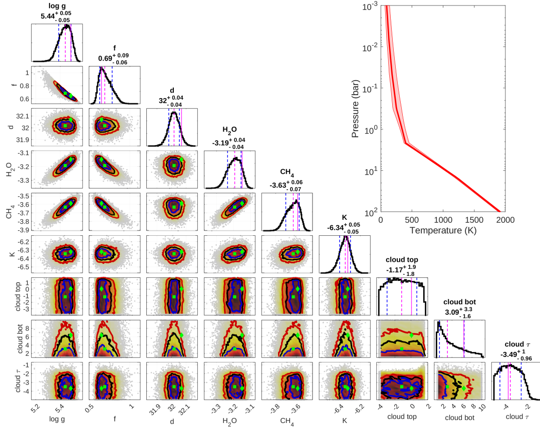
Figure 11. Posterior distributions for the retrieval of HD 19467 B. The dashed magenta-colored lines in the posterior plots refer to the location of the median value (also stated below each parameter), while the 1\sigma confidence limit is denoted by the blue dashed lines. The magenta dotted line shows the location of the best-fit model, i.e., the one with highest likelihood value. The solid blue, red, and yellow lines in the two-dimensional parameter correlation plots mark the 1\sigma , 2\sigma , and 3\sigma intervals, respectively. Here, the location of the median (best-fit) model is marked by green squares (diamonds). The panel in the upper, right corner depicts the retrieved temperature profile. The solid red line corresponds to the median profile, while the shaded, red area corresponds to the 1\sigma confidence interval.
