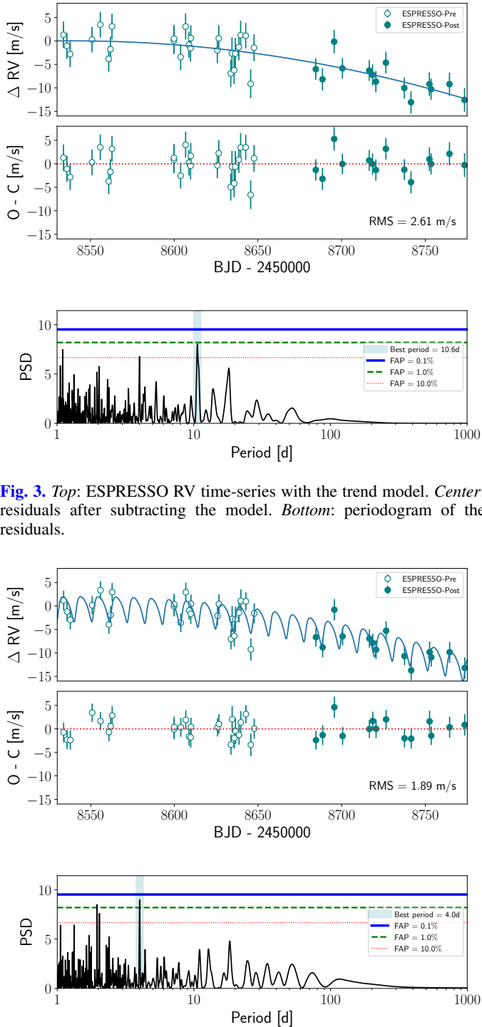
Fig. 4. Top: ESPRESSO RV time-series with a model that includes a trend and the planetary signal from K2-38c. Center: residuals after subtracting the model. Bottom: periodogram of the residuals.
