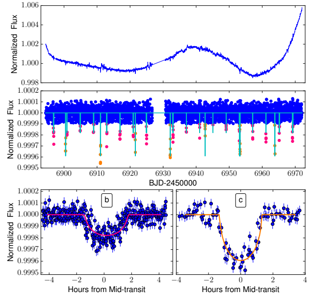
Fig. 1. Top: normalized flux of the light curve extracted using the EVEREST pipeline. Middle: detrended light curve with the transits of K2-38b and K2-38c marked with different colors. Bottom: folded light curve using the period of K2-38b ( P = 4.02 d) and K2-38c ( P = 10.56 d).
