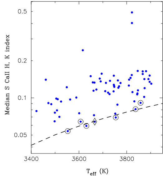
Fig. 2. Median S index for each star vs. stellar effective temperature. The dashed line represents a fit to those stars with the lowest S values (shown with circles). The star GJ 4196 (see text) is shown with a diamond symbol.
