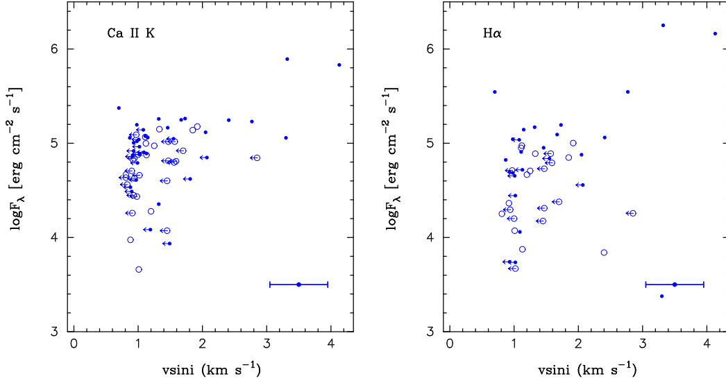
Fig. 6. Ca II K (left) and H \alpha (right) line emission excess flux vs. v \sin i . Possible young stars according to our kinematic analysis are shown with filled symbols. Upper limits on v \sin i are shown with arrows, while the typical error bar is shown in the lower right corner.
