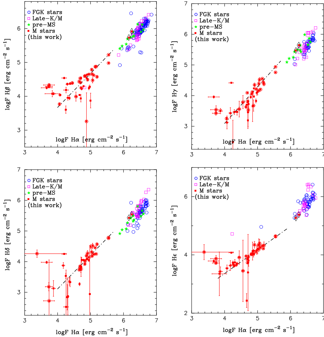
Fig. 11. Flux-flux relationships between Balmer lines: H\alpha , H\beta (top left panel); H\alpha , H\gamma (top right panel); H\alpha , H\delta (bottom left); and H\alpha , H\epsilon (bottom right). Colours and symbols are as in Fig. 10.
