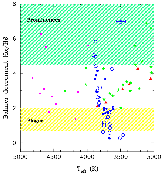
Fig. 9. Balmer decrement F_{\text{H}\alpha}/F_{\text{H}\beta} vs. the effective temperature. Possible young stars are shown with filled symbols. Green stars denote pre-MS M stars from Stelzer et al. (2013a), red triangles correspond to the active M dwarf templates from the Sloan Digital Sky Survey (Bochanski et al. 2007), while data from Frasca et al. (2015) is shown in purple squares. Typical ranges of solar plages and prominences are shown as hatched areas. Typical uncertainties are also shown.
