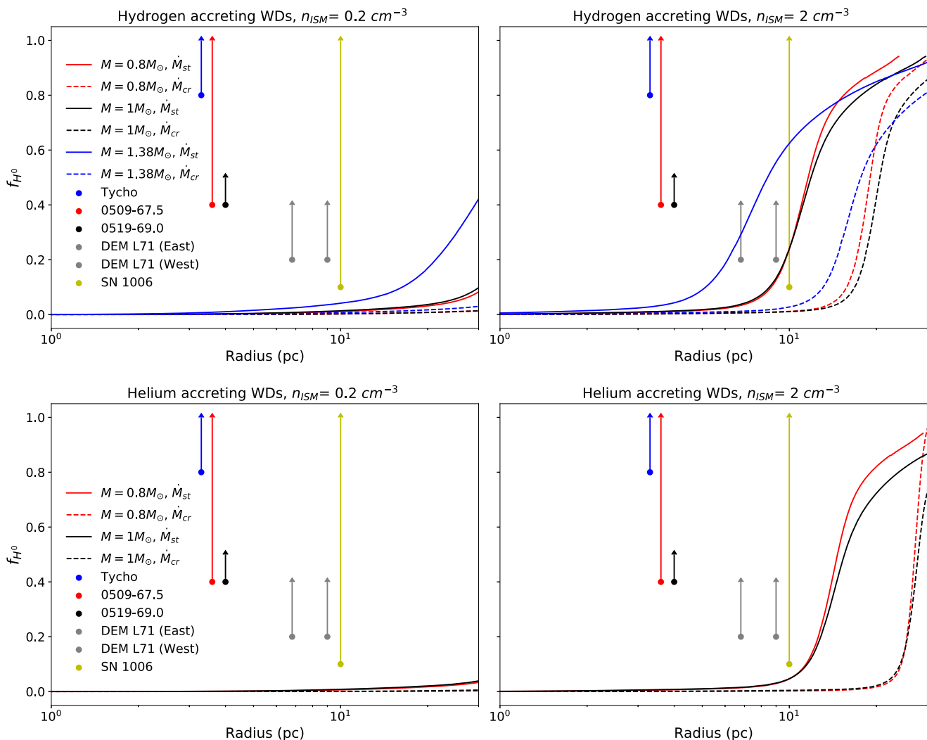
Figure 6. Hydrogen neutral fraction as a function of radial distance from CO WDs accreting H- and He-rich matter at the two stability boundaries in the steady accretion regime for various WD masses. The minimum hydrogen neutral fractions at the present radius of the shock of each remnant are also plotted.
