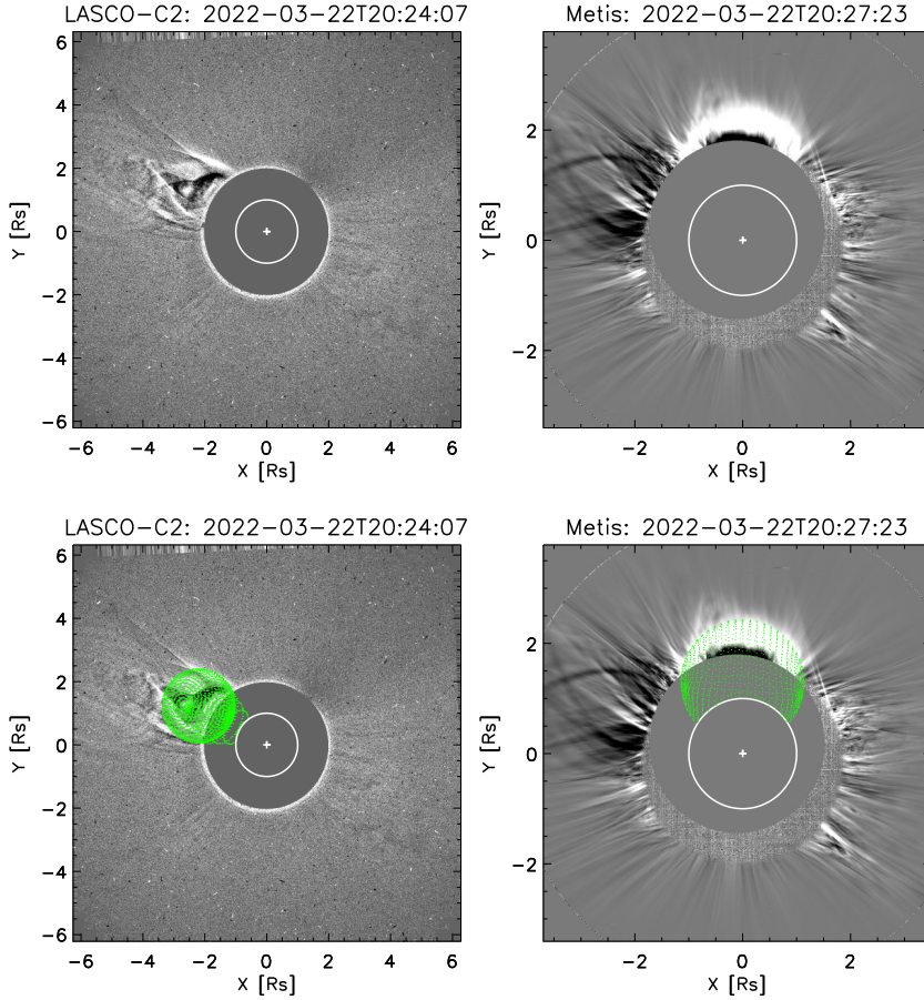
Fig. 3. 3D reconstruction of the CME using LASCO-C2 (left panels) and Metis (right panels). The times of each image are indicated at the top of each panel. The top (bottom) panels show the coronagraph images without (with) the reconstructed structure, which is shown by the green mesh.
