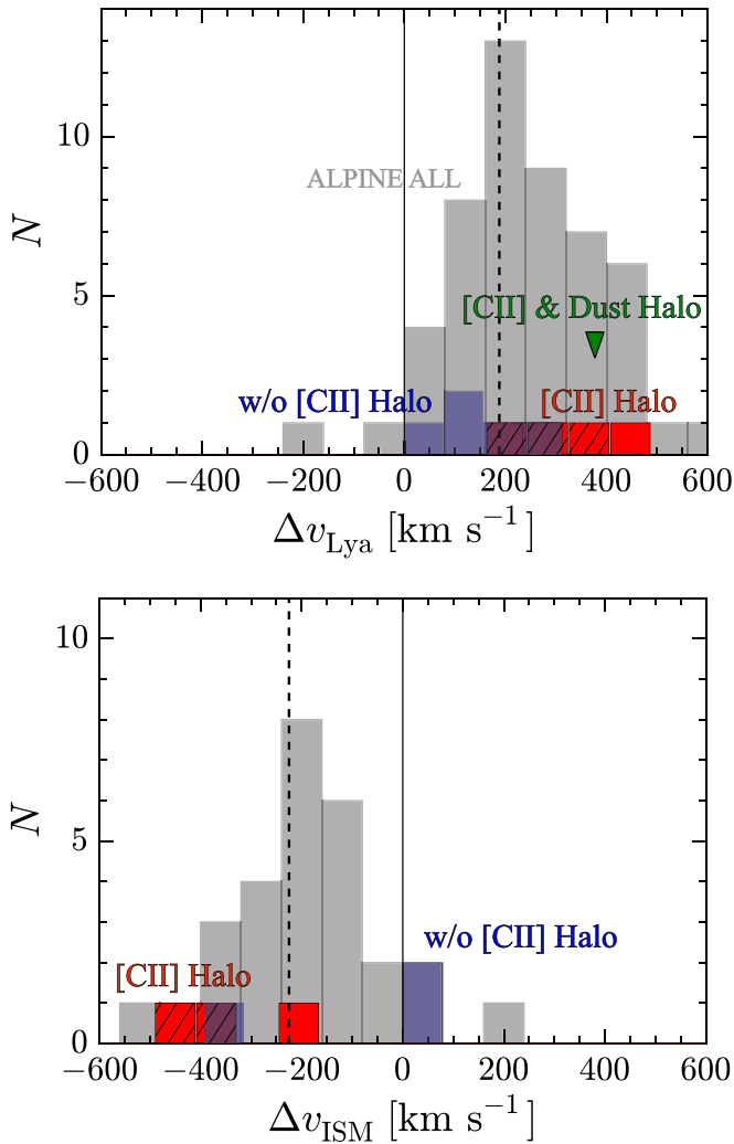
Figure 8. Histograms showing the velocity offsets ( \Delta v ) of the the \text{Ly}\alpha line (top) and the rest-frame UV metal absorption (bottom) with respect to the [C II] line that traces the systemic redshift. The red and blue histograms denote the [C II] Halo and w/o [C II] Halo objects. The three [C II] Halo objects marked with black squares in Figure 6 are presented in the hatched histogram. The green downward-pointing triangle in the top panel indicates the \Delta v_{\text{Ly}\alpha} value of the [C II] & Dust Halo object. The gray histogram shows the entire sample of the 53 and 29 ALPINE sources whose \text{Ly}\alpha line and rest-frame UV metal absorption have been identified among the [C II]-detected 75 ALPINE sources (see Cassata et al. 2020; Faisst et al. 2020). The solid and dashed lines denote the velocity center traced by the [C II] line and the median value of the entire sample, respectively.
