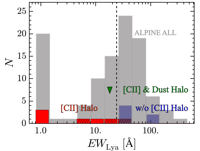
Figure 7. Histogram of the \text{Ly}\alpha EW. The red and blue histograms indicate the [C II] Halo and w/o [C II] Halo objects. The three [C II] Halo objects marked with black squares in Figure 6 are shown in the hatched histogram. The green downward-pointing triangle denotes the \text{Ly}\alpha EW value of the [C II] & Dust Halo object. The gray histogram shows the entire sample of the 116 ALPINE sources whose \text{Ly}\alpha line spectroscopy is available (see Cassata et al. 2020). The first (leftmost; \sim 1 Å) bin presents the objects whose \text{Ly}\alpha lines are undetected in the optical–NIR spectroscopy. The dashed line denotes the median of the entire sample excluding the sources whose \text{Ly}\alpha lines are undetected.
