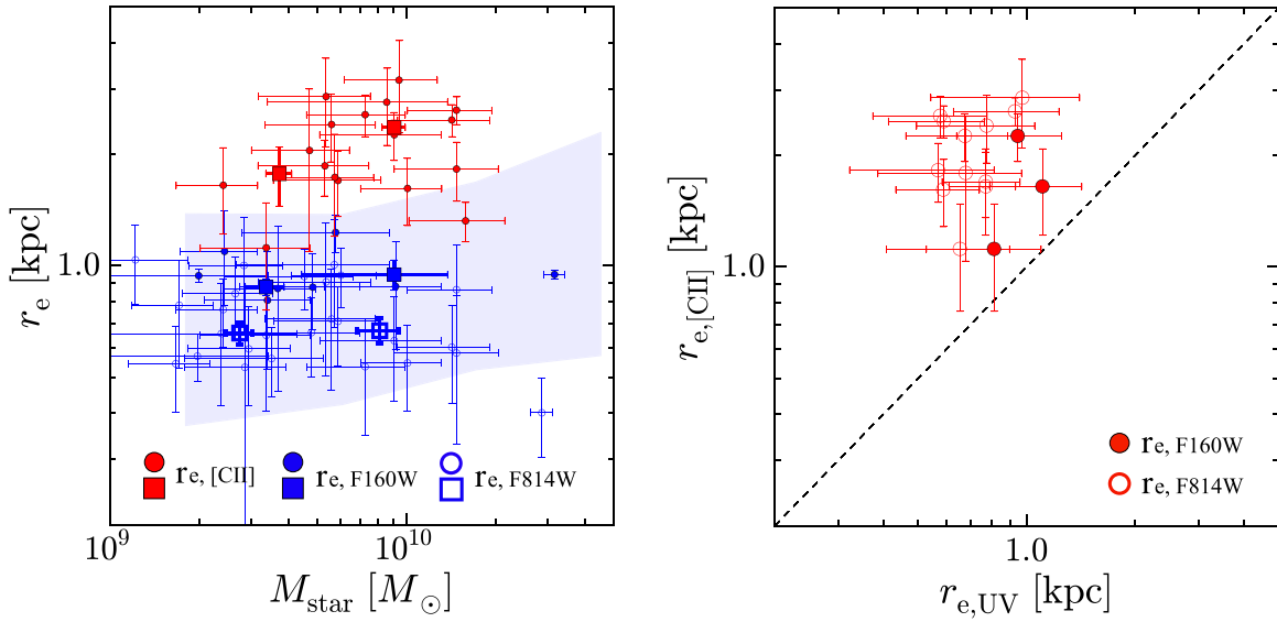
Figure 2. Physical sizes of ALPINE sources. Left: size vs. stellar mass. Red and blue circles indicate our [C II] and rest-frame UV size measurements as a function of M_{\text{star}} . The squares represent the median values in bins of M_{\text{star}} , where the error bars denote the standard error of the median. We present the reliable size measurement results (flag = 0) of the [C II] line and rest-frame UV for the 19 and 32 ALPINE sources, respectively, that are not classified as mergers. Both F814W and F160W measurements are shown for six ALPINE sources. Blue open and filled symbols denote the rest-frame UV size measurements in the HST/F814W and F160W maps, respectively. The blue shaded region gives the 1\sigma range of the rest-frame UV size distribution of \sim 4000 normal star-forming galaxies presented in Shibuya et al. (2015). Right: comparison between [C II] and rest-frame UV sizes among the individual galaxies. The red open and filled circles indicate whether the rest-frame UV sizes are estimated from the HST/F814W and F160W maps, respectively. We present the [C II] and rest-frame UV size measurements for 12 ALPINE sources whose measurements are reliably (flag = 0) obtained. Both F814W and F160W measurements are shown for three ALPINE sources.
