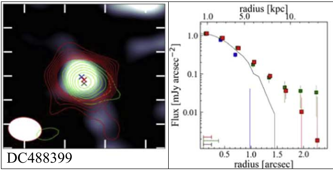
Figure 4. Representative examples of the spatial distributions of the [C II] line, the rest-frame FIR, and UV continuum. The remaining objects are presented in Figure B1. By evaluating the extended components, we identify three categories: [C II] Halo, w/o [C II] Halo, and [C II] & Dust Halo objects (see text). Left: the grayscale ( 6'' \times 6'' ) image shows the rest-frame UV emission from the HST imaging (Koekemoer et al. 2007, 2011). Red and green contours denote the 2.5\sigma , 3.5\sigma , 4.5\sigma , ..., 9.5\sigma levels of the ALMA [C II] line and the rest-frame FIR continuum emission, respectively. The green contour is presented only for the sources whose dust continuum emission is detected above the 5\sigma level. The HST image and ALMA contours are smoothed by the ALMA synthesized beam and the HST PSF, respectively, to match the spatial resolutions between the HST and ALMA maps. The smoothed PSF is shown at the lower left. The red, green, and blue crosses mark the peak pixel positions of the [C II] line, the rest-frame FIR, and UV continuum, respectively. Right: radial surface brightness profiles of the [C II] line (red squares), the rest-frame FIR (green squares), and UV (blue squares) continuum. The black solid curve shows the ALMA synthesized beam. All radial profiles are estimated from the median value in an annulus with a width of 0''.3 , and their peaks are normalized to the [C II] one. The errors denote the 16th–84th percentile of the median values in 100 random annuli. The spatial offsets between UV–[C II], UV–FIR, and [C II]–FIR peaks are presented in the red, green, and black bars at the lower left. For the HST maps with foreground objects removed, the radial profiles of the rest-frame UV continuum are shown by open blue squares.
