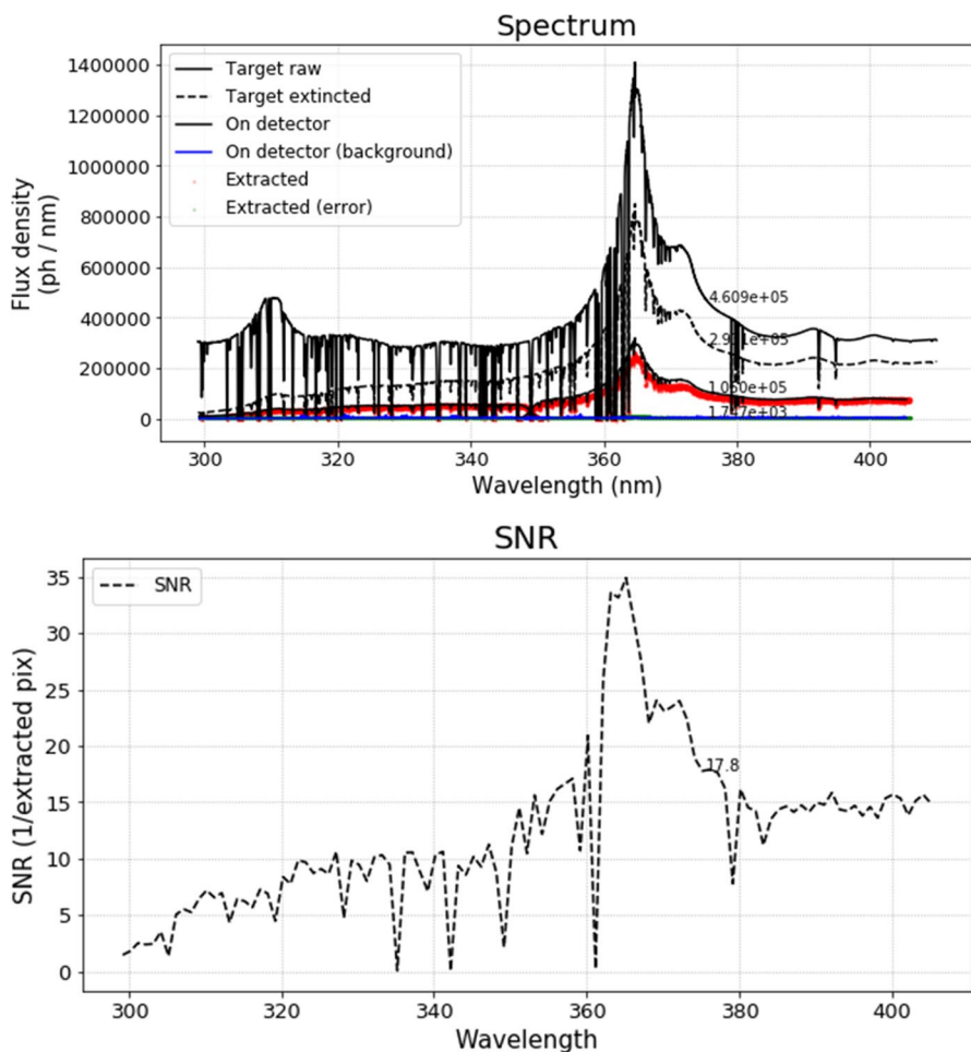
Fig. 5 Output of the E2E simulator for the case of a quasar at z_{\text{em}} = 2.5 with magnitude u(\text{AB}) = 18 observed for 600s. The upper panel shows the input spectrum (solid black line, target raw ), the input spectrum with atmospheric extinction (dashed black line, target extincted ), the spectrum that is seen by the detector, i.e. scaled by telescope and instrument efficiency (solid black line, on detector ), the background seen on the detector (solid blue line, on detector background ), the spectrum recovered by simple (non-optimal) extraction (red dots, extracted ), the error on the extracted spectrum (green dots, extracted error ). In the lower panel the signal-to-noise ratio per pixel is reported
