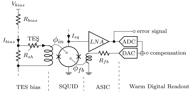
Figure 4. Layout of the TES, SQUID and ASIC operating in flux-locked loop.
