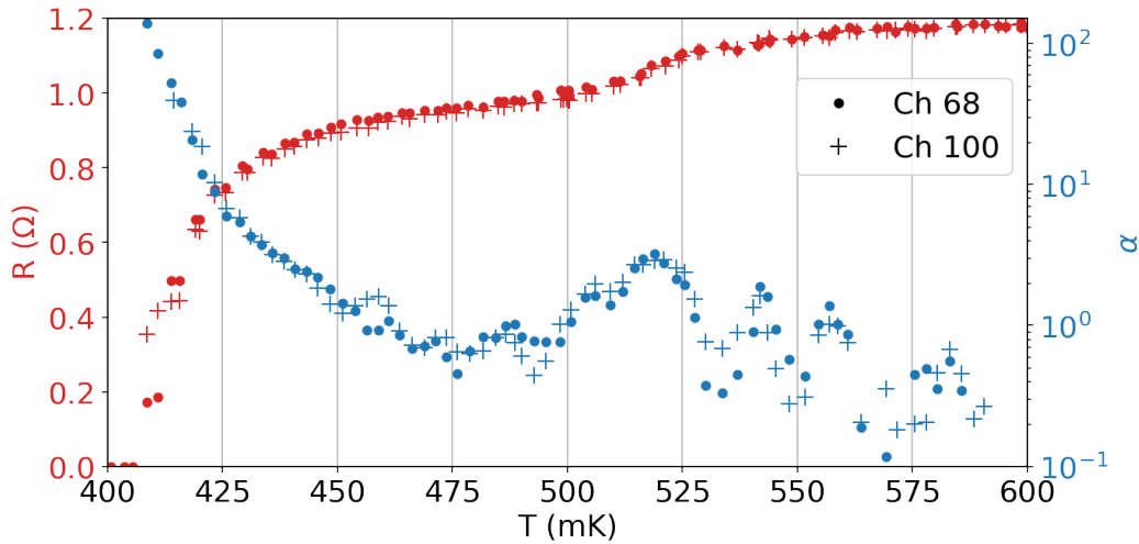
Figure 14. Resistance as a function of temperature for array P87 dark pixels on channels 68 and 100 (red) and derived \alpha = \frac{T}{R} \times \frac{\partial R}{\partial T} parameter (blue).
