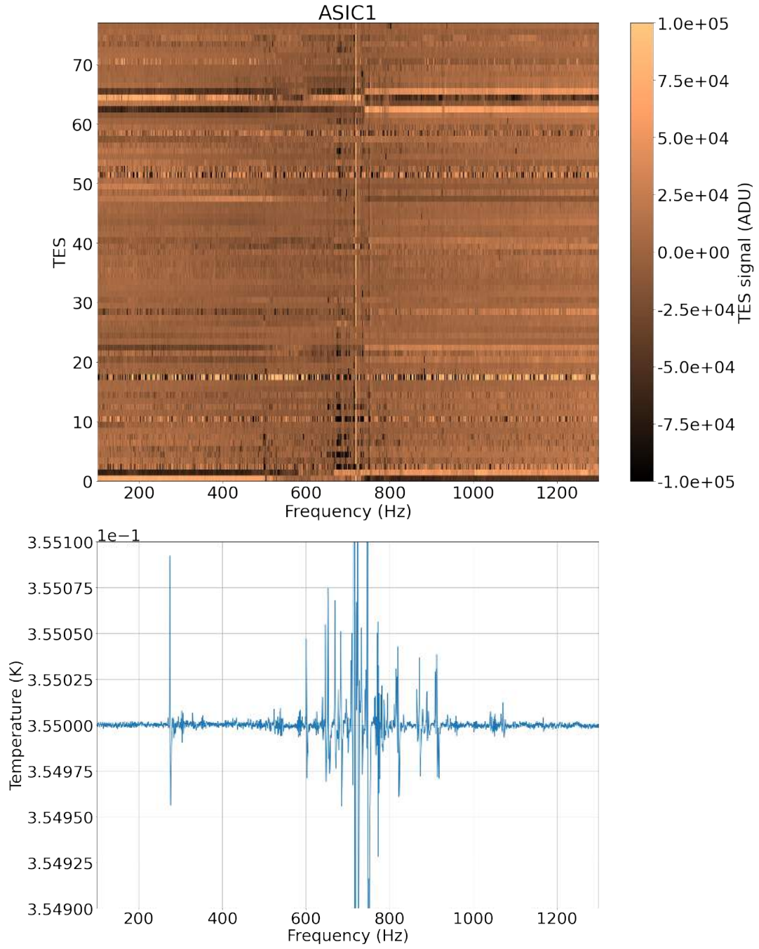
Figure 29. Top: Time ordered signals in ADU of some TES with the time axis converted in frequency of the mechanical excitation. Bottom: Temperature of the TES stage as a function of the frequency of excitation. The graphs have been adjusted to share the same x-axis. At mechanical excitation frequencies between about 600 Hz and 800 Hz, resonances are clearly seen on the TES signals and in the TES stage temperature.
