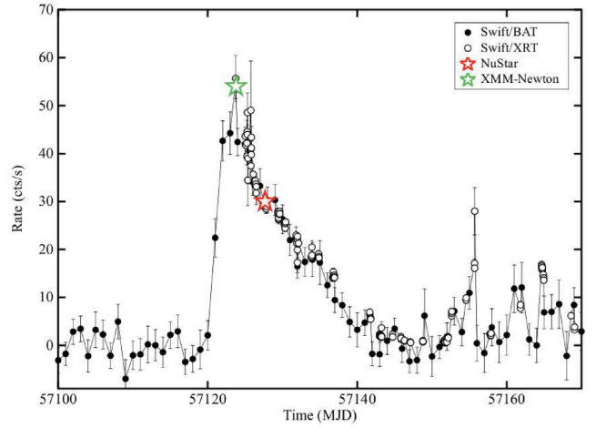
Figure 1. Swift /BAT and XRT light curve during the 2015 outburst of SAX J1808.4–3658. The dates of the XMM–Newton and NuSTAR observations are indicated with stars.
