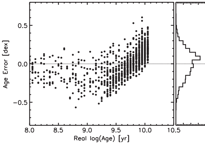
Figure 9. Age error as a function of true age for the simulated sample found using [\text{Fe}/\text{H}] , T_{\text{eff}} , M_{VT} , and \log g as measured parameters for a Bayesian analysis. Using this method of age estimation, the young stars are assigned ages that are preferentially too old and the old stars are assigned ages that are preferentially too young. The right panel shows the histogram of age errors as shown in the lower right panel of Figure 7.
