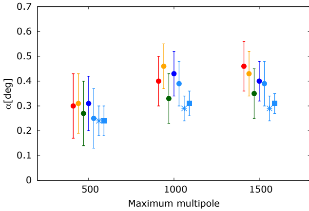
Fig. 5. Birefringence angle estimates (in degrees) versus the maximum multipole considered. Only (1\sigma) statistical uncertainties are shown here; with systematic errors discussed later. Commander is shown in red, NILC in orange, SEVEM in green, SMICA (full-mission data) in blue, and SMICA (half-mission data) in cyan. Dot symbols refer to the estimates obtained with the D_\ell^{TB} estimator. Star symbols refer to estimates coming from D_\ell^{EB} and squares are obtained through the combination of D_\ell^{TB} and D_\ell^{EB} .
