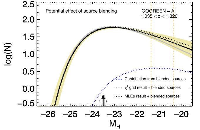
Figure 13. Potential effect of source blending on the red-sequence LF of the seven GOGREEN clusters. The solid black and gray lines, as well as the vertical arrows, correspond to the same LF fits as Figure 3. The blue dotted line corresponds to the potential contribution from blended sources that drop out of the red sequence and thus are not accounted for in the LF. The black and gray dotted lines are the sum of the LF fits with this contribution from blended sources. It can be seen that the resultant LFs are still within the 1\sigma uncertainties of the LF estimated from the MLE method; therefore, source blending is unlikely to affect our conclusions.
