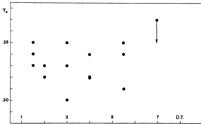
Fig. 4. Plot of Y -values [from Eq. (13)] vs. the HB Dickens type. The arrow indicates a lower limit for 47 Tuc still compatible with the data (see text for discussion)
