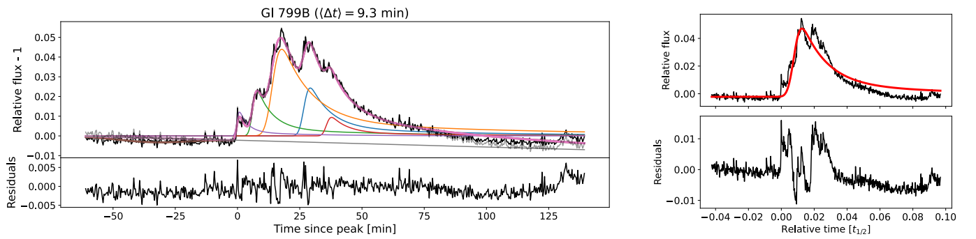
Fig. 19. QPP candidate on Gl 799 B. Left: the mean time between consecutive peaks is reported in the title. This QPP candidate is probably the same one reported by Howard & MacGregor (2022) ; their Fig. 7, left panel), for which we recover a similar period to their \approx 7.5 min. The individual flare components that were identified by our algorithm are drawn with different colours, and the total model is represented with a thick line. Right: on the top sub-panel, fit to the flare profile with a single-peak model. On the lower sub-panel, the residuals used to estimate the oscillation amplitude.
