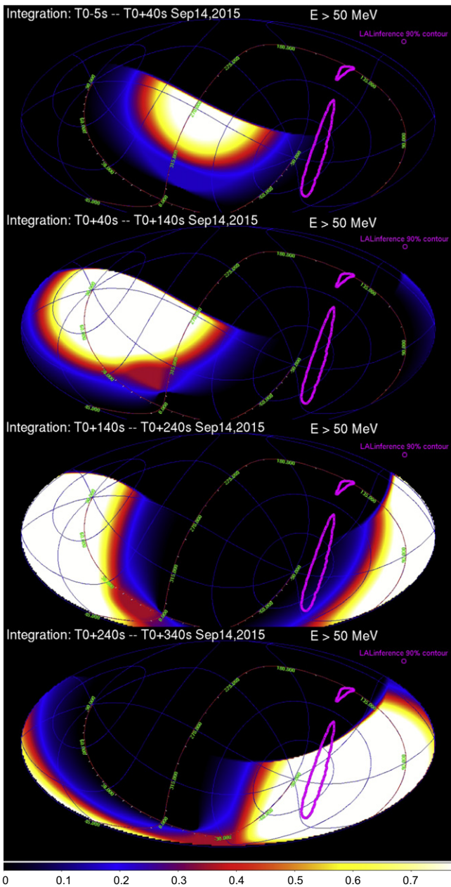
Figure 1. Hammer-Aitoff projection in Galactic coordinates of the AGILE satellite rotation and a typical sequence of E > 50 MeV gamma-ray exposure maps (in \text{cm}^2 \text{s sr} , using a 0.5^\circ pixel size) as the satellite rotates in spinning mode, scanning 80% of the sky in about 7 minutes. The AGILE -GRID FOV radius is assumed to be 70^\circ . In this case, the Earth is occulting the FOV in the Northern Galactic hemisphere. The exclusion region for the albedo photons is 80^\circ from the Earth center. This sequence applies to the satellite rotation that includes the prompt event time of GW150914 (localization region marked by the purple contour, LALInference 90% contour level, A16e).
