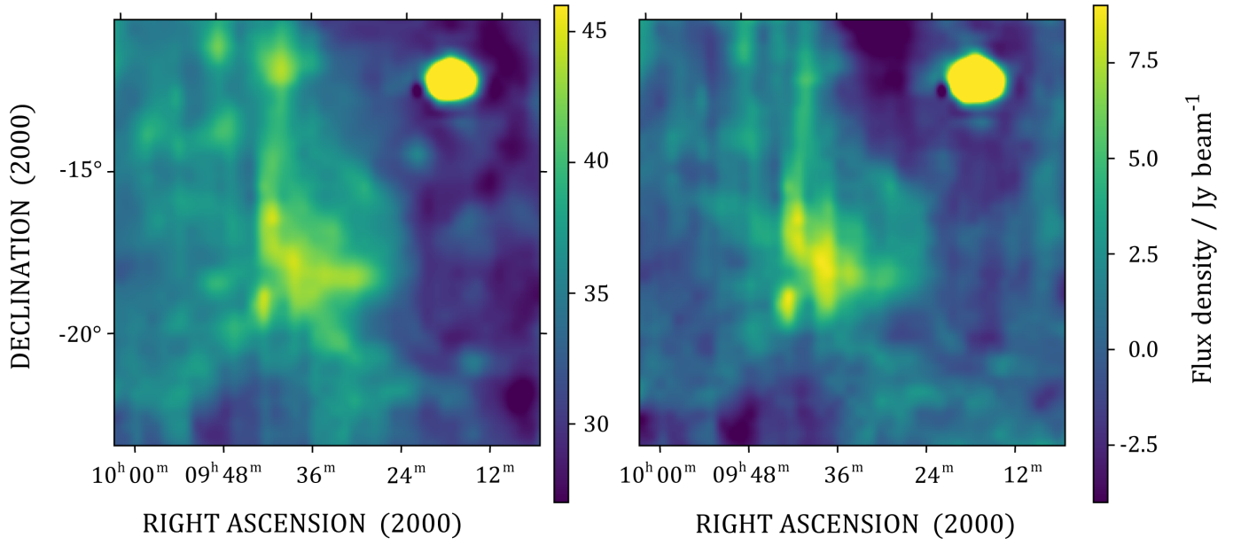
Fig. 7. 100 deg 2 of the region surrounding the Hoinga SNR as seen at 408 MHz by the survey by Haslam et al. (1982), after conversion from K to Jy beam -1 . Left panel: original image, and right panel: image after source-subtraction and backgrounding, discussed in Sect. 3.2. Hoinga is visible as an ellipse in the centre of the image, while Galactic cirrus and scan line artefacts from the Parkes observing strategy dominate the surroundings. The bright source in the northwest is Hydra A, and subtraction of this source has not been performed.
