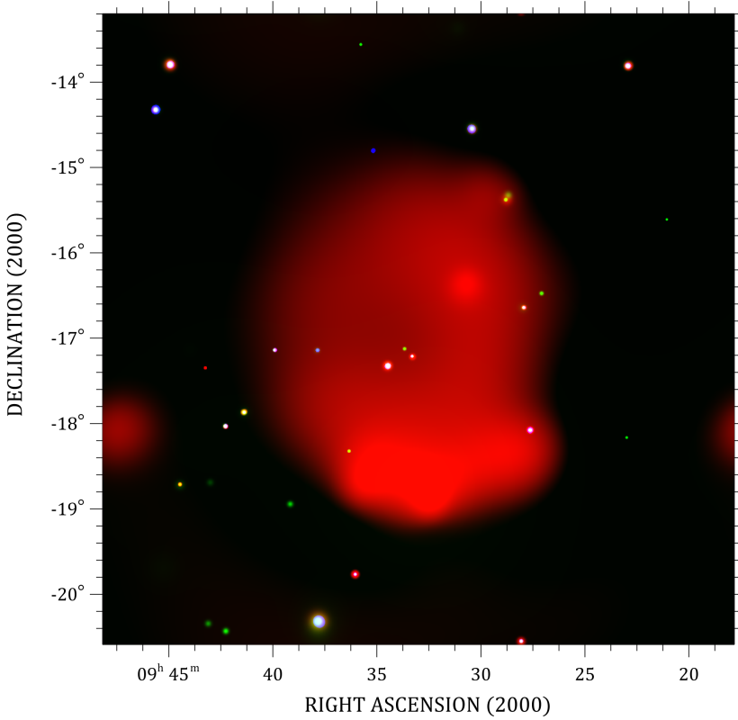
Fig. 2. Hoinga SNR as seen in the eROSITA all-sky survey eRASS1. Photons to produce this 7.5 \times 7.5 image were colour coded according to their energy (red for energies 0.2–0.7 keV, green for 0.7–1.2 keV, blue for 1.2–2.4 keV). An adaptive kernel smoothing algorithm was applied to the images in each energy band.
