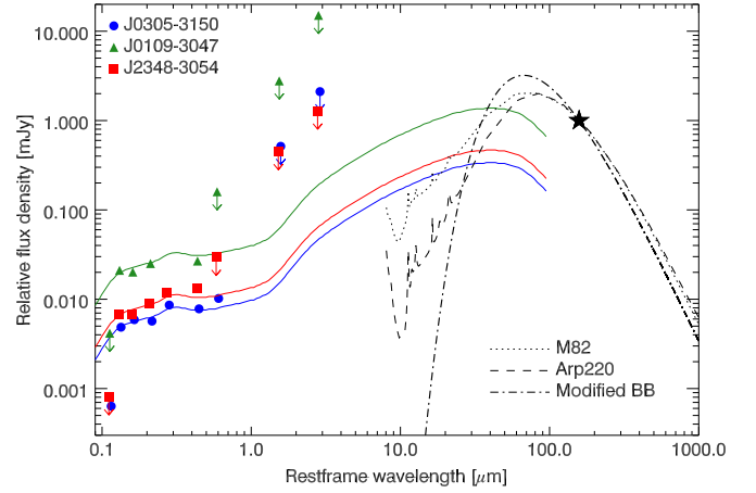
Figure 3. Spectral energy distributions (SEDs) of the three VIKING quasars, normalized to 1 \text{ mJy} at 158 \mu\text{m} in the rest frame. The rest-frame UV to near-infrared data points are taken from Venemans et al. (2013) and from the Wide-field Infrared Survey Explorer (WISE, Wright et al. 2010). We fitted the quasar template of Richards et al. (2006) to the short-wavelength ( \lambda_{\text{obs}} < 30 \mu\text{m} ) data points of each quasar. The three models used in this paper to model the far-infrared emission are shown by the dotted line (M82 template), dashed line (Arp 220 template), and dotted–dashed line (modified blackbody).
