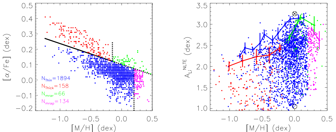
Fig. 1. Left: [\alpha/\text{Fe}] vs. [M/H] patterns for the thin-disk (blue), canonical thick-disk (red), metal-rich [\alpha/\text{Fe}] -rich stars (green), and super-metal-rich solar- \alpha stars (magenta). The black lines show how we identified these four MW populations. Right: AMBRE NLTE lithium abundance vs. metallicity for the corresponding four populations using the same color-code as in the left panel. For a given population, we plot the maximum lithium abundance using the same method as Guiglion et al. (2016). The meteoric lithium abundance, which is not affected by from stellar evolution, is also shown ( \otimes ).
