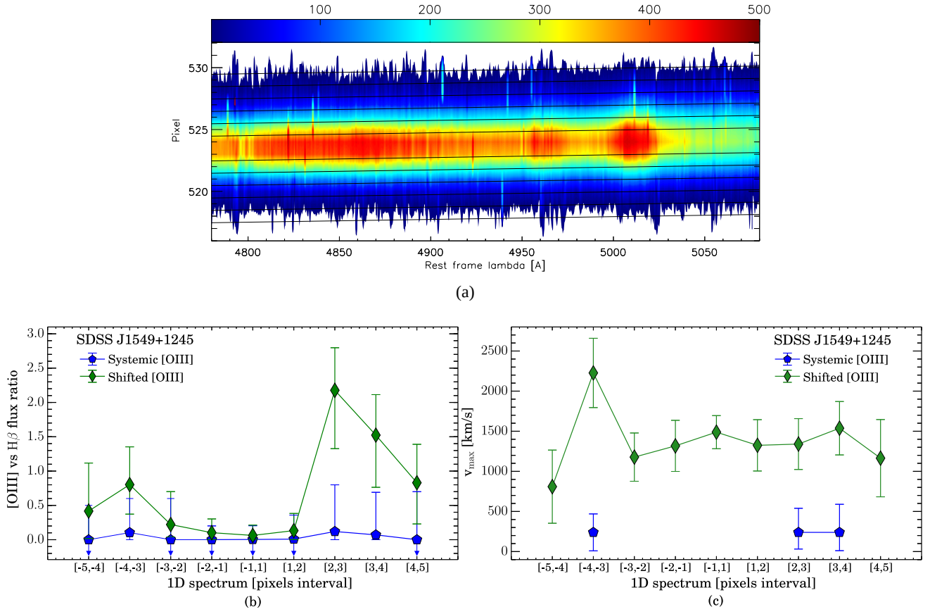
Fig. 11. Same as Fig. 8 but for J1549+1245 (1 pixel \sim 2.1 kpc at the redshift of this source).
