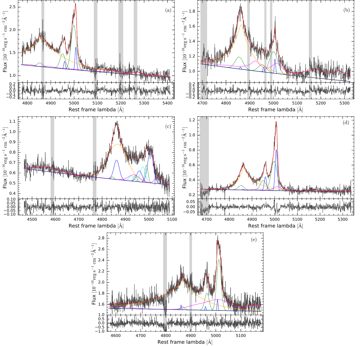
Fig. 1. LUCI1 spectra of the five analysed WISSH quasars. The red lines show the resulting best-fits for (a) SDSS J0745+4734, (b) J0900+4215, (c) J1201+1206, (d) J1326–0005 and (e) J1549+1245. Blue and green curves respectively refer to the NLR core and broad emission of both [OIII] and H \beta . BLR H \beta emission is indicated in orange and FeII emission is indicated in magenta. The cyan curve in panel (c) represents the additional components necessary to account for the plateau-like emission feature between 4900–5000 Å in J1201+1206. Grey bands indicate the regions excluded from the fit due to presence of telluric features.
