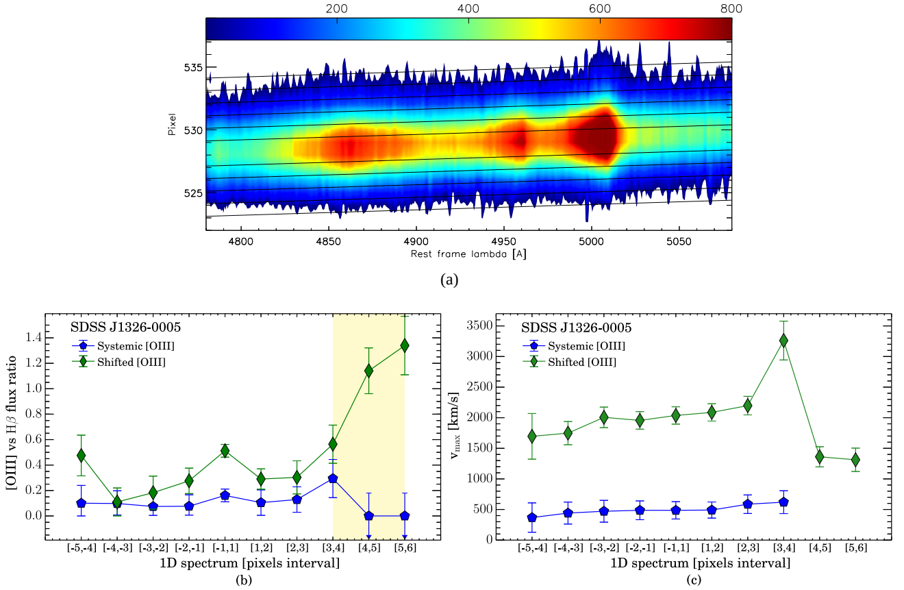
Fig. 10. Same as Fig. 8 but for J1326–0005 (1 pixel \sim 1.9 kpc at the redshift of this source).
