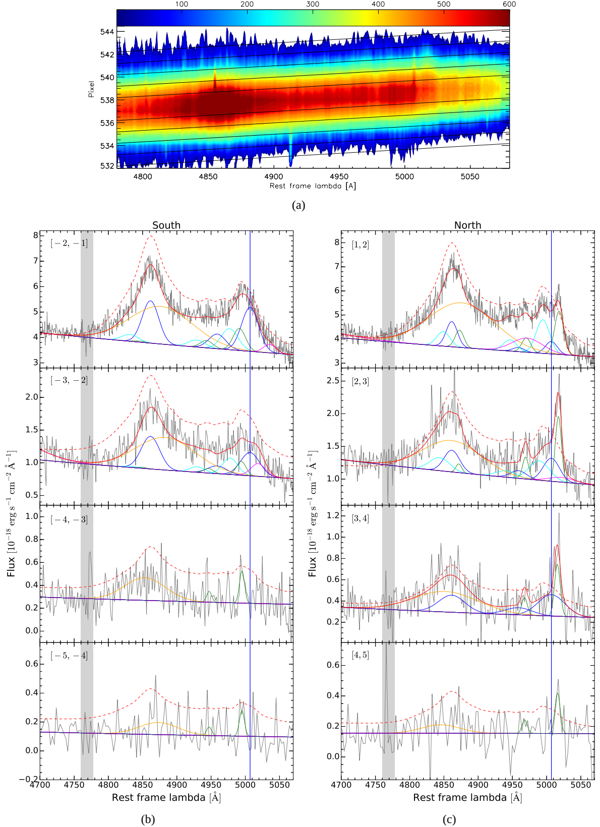
Fig. 2. (a) 2D LUCI1 spectrum of J1201+1206. Blue to red colors indicate increasing counts. Since the LUCI1 spectra have been acquired with PA = 0 deg, top and bottom correspond to North and South directions, respectively. The black solid lines indicate the apertures used for extracting the off-nuclear spectra. Panels (b) and (c) show the "off-nuclear" spectra of J1201+1206 extracted in 1 pixel ( \sim 1.9 kpc) width regions at increasing distances from the peak of the spatial profile of the continuum emission. Negative(positive) pixel values correspond to South(North) direction. In both panels, the offset increases from top to bottom, as indicated by the corresponding pixels interval. Spectral components are indicated as in Fig. 1c. The vertical line corresponds to \lambda = 5007 \text{ \AA} , while the dashed red line indicates the best-fit model of the central spectrum extracted from the two-pixels region [-1,1] , plotted with arbitrary normalization for display purpose only. Grey bands indicate the regions excluded from the fit due to the presence of telluric features.
