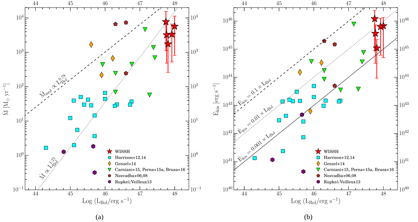
Fig. 7. Mass rate (a) and kinetic power (b) of the ionised outflows as a function of L_{\text{Bol}} . Values obtained for the WISSH quasars (red stars) are compared with other samples from literature (i.e. Harrison et al. 2012, 2014; Genzel et al. 2014; Carniani et al. 2015; Perna et al. 2015a; Brusa et al. 2016; Nesvadba et al. 2006, 2008; Rupke & Veilleux 2013). Error bars are calculated as described in Sect. 6.2. In panel (a) the dotted line corresponds to the best-fit relation \dot{M} \propto L_{\text{Bol}}^{1.21} derived for ionised outflows and the dashed line to the \dot{M} \propto L_{\text{Bol}}^{0.78} best-fit relation to molecular outflows (see Fiore et al. 2016, A&A submitted, for a complete discussion). In panel (b) dashed, dotted and solid lines represent an outflow kinetic power that is 10%, 1% and 0.1% of the AGN luminosity, respectively.
