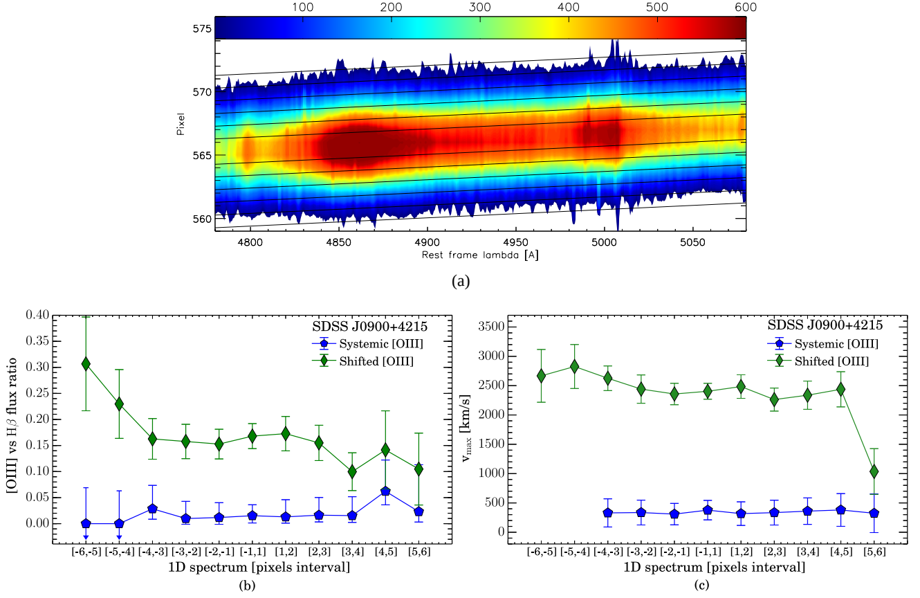
Fig. 9. Same as Fig. 8 but for J0900+4215 (1 pixel \sim 1.9 kpc at the redshift of this source).
