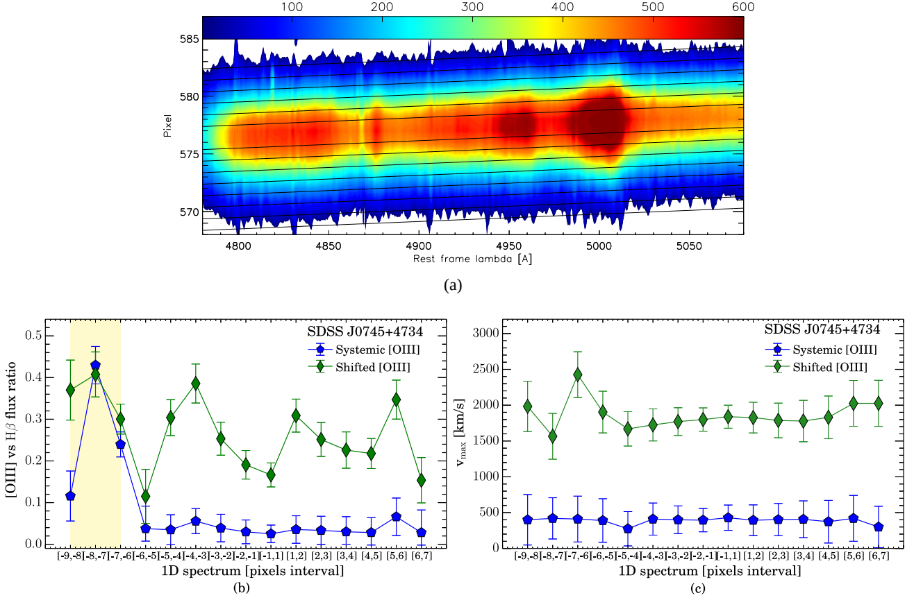
Fig. 8. (a) 2D LUCI1 spectrum of J0745+4734. Blue to red colours indicate increasing counts. Top and bottom correspond to North and South direction, respectively. The black solid lines indicate the apertures used for extracting the off-nuclear spectra. (b) The integrated flux ratio of the shifted and systemic [OIII] components with respect to the BLR H\beta emission line detected in the "off-nuclear" spectra of J0745+4734 extracted from different apertures. Negative(positive) pixel values correspond to South(North) direction (1 pixel \sim 1.9 kpc at the redshift of J0745+4734). The yellow band highlights the presence of extended [OIII] emission. (c) Maximum velocity of the shifted and systemic [OIII] components detected in the "off-nuclear" spectra of J0745+4734.
