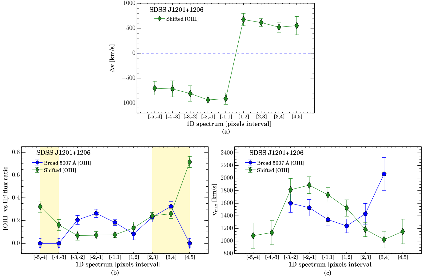
Fig. 3. (a) Velocity shift of the blue/redshifted [OIII] component with respect to 5007 Å (dashed line), detected in the "off-nuclear" spectra of J1201+1206 extracted from different apertures. Negative(positive) pixel values correspond to South(North) direction (1 pixel \sim 1.9 kpc at the redshift of J1201+1206). (b) The ratio between the integrated flux of the two [OIII] components (i.e. the broad one at 5007 Å and the blue/redshifted one) and the BLR H \beta emission for the "off-nuclear" spectra of J1201+1206. The yellow bands highlight the presence of extended [OIII] emission. (c) Maximum velocity of the broad [OIII] component at 5007 Å and the blue/redshifted [OIII] component detected in the "off-nuclear" spectra of J1201+1206.
