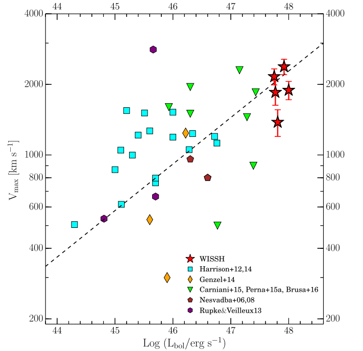
Fig. 6. Maximum velocity of the outflow versus the AGN L_{\text{Bol}} of the WISSH quasars compared with other samples from literature (i.e. Harrison et al. 2012, 2014; Genzel et al. 2014; Carniani et al. 2015; Perna et al. 2015a; Brusa et al. 2016; Nesvadba et al. 2006, 2008; Rupke & Veilleux 2013). The dashed line represents the relation L_{\text{Bol}} \propto v_{\text{max}}^5 (with arbitrary normalization) expected for energy conserving winds (see Costa et al. 2014).
