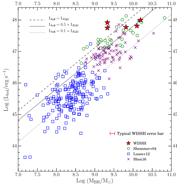
Fig. 4. Bolometric luminosity as a function of the H\beta -based SMBH mass ( M_{\text{BH}}^{H\beta} ) for different AGN samples. The WISSH quasars are indicated by red stars, while squares refer to X-ray selected Type 1 AGN from Lusso et al. (2012). Circles and crosses indicate the optically selected z \sim 2 - 3 quasars from Shemmer et al. (2004) and Shen (2016), respectively. The lines correspond to L_{\text{Bol}}/L_{\text{Edd}} = 1 (dashed), L_{\text{Bol}}/L_{\text{Edd}} = 0.5 (solid) and L_{\text{Bol}}/L_{\text{Edd}} = 0.1 (dotted).
