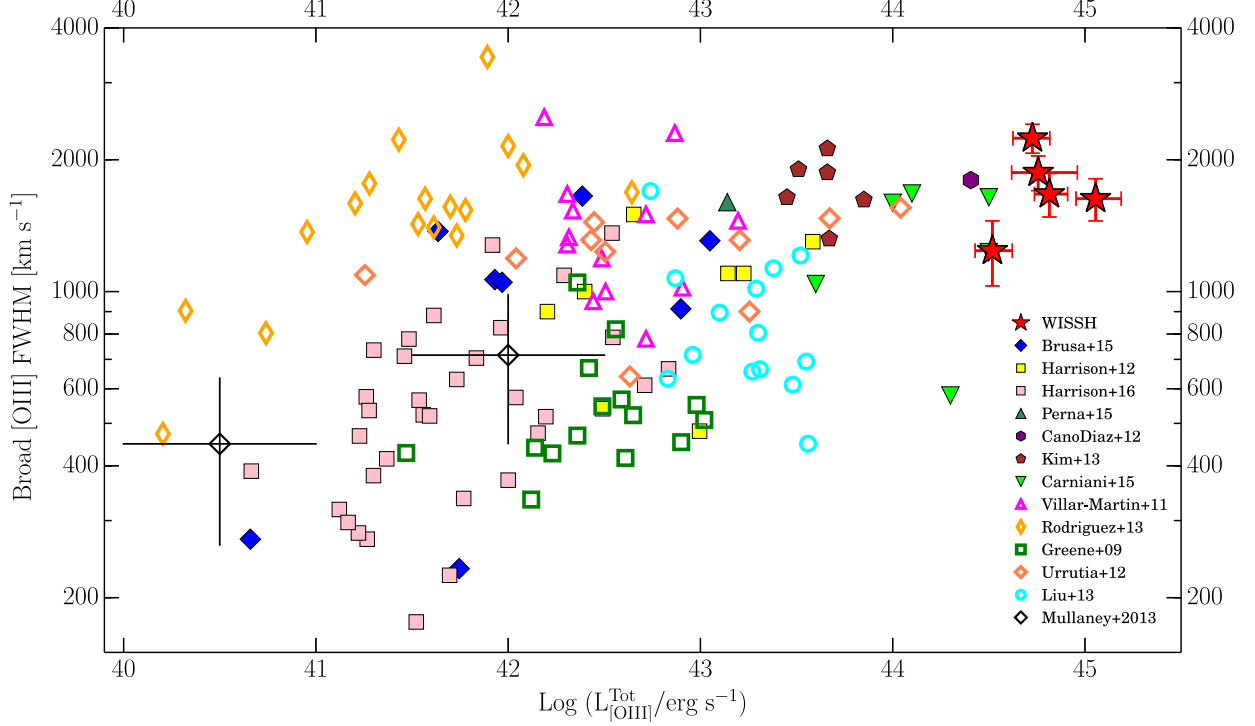
Fig. 5. \text{FWHM}_{[\text{OIII}]^{\text{broad}}} as a function of the total observed [\text{OIII}]\lambda 5007 \text{ \AA} luminosity ( L_{[\text{OIII}]}^{\text{Tot}} ) for different AGN samples. WISSH quasars (red stars) are compared with other samples of Type 1 and Type 2 AGN at low ( z < 1 , empty symbols) and high ( z > 1 , filled symbols) redshift. We plot the values obtained for: a sample of obscured (Greene et al. 2009; Brusa et al. 2015; Perna et al. 2015a), red (Urrutia et al. 2012), Type 2 (Villar-Martín et al. 2011; Liu et al. 2013), luminous z \sim 2.4 (Cano-Díaz et al. 2012; Carniani et al. 2015), KASHz at z \sim 1.1 - 1.7 (Harrison et al. 2016) and radio quasars (Kim et al. 2013), in addition to the local and high- z ULIRGs by Rodríguez Zaurín et al. (2013) and Harrison et al. (2012), respectively. The average values in two L_{[\text{OIII}]}^{\text{Tot}} bins for optically-selected Type 2 AGN in Mullaney et al. (2013) are also shown.
