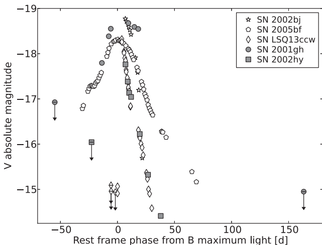
Figure 6. V-band absolute light curve for SN 2001gh compared with those of the peculiar SNe Ib 2002bj, 2002hy ( R -band absolute magnitudes), 2005bf and the Type Ibn LSQ13ccw (sloan r -band converted into Johnson-Cousins R -band). The magnitudes of SNe 2001gh and 2002hy have been corrected for the reddening values adopted in this paper, E(B - V) of 0.016 and 0.141 mag, respectively, and accounting for their adopted distance moduli of 39.33 \pm 0.10 and 33.61 \pm 0.20 mag. Distances and extinction estimates for all other SNe have been taken from the literature. Ages are relative to the rest-frame B maximum light.
