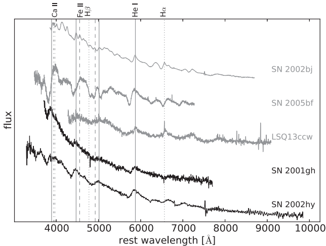
Figure 5. Comparison of the early optical spectrum of SN 2001gh with those of the peculiar Type Ib SNe 2002bj, 2002hy, 2005bf and the Ibn LSQ13ccw at epochs between -5 and 11 d from the maximum light. Vertical solid lines mark the rest-frame position of the main He I features, while the dotted, dashed, and dot-dashed lines give the rest wavelength positions of the main H and Fe II features, along with those of the Ca II H&K doublet. All spectra have been reddening and redshift corrected assuming the values adopted in this work and from the literature.
