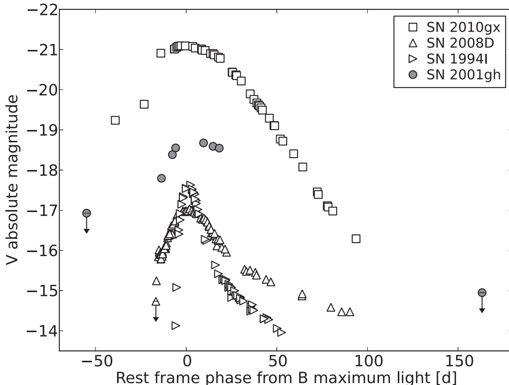
Figure 4. V -band absolute light curve for SN 2001gh compared with those of SNe Ib 2008D, the superluminous 2010gx ( B -band absolute magnitude) and the Ic 1994I. The magnitudes of SNe 2001gh have been corrected for the assumed reddening, E(B - V) of 0.016 mag, and the adopted distance modulus of 39.33 \pm 0.10 mag. Distances and extinction estimates for all other SNe have been adopted from the literature. Ages are relative to B maximum light in the rest frame.
