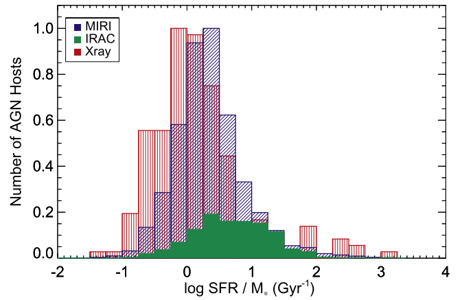
Figure 7. We show the host galaxy property \text{sSFR} = \text{SFR}/M_* of CANDELS galaxies identified as likely AGNs according to a hard X-ray cut (red histogram; L_{2\text{--}10 \text{ keV}} \geq 10^{43} \text{ erg s}^{-1} ) and MIRI color selection (blue histogram). We have normalized each distribution to allow easier comparison, although the MIRI distribution has 20\times more sources. The MIRI selection is sensitive to host galaxies with higher sSFRs. We illustrate which of the MIRI-selected AGN hosts would also be selected with the Donley et al. (2012) IRAC selection criteria. Due to the sensitivity and coverage of the MIRI filters, we will be able to select larger samples of AGN hosts than was possible with IRAC selection.
