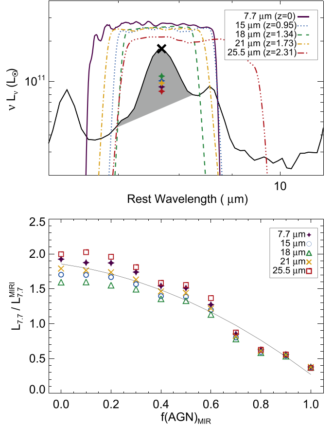
Figure 3. Top panel: we demonstrate, using the MIR0.0 template from Kirkpatrick et al. (2015), how much of the 7.7 \mu\text{m} feature each MIRI filter covers at the redshifts where the central wavelength of each filter is 7.7 \mu\text{m} (listed in the legend). The gray shaded region indicates which part of the spectrum is integrated to calculate L_{7.7} (black cross), while the filled stars show the photometry (in units of \nu L_\nu ) measured through each of the MIRI filters. The photometry is lower because it includes more of the spectrum at lower luminosity. Bottom panel: ratio of the MIRI photometry ( L_{\text{MIRI}} ) measured through different MIRI filters depending on redshift to the intrinsic L_{7.7} of the PAH feature. The lower fractions with increasing f(\text{AGN})_{\text{MIR}} are due to an increased warm dust continuum due to heating by an AGN. If L_{7.7} is going to be used to calculate SFRs, corrections need to be made for an AGN contribution. The black line is the empirical relationship between L_{7.7}/L_{\text{MIRI}} and f(\text{AGN})_{\text{MIR}} .
