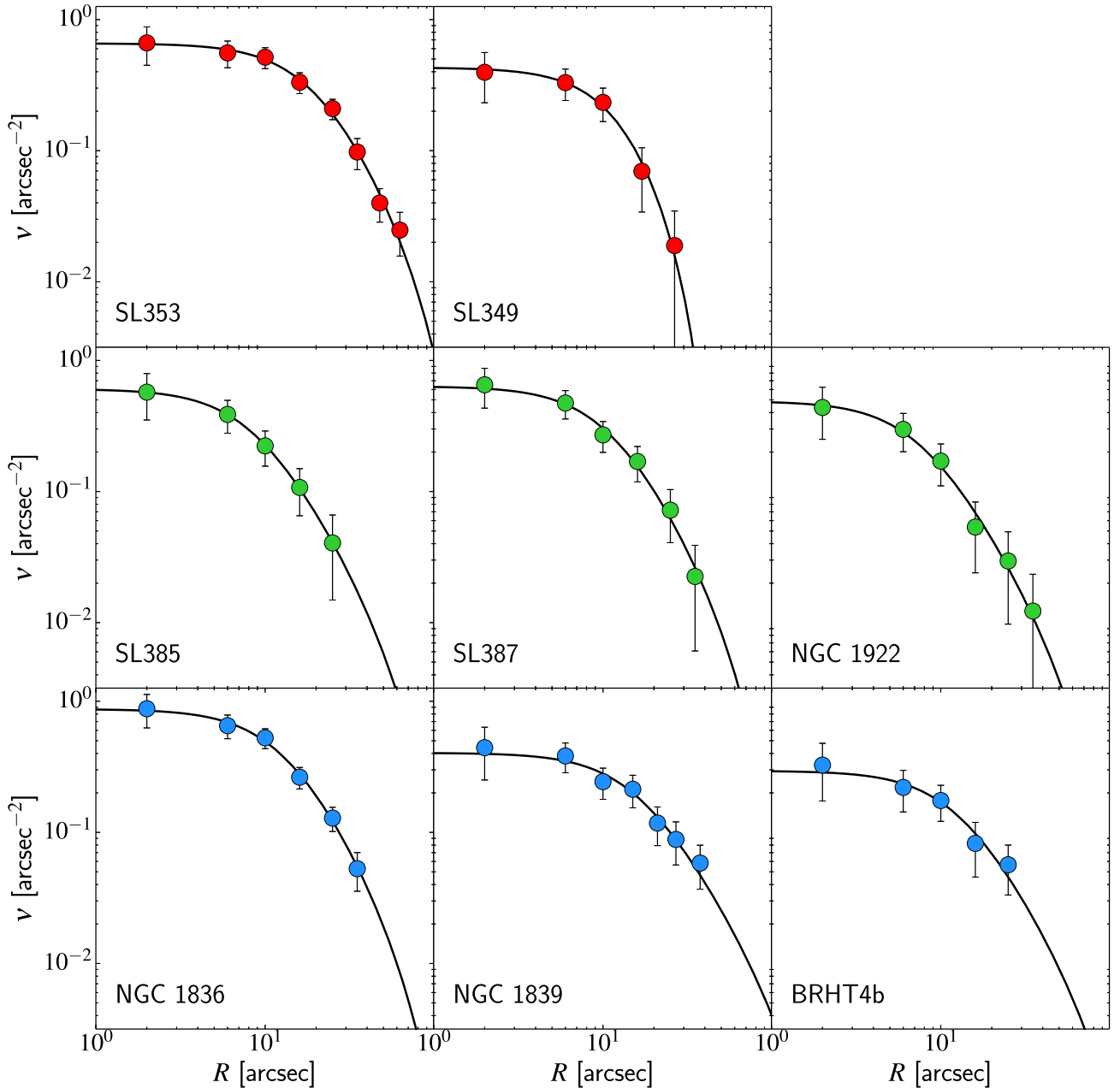
Figure 7. Number density profiles of the clusters in our sample, as indicated by the labels in the panels. Solid lines correspond to the best-fitting King (1996) model fits, and the data are indicated with circles. Each row corresponds to a different group of clusters, identified also by the different colours of the points in the panels. For each data point, vertical error bars are shown. The vertical and horizontal axes span the same range in every panel, to allow a more direct comparison among the clusters.
