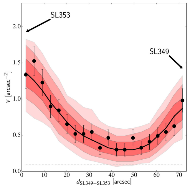
Figure 10. Black points with vertical error bars indicate the number density measured from the data along the line connecting clusters SL353 and SL349 on the plane of the sky. The thick solid line represents the median of the distribution of the number density calculated from the 1000 random realizations of the simulated observations in the same sky region; the shaded areas correspond to 1\sigma , 2\sigma and 3\sigma from the median. The dashed line indicates the uniform background density.
