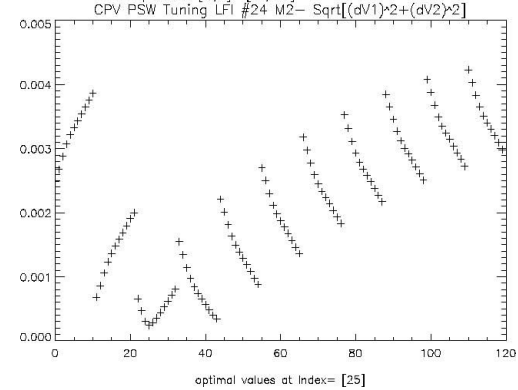
CPV PSW Tuning LFI #24 M2- \text{Sqrt}[(dV1)^2 + (dV2)^2]
