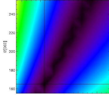
CPV PSW Tuning LFI #27 M2- \text{Sqrt}[(dV1)^2 + (dV2)^2]
