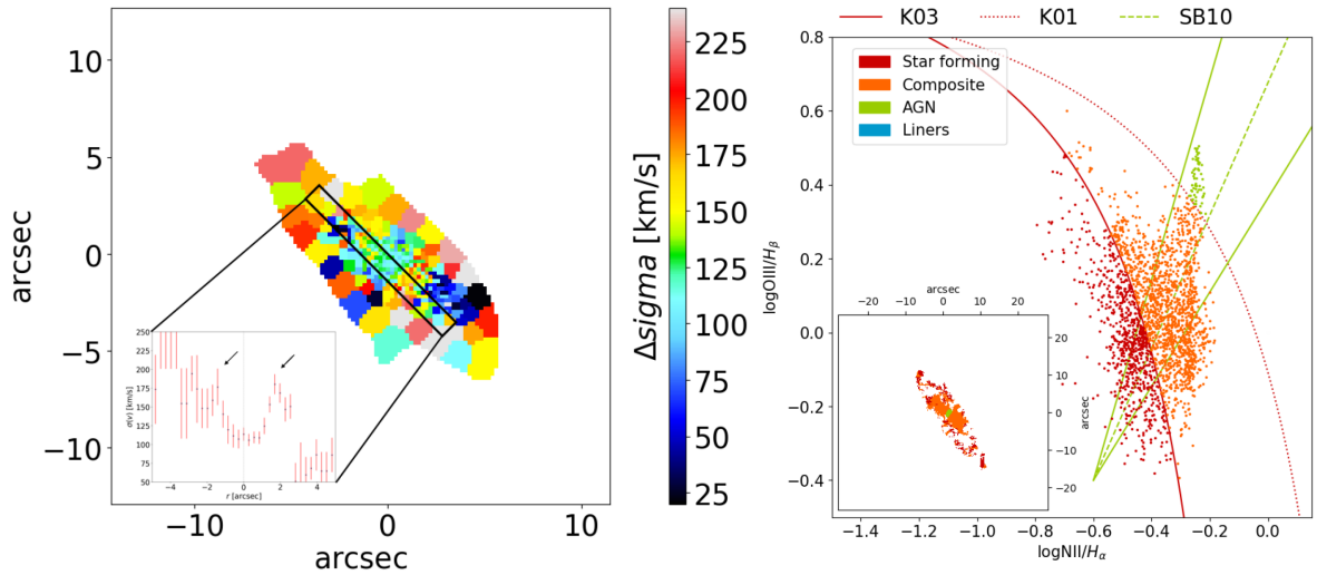
Figure 9. P4946. Left: Stellar velocity dispersion map. The inset shows the stellar velocity dispersion profile in the inner region. The two arrows show the double peak, indication of the presence of two counter-rotating stellar components. Right: BPT line-ratio diagram for [O\text{III}]\lambda 5007/H\beta versus [N\text{II}]\lambda 6583/H\alpha . Lines are from Kauffmann et al. (2003, K03), Kewley et al. (2001, K01), and Sharp & Bland-Hawthorn (2010, SB10) to separate Star-forming, composite, AGN, and LINERS. In the inset, the BPT line-ratio map is shown. Only spaxels with an S/N > 3 in all the emission lines involved are shown.
