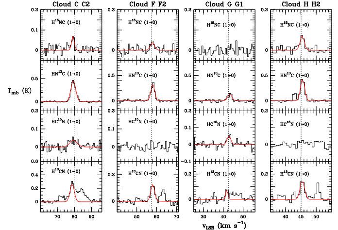
Fig. 1. From left to right, top to bottom panels: emission lines of \text{H}^{15}\text{NC} , \text{HN}^{13}\text{C} , \text{HC}^{15}\text{N} , and hyperfine transitions of \text{H}^{13}\text{CN} observed with IRAM 30 m towards IRDCs C, F, G, and H. Red lines indicate the best Gaussian fit to the lines. The hyperfine components of \text{H}^{13}\text{CN} were initially fitted but given the bad results of the fit; in a second step only the main F = 2 \rightarrow 1 component of \text{H}^{13}\text{CN} was fitted using a single-Gaussian component profile (see red line in bottom panels and Sect. 3.1 for details). See also Figs. A.1–A.4 for all spectra taken.
