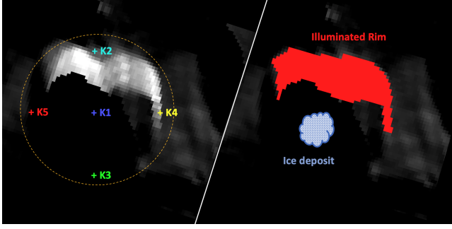
Figure 9. Simulated illumination conditions, or \cos(i) , occurring on Kandinsky crater at TA=200^\circ (left panel). The area of the sun illuminated rim (in red, departing from point K2) and the location of the putative water ice deposit (blue dots, corresponding to location K1) on the unilluminated crater floor are shown on the right panel.
