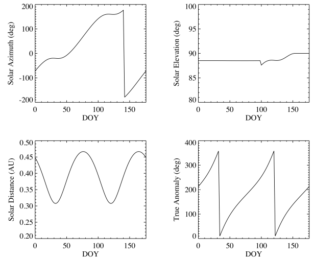
Figure 5. Average illumination conditions above Prokofiev and Kandinsky craters and Mercury’s orbital parameters for one hermean solar day. The illumination rendering shown in the previous Fig. 4 at TA=200^\circ corresponds to DOY=84.
