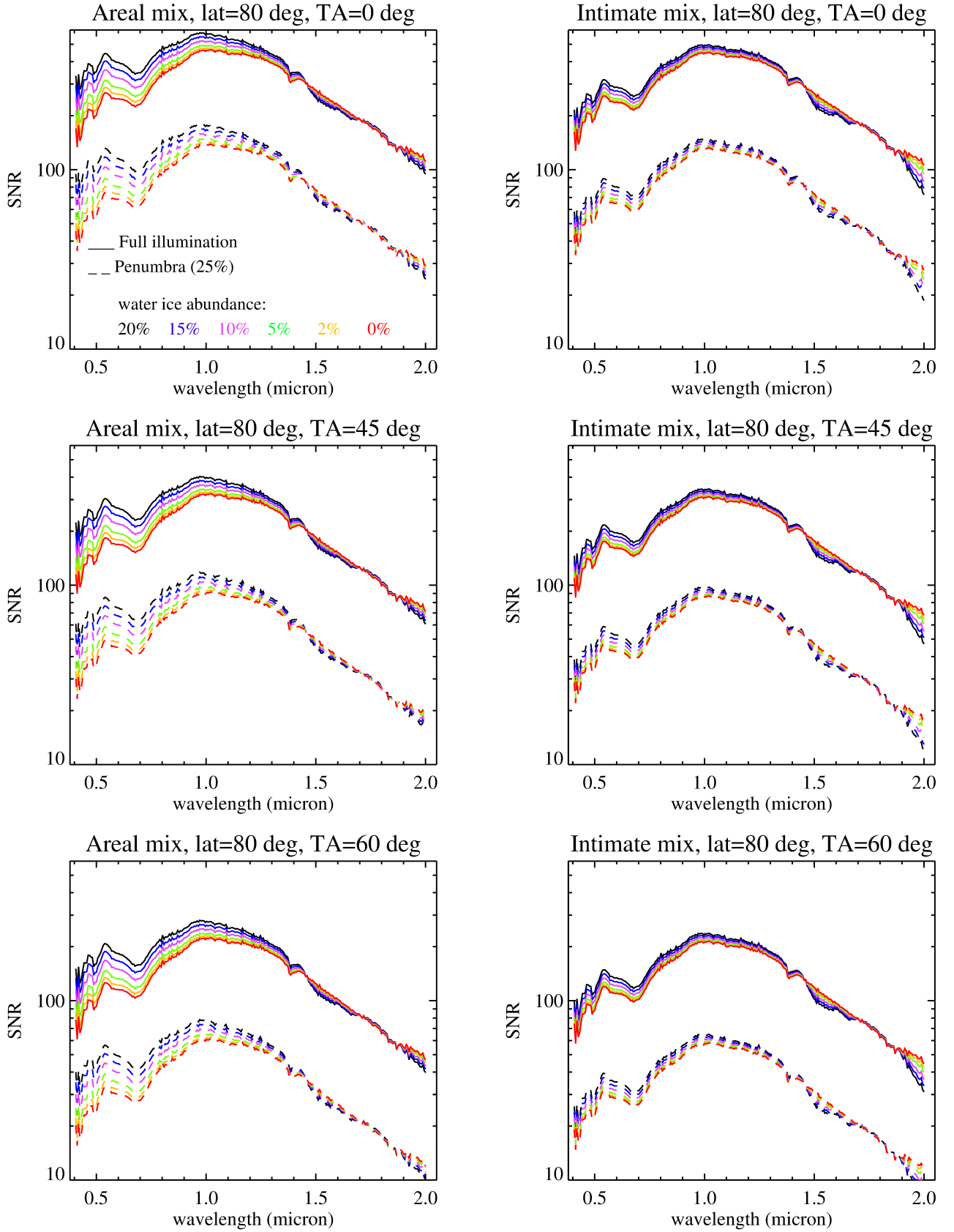
Figure 11. VIHI theoretical SNR in the direct illumination (solid lines) and in the penumbra (efficiency of 25% of the direct illumination, dashed lines) for AMT-water ice mixtures from 100:0% to 80:20% abundances, 100\ \mu\text{m} grain diameter, computed at latitude \pm 80^\circ for perihelion orbital arc (from top to bottom TA = 0^\circ , 45^\circ , 60^\circ ). Areal and intimate mixing cases are shown on the left and right columns, respectively. Simulations are performed with i=80^\circ and e=0^\circ .
