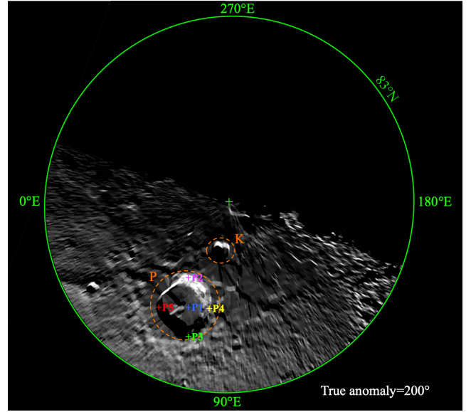
Figure 4. Illumination rendering on the north polar regions for TA=200^\circ . The full simulation covering an entire solar day is available as a supplemental online material. Locations P1-5 are shown for Prokofiev (similar positions for Kandinsky are shown in Fig. 9) at larger scale.
