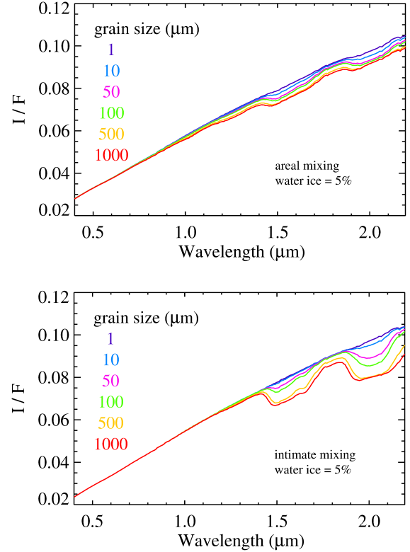
Figure 8. Simulated I/F spectra of AMT-water ice mixture with relative abundance 95:5% (areal mix on the top panel, intimate mixing on bottom panel) for 1 to 1000 \mu\text{m} water ice grains diameters. Incidence angle is 80^\circ , emission angle is 0^\circ .
