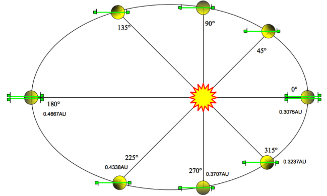
Figure 1. Schematics of Mercury and BepiColombo spacecraft orbits (green lines) seen from Sun north pole. At TA=0° Mercury is at perihelion and the spacecraft is at apoherm on the day side. At TA=180° Mercury is at aphelion and the spacecraft is at periherm.
