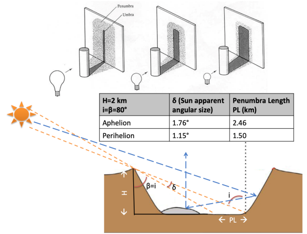
Figure 2. Top panel: umbra and penumbra cast by an extended source at finite distance. Centre table: penumbra length values for a crater's rim of height H=2 km placed at latitude 80^\circ at perihelion and aphelion. Bottom panel: penumbra geometry case (orange lines) and indirect illumination case of an ice deposit within PSR by the illuminated rim of the crater (blue lines, see discussion in Section 5).
