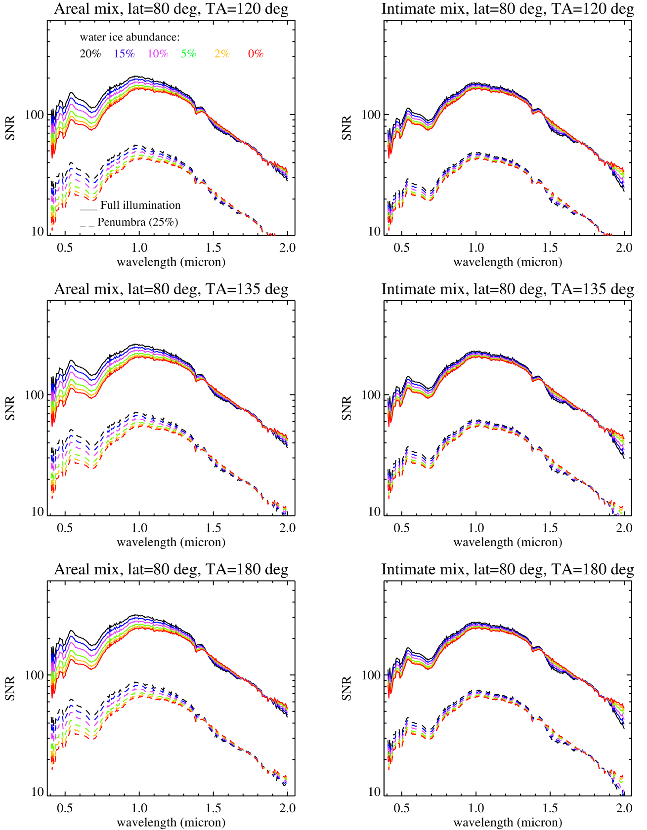
Figure 12. VIHI theoretical SNR in the direct illumination (solid lines) and in the penumbra (efficiency of 25% of the direct illumination, dashed lines) for AMT-water ice mixtures from 100:0% to 80:20% abundances, 100\ \mu\text{m} grain diameter, computed at latitude \pm 80^\circ for aphelion orbital arc (from top to bottom \text{TA}=120^\circ, 135^\circ, 180^\circ ). Areal and intimate mixing cases are shown on the left and right columns, respectively. Simulations are performed with i=80^\circ and e=0^\circ .
