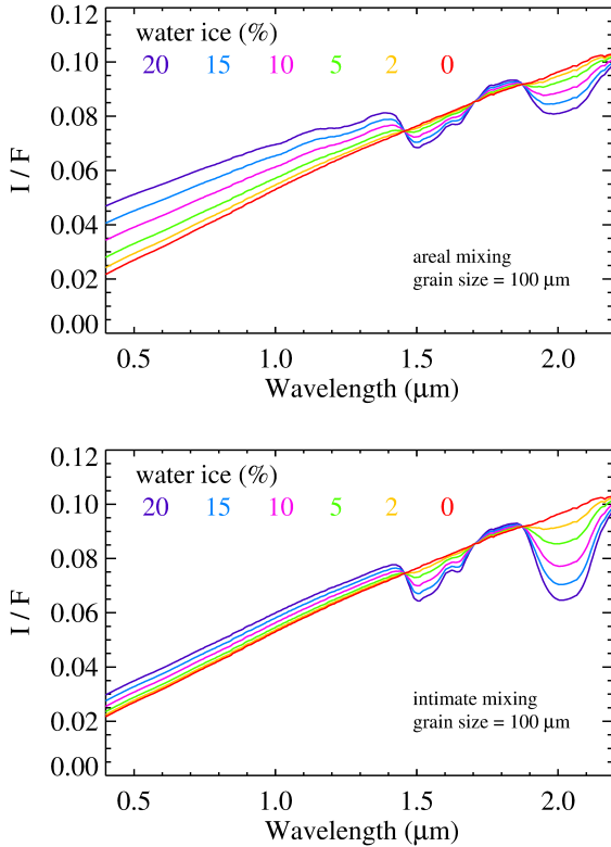
Figure 7. Simulated I/F spectra of AMT-water ice mixtures with relative abundances from 100:0% to 80:20% (areal mixture on top panel, intimate mixture on bottom) for 100 \mu\text{m} water ice grains diameter. Incidence angle is 80^\circ , emission angle is 0^\circ .
