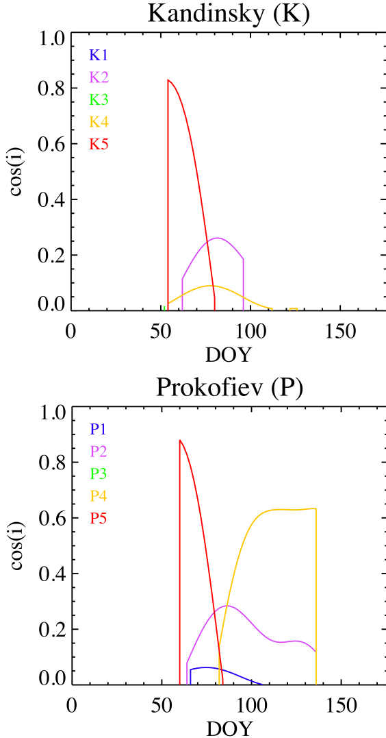
Figure 6. Illumination conditions above center and rims of Kandinsky (top panel) and Prokofiev (bottom panel) craters locations #1-5 for one hermean solar day.
