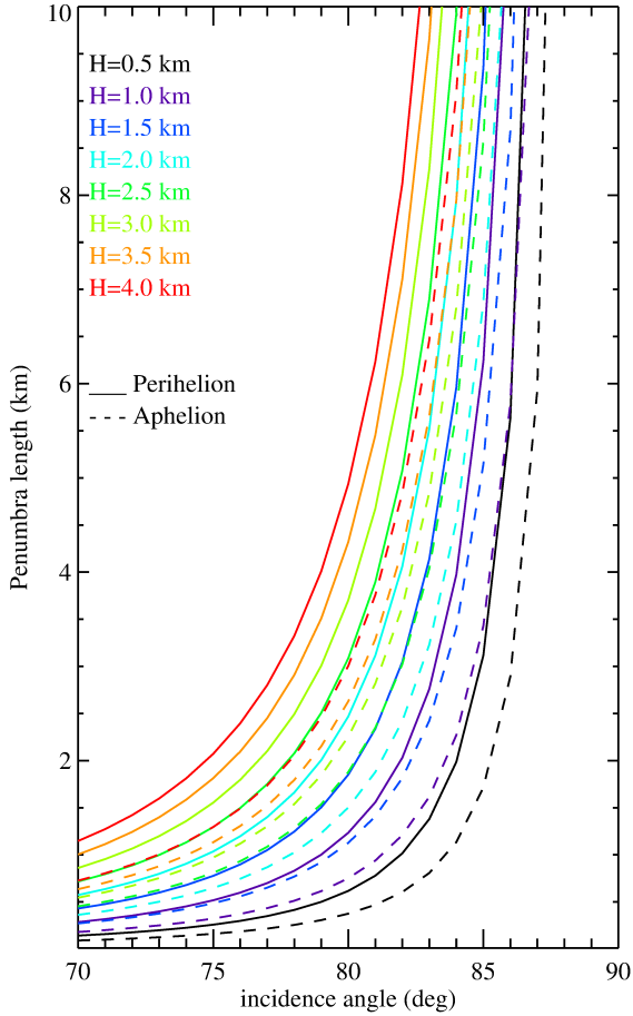
Figure 3. Penumbra length cast by the Sun at at perihelion (solid line) and aphelion (dashed line) from a crater’s rim of variable height between 0.5 to 4 km placed at latitude 80°.
