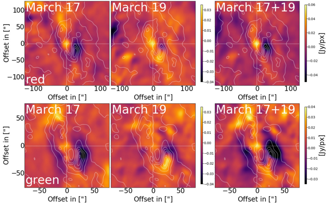
Figure 5. Red and green integrated residual maps for the observations on March 17 (left column), March 19 (middle column), and the two nights combined (right column).
