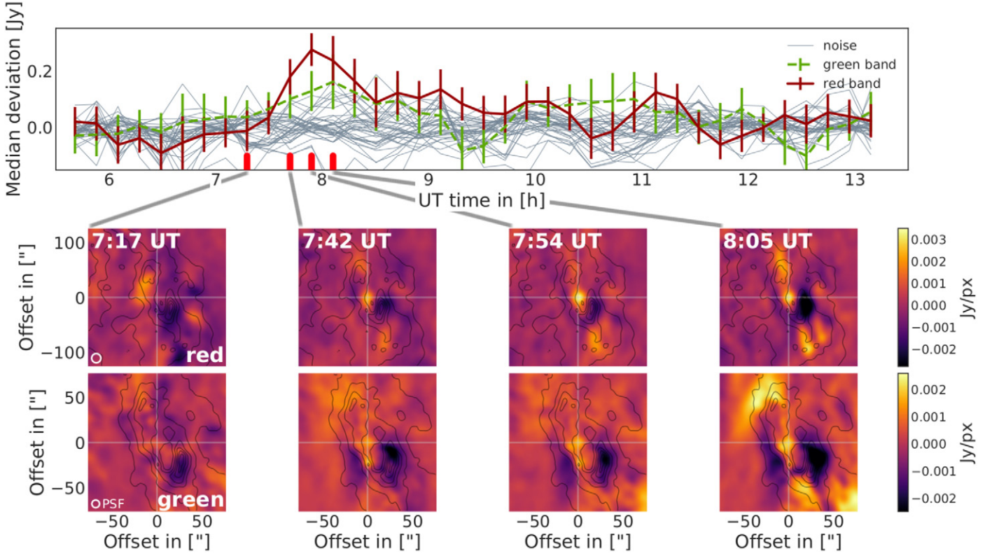
Figure 2. The FIR variability on March 17: the upper panel shows the light curves of the red and green bands, as well as the reference light curves of the red band. Below are the residual maps, which show the variable flux of Sgr A*. The contour lines are intensity profiles of the respective median images. A point source is visible at the position of Sgr A*.
