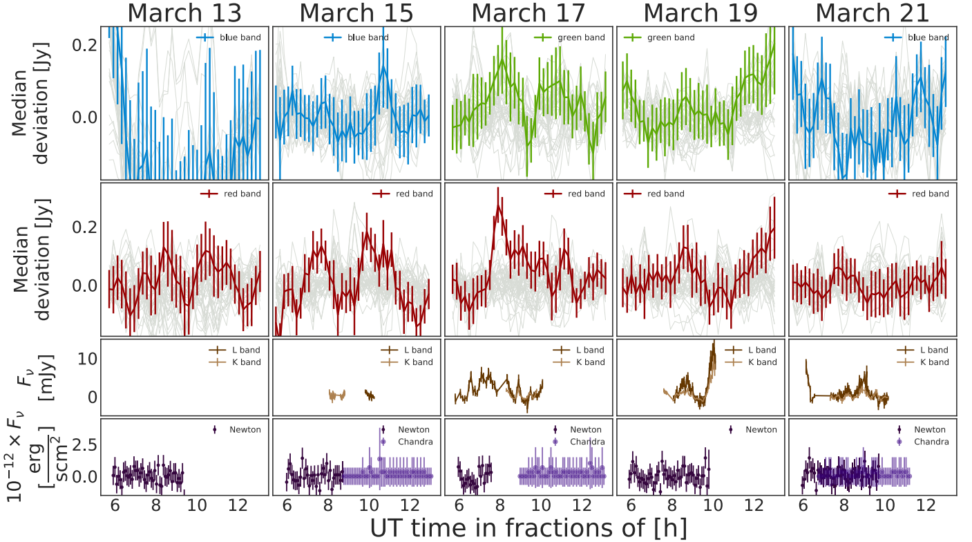
Figure 14. All available light curves. The top two rows show the FIR light curves obtained with Herschel /PACS. The top row are the light curves of the blue and green bands (color-coded). The second row is the light curve of the red band. The gray light curves are those of the reference positions (see Section 2.3.1). The lower two rows show the parallel NIR ( L' and K bands) and X-ray observations from NACO , XMM-Newton , and Chandra , where available.
