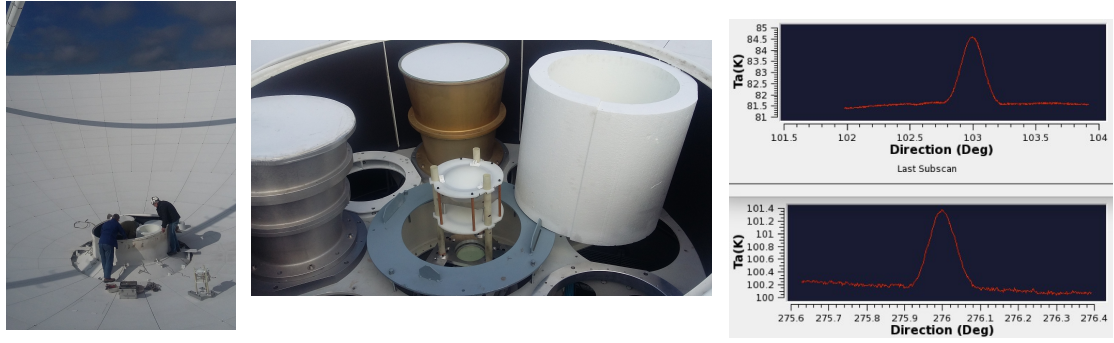
Fig. 4 Left panel. Mounting of the collimator at the Cassegrain focus of the Medicina antenna. Middle panel. The collimator mounted on the dewar of the K-band receiver. Right panel. Example of almost identical antenna beam-patterns obtained during an azimuth scan without (top) and with (bottom) the collimator, but with no TP applied. The raw horizontal scale is not corrected for the different elevations. The vertical scale is raw antenna temperature.
