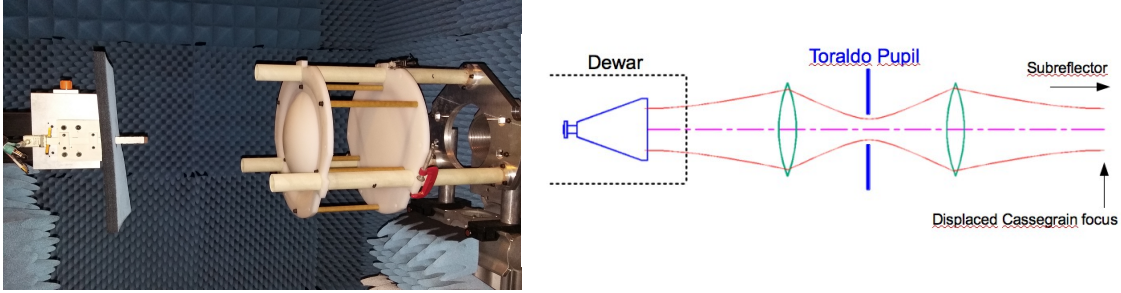
Fig. 3 Left panel. Laboratory setup showing the two-lens collimator, illuminated by a K-band corrugated feed horn. The focus fields are sampled with an open waveguide. Right panel. Gaussian-beam propagation in the collimator.
