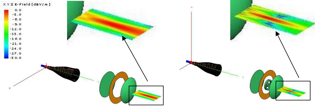
Fig. 1 FEKO simulations at 20 GHz showing the (normalized) field amplitude at the focus of the collimator without ( left panel ) and with ( right panel ) TP. The collimator is illuminated by the same corrugated feed horn of the K-band receiver at Medicina.
