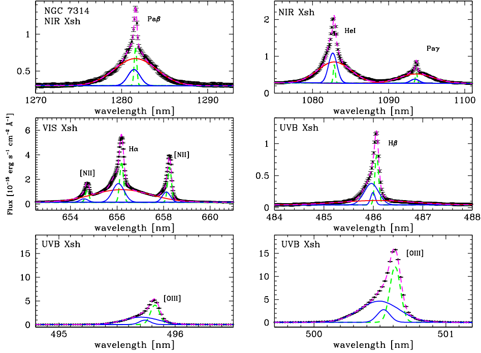
Figure 19. Near infrared and optical spectra of NGC 7314, corrected for redshift. Top-left: Pa \beta +[Fe II] region. Top-right: He I+Pa \gamma region. Center-left: H \alpha + [N II] region. Center-right: H \beta + [O III] region. Bottom-left: [O III] \lambda 4959 region. Bottom-right: [O III] \lambda 5007 region. The narrow, intermediate and broad components are shown with green-dashed, blue and red lines, respectively. The magenta-dashed line shows the total fitting model.
