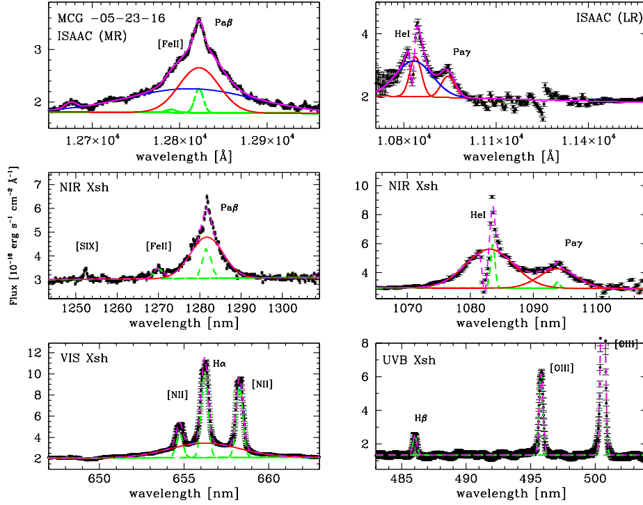
Figure 11. Near infrared and optical spectra of MCG-05-23-016, corrected for redshift. Top-left: ISAAC MR Pa \beta +[Fe II] region. Top-right: ISAAC LR He I+Pa \gamma region. Center-left: X-shooter Pa \beta +[Fe II] region. Center-right: X-shooter He I+Pa \gamma region. Bottom-left: X-shooter H \alpha +[N II] region. Bottom-right: X-shooter H \beta +[O III] region. The narrow, intermediate and broad components are shown with green-dashed, blue and red lines, respectively. The magenta-dashed line shows the total fitting model.
