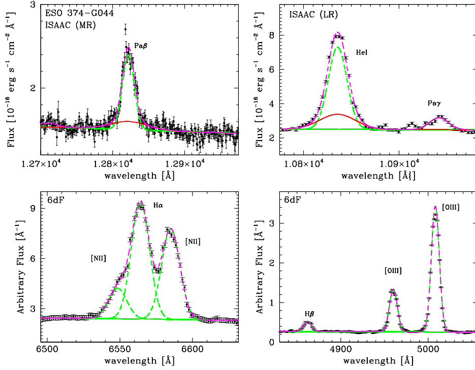
Figure 9. Near infrared and optical spectra of ESO 374–G044, corrected for redshift. Top-left: Pa \beta +[Fe II] region. Top-right: He I+Pa \gamma region. Bottom-left: H \alpha + [N II] region. Bottom-right: H \beta + [O III] region. The narrow, intermediate and broad components are shown with green-dashed, blue and red lines, respectively. The magenta-dashed line shows the total fitting model.
