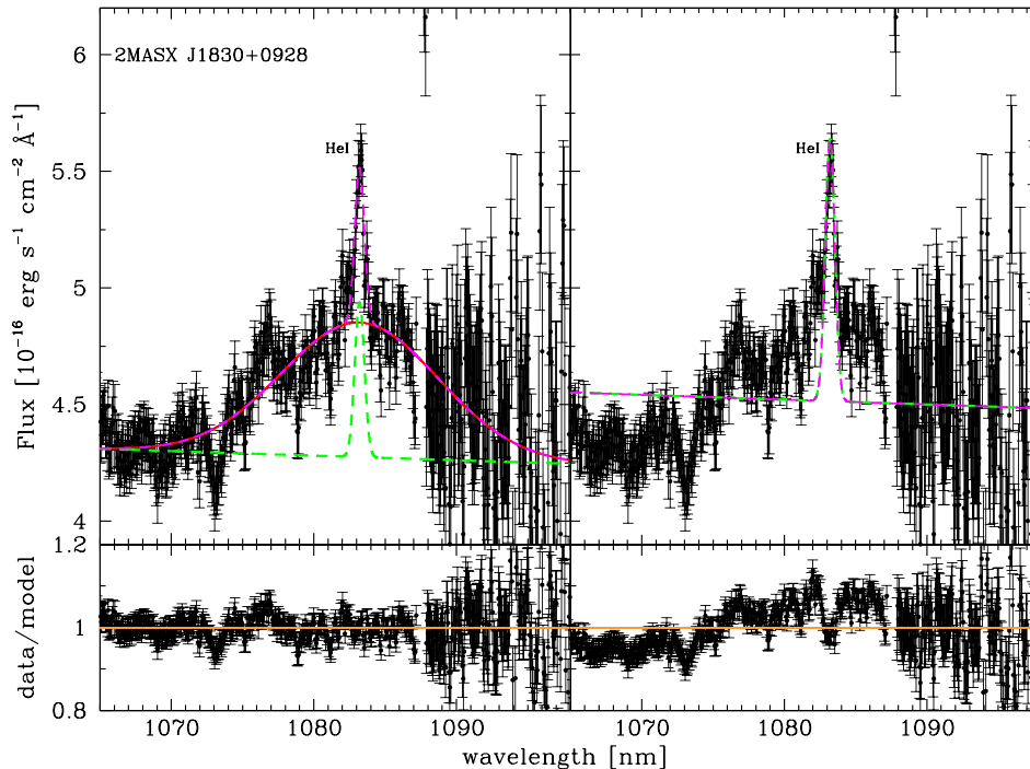
Figure A6. Left: best fit of the He I line of 2MASX J18305065+0928414 including a broad ( \text{FWHM} = 3513 \text{ km s}^{-1} ) He I component. Right: same as before without including a broad He I component. Lower panels show the data to model ratio.
