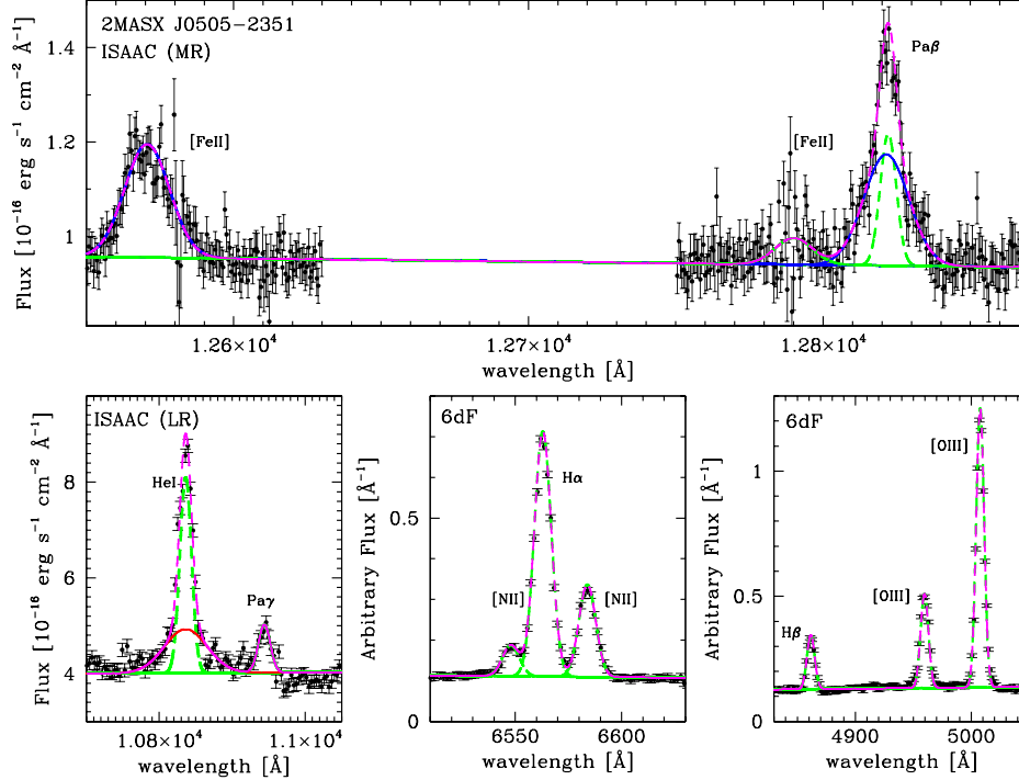
Figure 8. Near infrared and optical spectra of 2MASX J05054575-2351139, corrected for redshift. Top: Pa \beta +[Fe II] region. Bottom-left: He I+Pa \gamma region. Bottom-middle: H \alpha +[N II] region. Bottom-right: H \beta +[O III] region. The narrow, intermediate and broad components are shown with green-dashed, blue and red lines, respectively. The magenta-dashed line shows the total fitting model.
