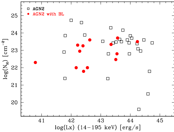
Figure 27. Hydrogen column density, N_H , as a function of the 14–195 keV luminosity of the ‘non-broad’ (black open squares) and the ‘broad’ (red filled circles) AGN2 samples.
