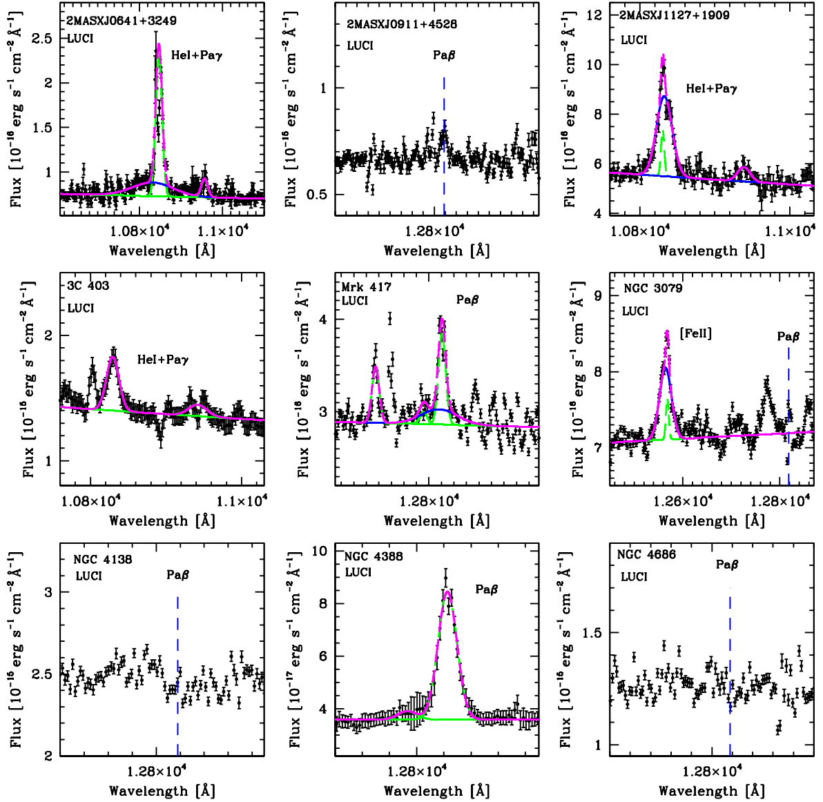
Figure B1. Lines fit of LUCI 'non-broad' AGN2.
