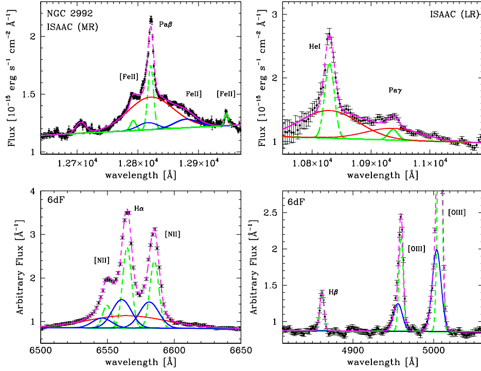
Figure 15. Near infrared and optical spectra of NGC 2992, corrected for redshift. Top-left: Pa \beta +[Fe II] region. Top-right: He I+Pa \gamma region. Bottom-left: H \alpha + [N II] region. Bottom-right: H \beta + [O III] region. The narrow, intermediate and broad components are shown with green-dashed, blue and red lines, respectively. The magenta-dashed line shows the total fitting model.
