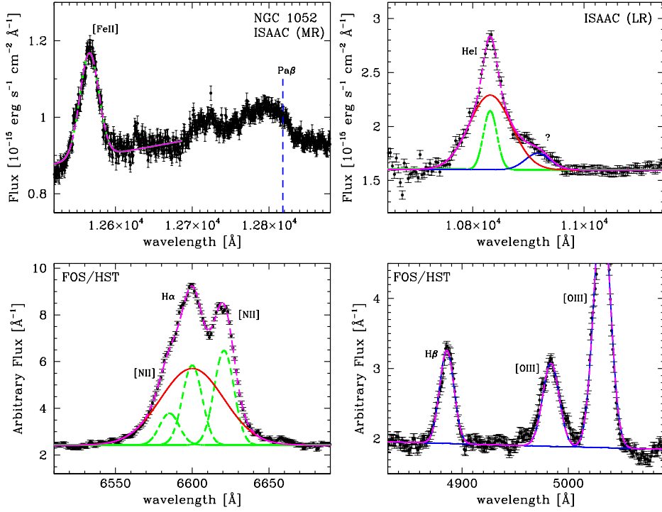
Figure 13. Near infrared and optical spectra of NGC 1052, corrected for redshift. Top-left: Pa \beta +[Fe II] region. Top-right: He I+Pa \gamma region. Bottom-left: H \alpha + [N II] region. Bottom-right: H \beta + [O III] region. The narrow, intermediate and broad components are shown with green-dashed, blue and red lines, respectively. The magenta-dashed line shows the total fitting model. The blue-dashed vertical line indicate the Pa \beta position.
