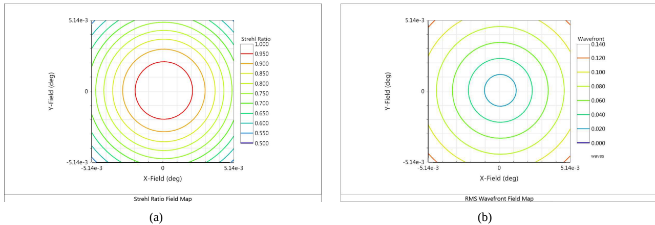
Figure 7. Telescope Strehl ratio (a) and telescope RMS WFE (b) calculated over a 37 arcsec square field of view for a wavelength of 3.9\text{ }\mu\text{m} .
