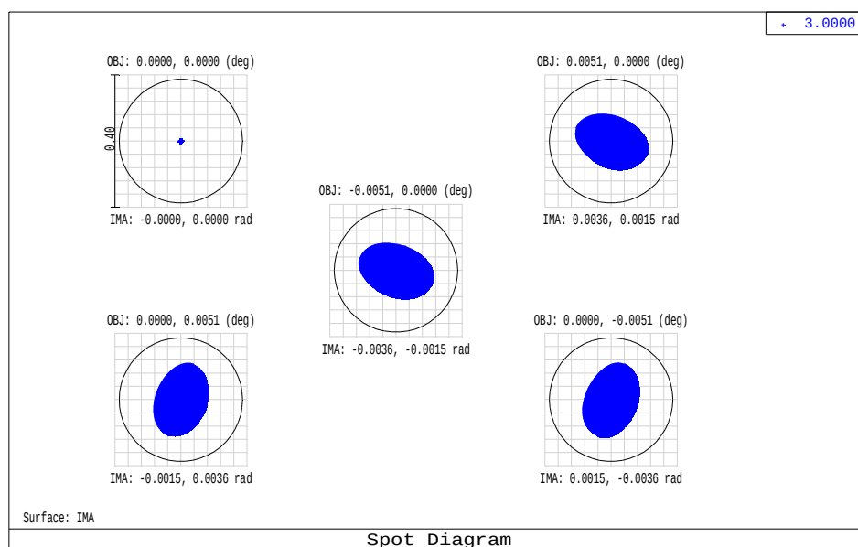
Figure 6. Spot diagrams for the telescope in afocal image space (units are mrad). The spot diagrams are compared with the Airy disk calculated at the nominal telescope diffraction limited wavelength of 3 \mu\text{m} .
