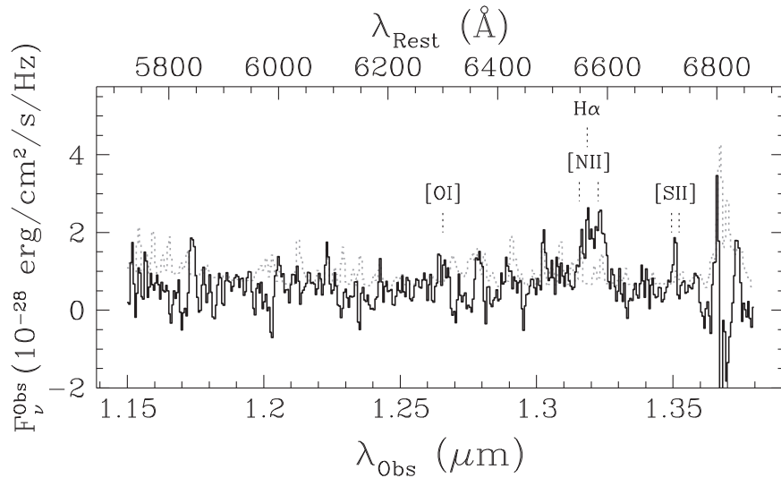
Figure 3. Near-IR Keck/NIRSPEC spectrum of WISE J1036+0449 (see Section 2.1.2 for details). The dashed line shows the error spectrum.
