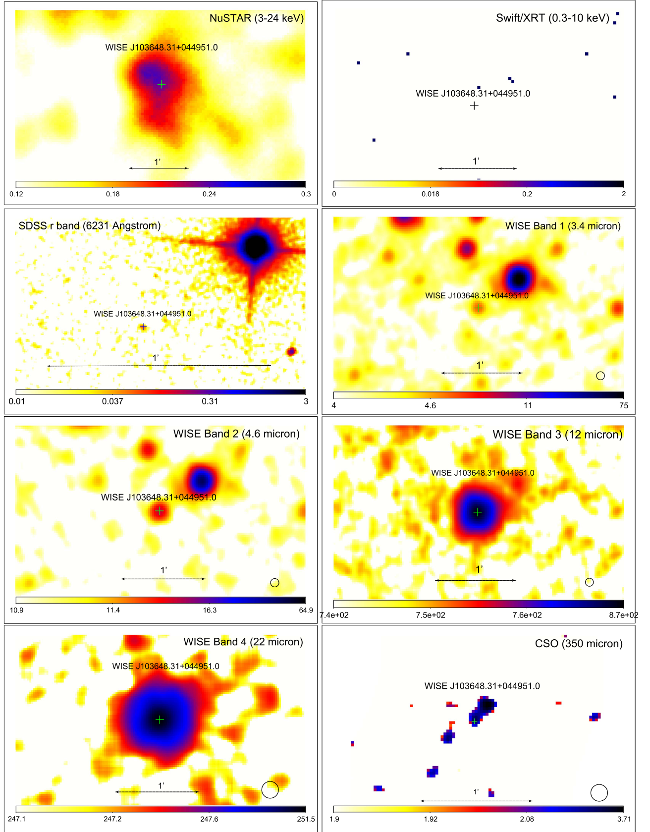
Figure 1. Images of the field around WISE J1036+0449 from the hard X-rays to the far-IR. From top to bottom, the panels show the images obtained by NuSTAR FPMA (3–24 keV); Swift /XRT (0.3–10 keV); the SDSS r -band (6231 Å); WISE band 1 (3.4 μm), band 2 (4.6 μm), band 3 (12 μm), and band 4 (22 μm); and CSO (350 μm). The NuSTAR image was obtained by combining three observations, as described in Section 4, and was smoothed with a Gaussian kernel of a radius of 12 pixels. The SDSS image was smoothed with a Gaussian kernel of a radius of 2 pixels. The CSO image shows the signal-to-noise ratio per pixel. The crosses show the position of WISE J1036+0449, while the circles on the bottom right show the size of the beam. In all images, north is up and east is left.
