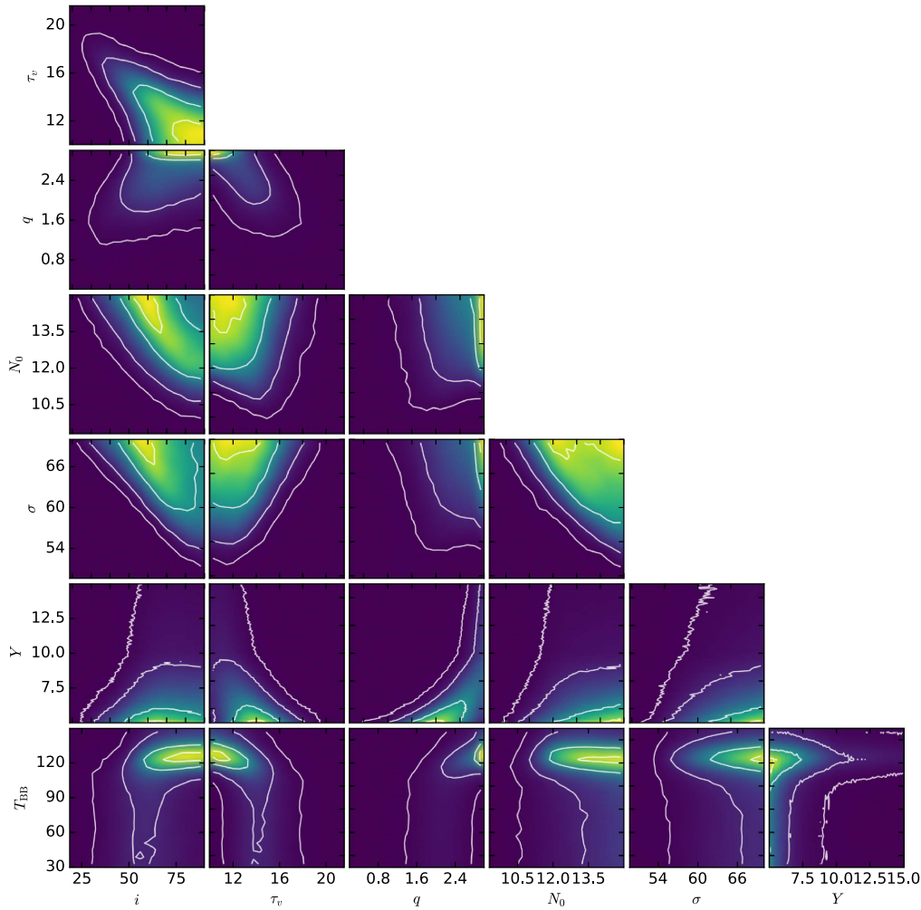
Figure 9. Confidence plot for the SED fit carried out using the complete data set. The white contours are at 1%, 10%, 50%, and 90% of the peak pixel in each panel.
