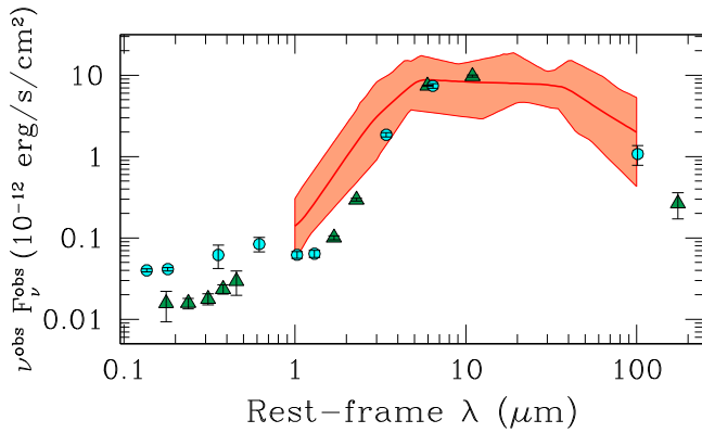
Figure 4. Rest-frame UV through far-IR broadband SED of WISE J1036+0449 (green triangles). The green triangles show the flux measured in the SDSS u'r'g'i'z' bands, the four WISE photometric bands, and the CSO/SHARC II 350 \mu\text{m} band. The red solid line shows the geometric mean SED of the sources studied by Tsai et al. (2015) using WISE and Herschel Space Observatory observations, scaled to the WISE photometry of WISE J1036+0449. The cyan circles show the SED of WISE J1814+3412 (renormalized to a similar flux level of WISE J1036+0449 for comparison), while the light red region shows the range covered by all the sources in the study of Tsai et al. (2015). The SED is shown in \nu F_\nu for comparison with that of Tsai et al. (2015).
