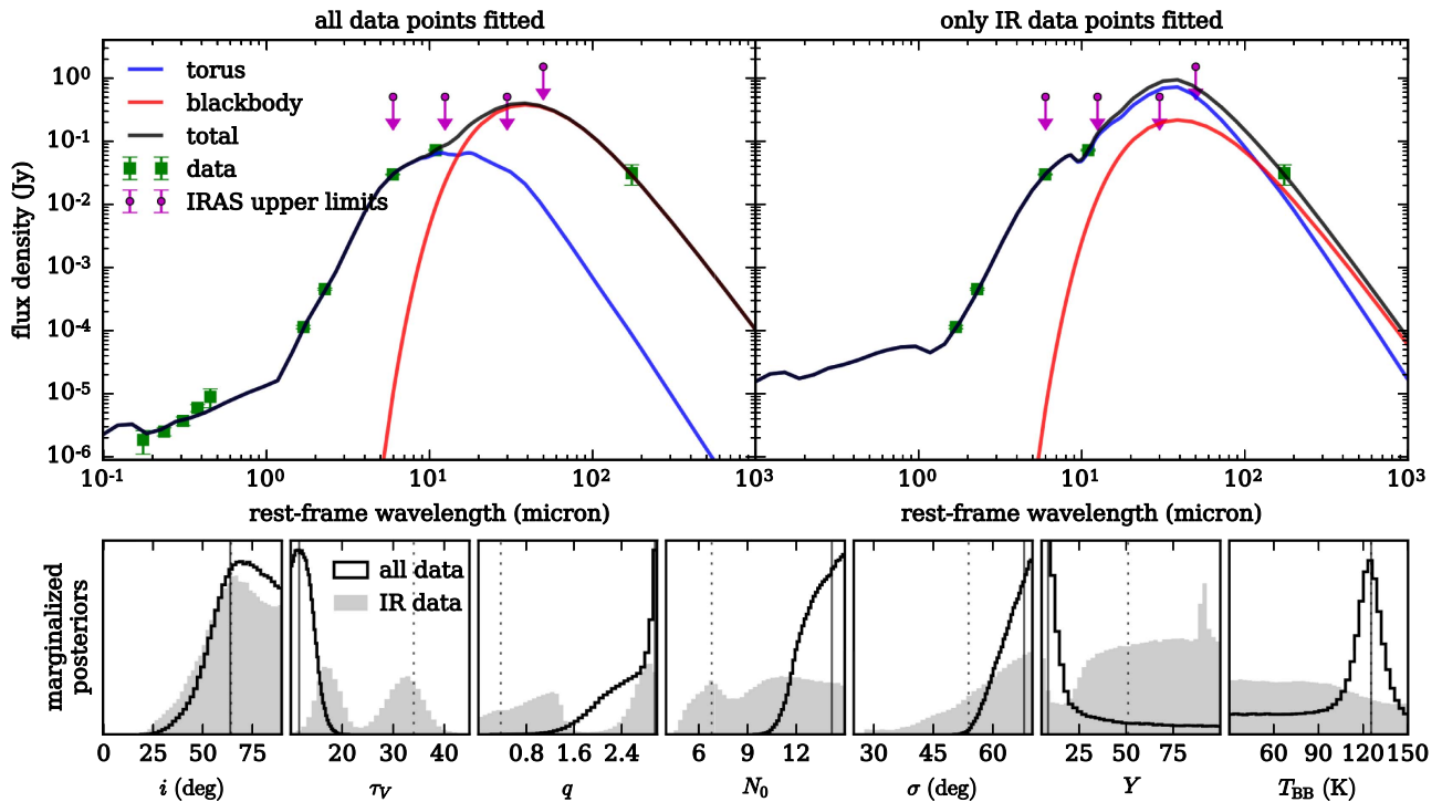
Figure 5. SED fitting and Bayesian inference of model parameters. Upper left: maximum a posteriori (MAP) composite model (in black), comprised of an AGN torus component (blue) and a modified BB (red), fitted to all available data of WISE J1036+0449 (green squares with error bars). The purple circles show the IRAS upper limits (Neugebauer et al. 1984). Upper right: same, but fitted to IR data only. Lower panels: marginalized posterior of all model parameters for the all-data model (black histogram) and the IR-only model (gray histogram). The solid and dotted vertical lines indicate the MAP values of each parameter for the two respective models. The SED is in F_\nu for consistency with the fitting procedure of Nikutta (2012). A detailed description of the different parameters and of the results obtained by the SED fitting is presented in Appendices A and C.
