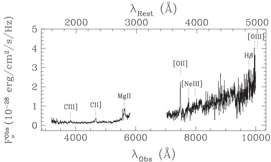
Figure 2. UV/optical spectrum of WISE J1036+0449, obtained with the LRIS instrument at the Keck Observatory. See Section 2.1.1 for details.
