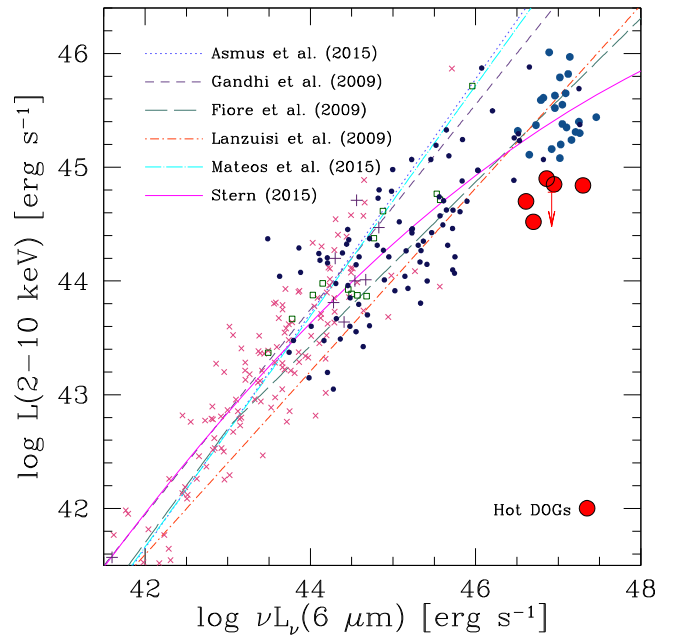
Figure 8. Rest-frame 6 \mu\text{m} luminosity vs. intrinsic rest-frame 2–10 keV luminosity for several samples of AGNs: Hot DOGs from this work (big red circles; the red arrow represents the upper limit for WISE J2207+1939), broad-lined AGNs from the SEXSI survey (Eckart et al. 2010; open green squares), luminous quasars from Just et al. (2007; large solid blue circles), Compton-thin AGNs observed by NuSTAR (Alexander et al. 2013; Del Moro et al. 2014; purple crosses), quasars from SDSS DR5 (Young et al. 2009; small blue dots), and local Seyfert galaxies (Gandhi et al. 2009; Asmus et al. 2015; red crosses). The lines illustrate five L_{6\mu\text{m}}-L_{2-10 \text{ keV}} relations (see Section 5.2 for details). The mid-IR luminosities of Asmus et al. (2015) were obtained at 12 \mu\text{m} . The figure shows that hot DOGs are significantly weaker in the X-ray band than unobscured quasars in the same 6 \mu\text{m} luminosity range.
