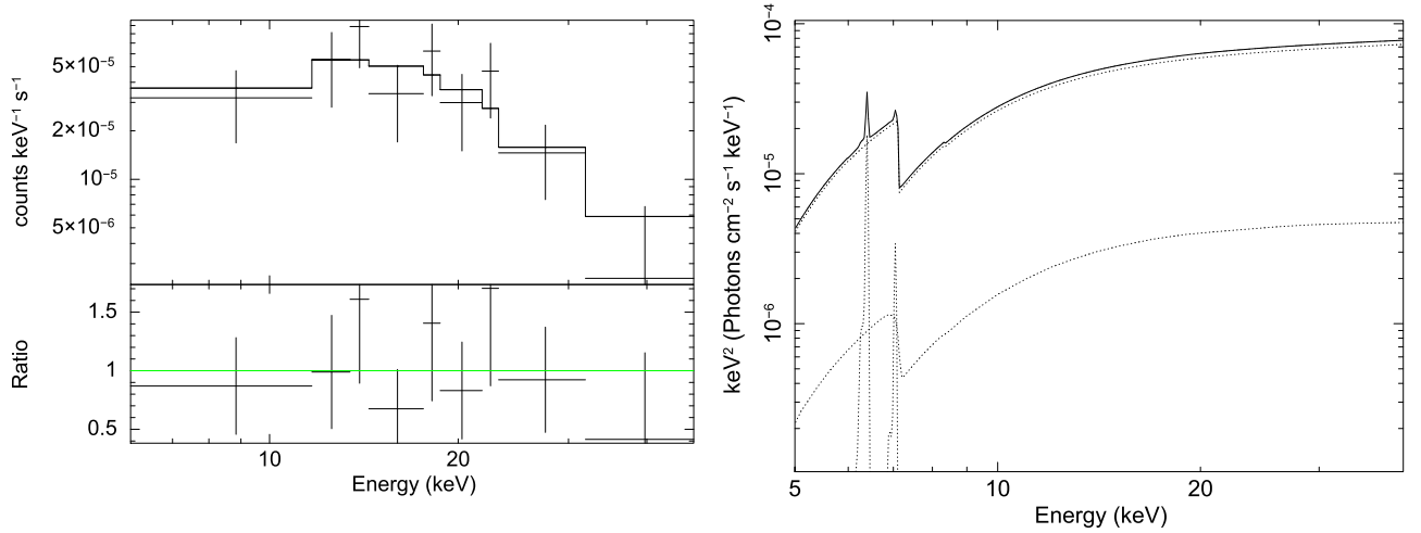
Figure 6. Left panel: combined NuSTAR FPMA and FPMB spectrum of WISE J1036+0449 fitted with the MYTORUS model (assuming \Gamma = 1.9 ; see Section 4). The bottom panel shows the ratio between the data and the model. Right panel: spectrum of the MYTORUS model with the parameters fixed to those obtained by fitting the combined NuSTAR FPMA and FPMB spectrum. The dotted lines represent the primary X-ray emission (upper part of the figure), the scattered component (lower part), and the fluorescent lines. In both plots, the energies are in the rest frame of the source.
