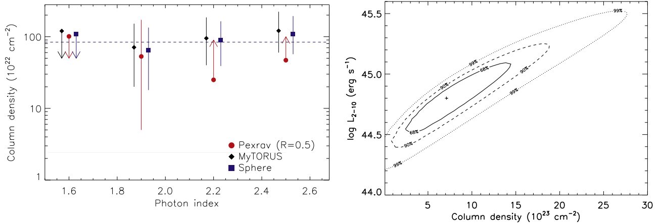
Figure 7. Left panel: values of the column density N_H obtained by assuming different values of the photon index of the primary X-ray radiation for the PEXRAV, MYTORUS, and SPHERE models. The points obtained with the last two models have been shifted by \Delta\Gamma = \mp 0.03 for visual clarity. The dashed line shows the value of N_H obtained from E(B - V) by using Equation (1) (see also Table 3). Right panel: confidence intervals of the intrinsic 2–10 keV luminosity and the column density for WISE J1036+0449 obtained using the MYTORUS model. The continuous, dashed, and dotted lines represent the 68%, 90%, and 99% confidence contours, respectively. The black cross represents the best-fit value of the parameters.
