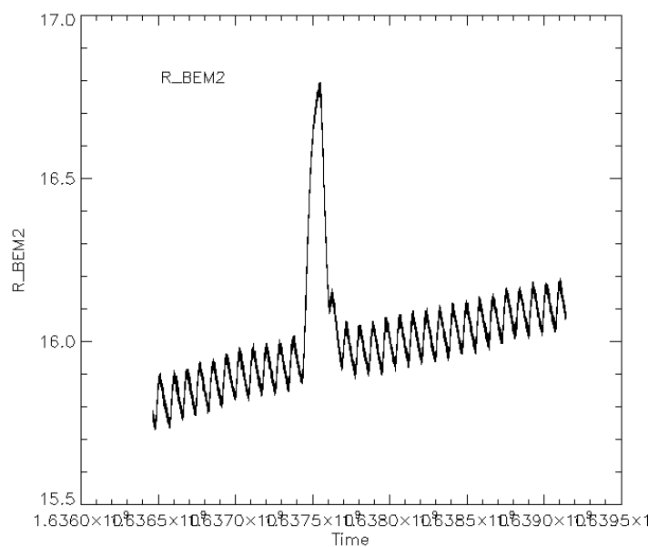
Figure 9 BEU temperature from OD 180 to OD 210: the abrupt increase is due to the transponder heating effect.
